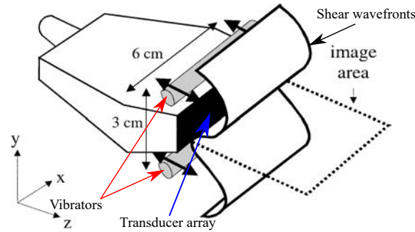
Figure 1.4: 2D transient elastography: Shear waves are generated using a vibrator composed of two parallel rods. The linear array of transducers is placed between the rods. The shear wave front has a cylindrical shape in the out-of plane direction. Source: [SAN 02a]
