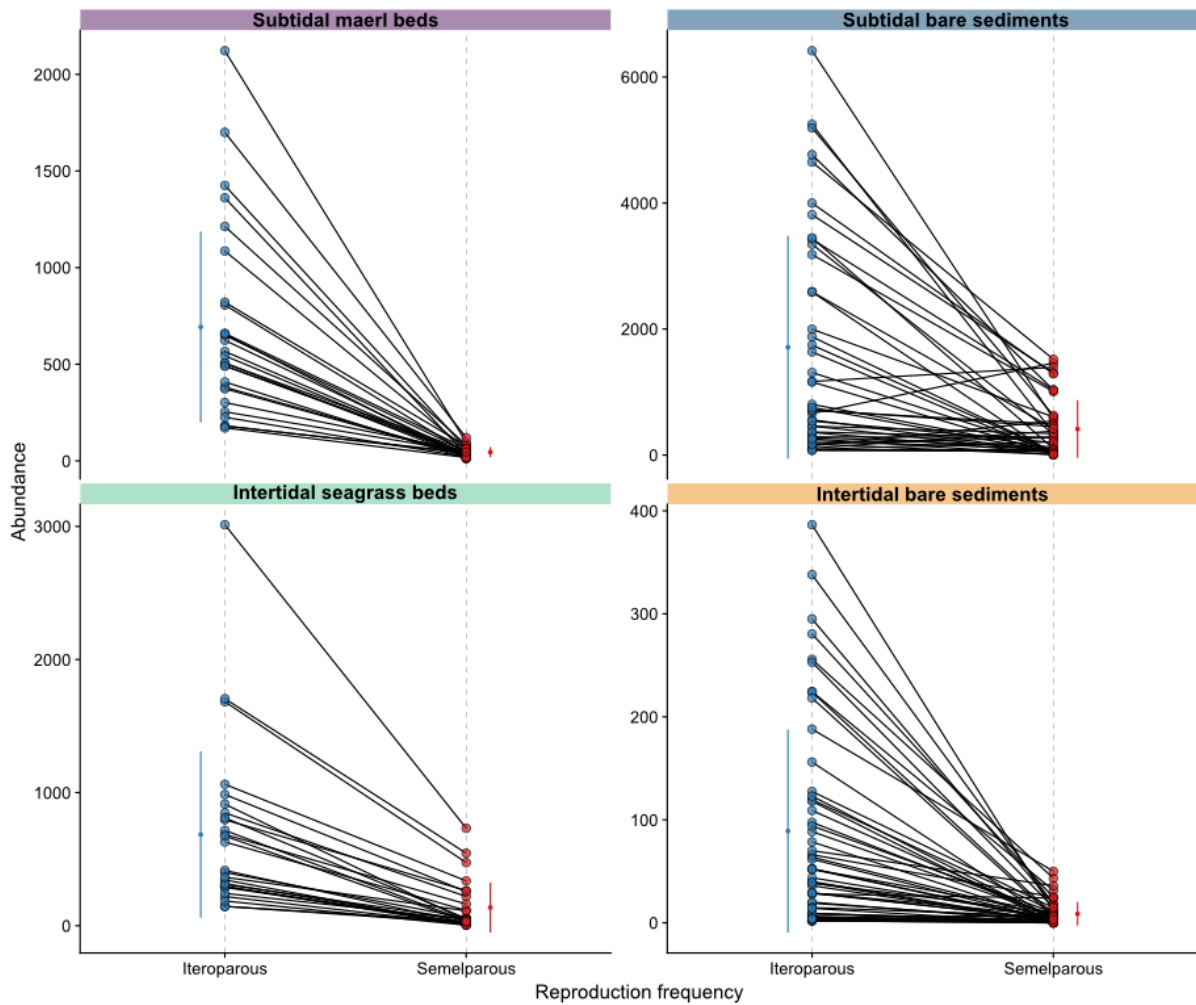
Figure 4. Abundances of the two modalities of reproduction frequency for the different assemblages of each habitat. The lines link the abundance of one modality to the abundance of the other for each assemblage. The mean and standard deviation of each modality for each habitat are plotted next to the points. For subtidal maerl assemblages, reproduction frequency consistently converge towards iteroparous species while the distribution of abundances among the two modalities is more variable and in general follow a random pattern in the other habitats (see Figure 3 of the Supplementary material)
