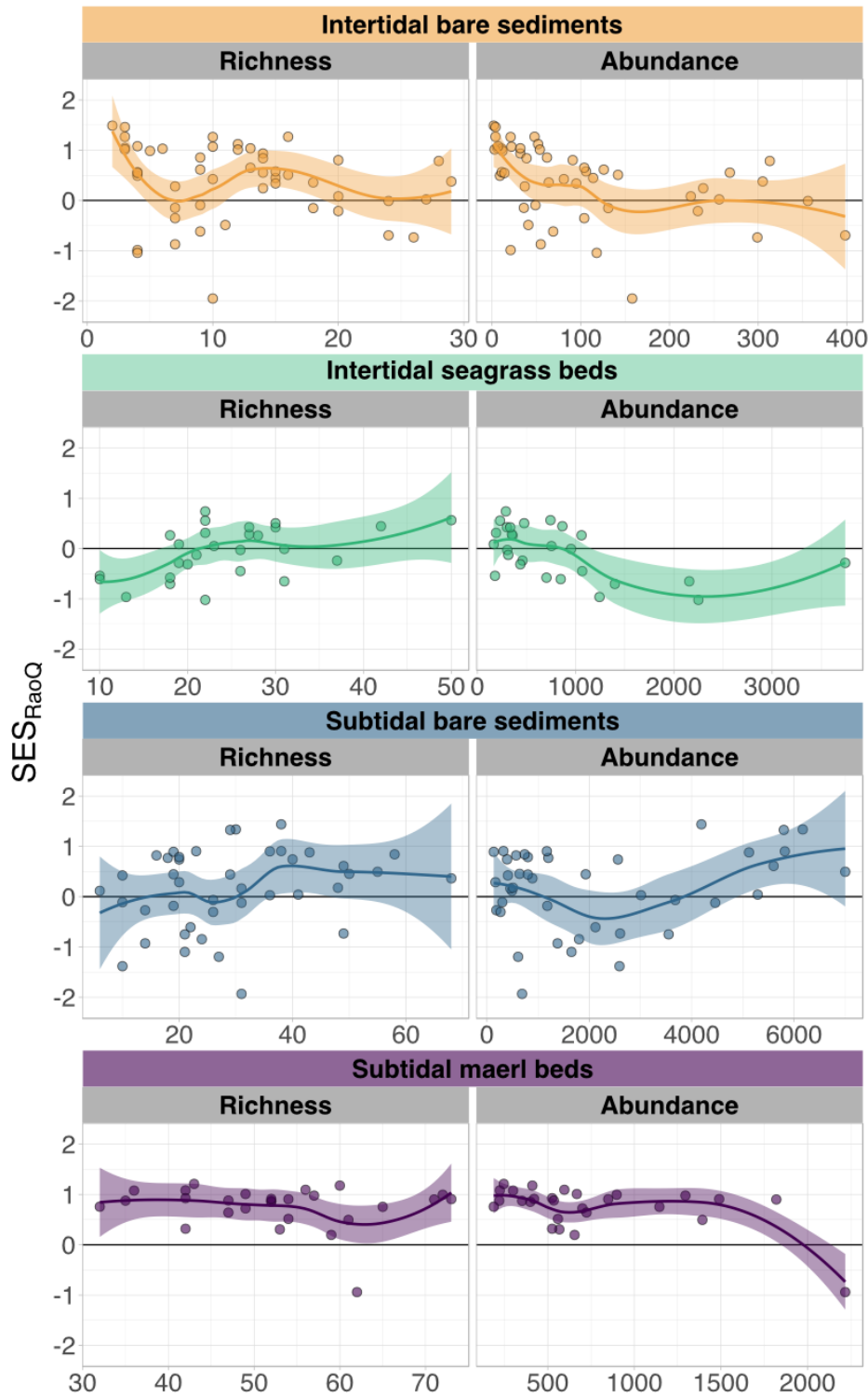
Figure 2. Relationships between the SES_{RaoQ} and the richness or total abundance of the assemblages for the four habitats
