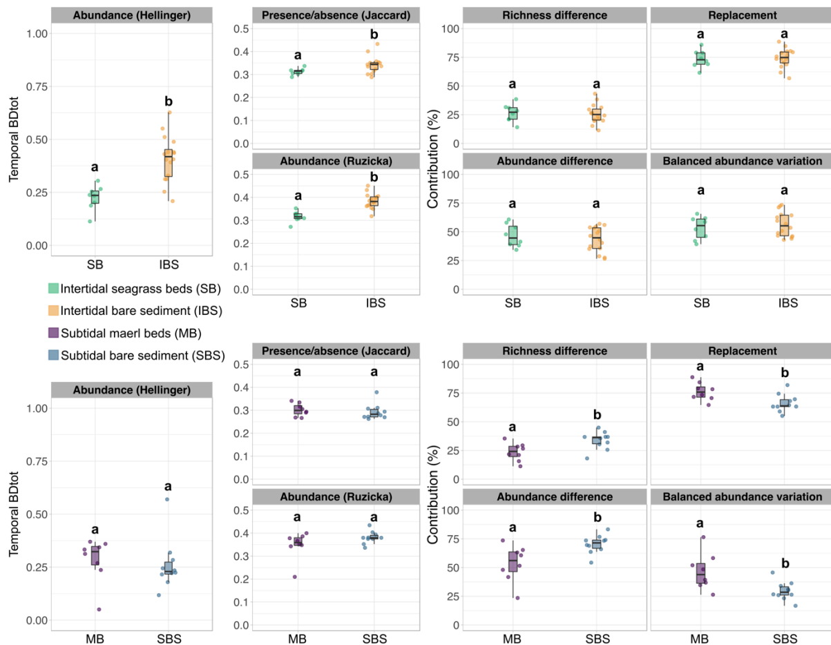
Figure 4. Temporal variability of the assemblages according to the habitats. The overall temporal \beta diversity of each site (Temporal BDtot) was measured on species density data using Hellinger distances as well as the Ružička difference index and on presence/absence data using Jaccard dissimilarity. When all years contain a different set of species with no species in common, the maximum value that BDtot can take is 0.5 for the Jaccard dissimilarity and for its quantitative form, the Ružička difference index. This maximum value is 1 for the Hellinger distance. The overall contributions of species replacement (vs richness differences) and balanced abundance variation (vs total abundance differences) to the total temporal \beta diversity of the assemblages were assessed by partitioning the Jaccard dissimilarity and the Ružička difference index respectively. This was done using Podani-family decompositions as described in Legendre (2014). Contributions are represented as percentages of BDtot. Within each habitat, points were jittered along the x-axis to see them individually. Differences between biogenic and bare habitats were assessed within each tidal level using Mann-Whitney-Wilcoxon tests. Within each panel, significant differences at the \alpha = 0.05 threshold are represented by different letters.
