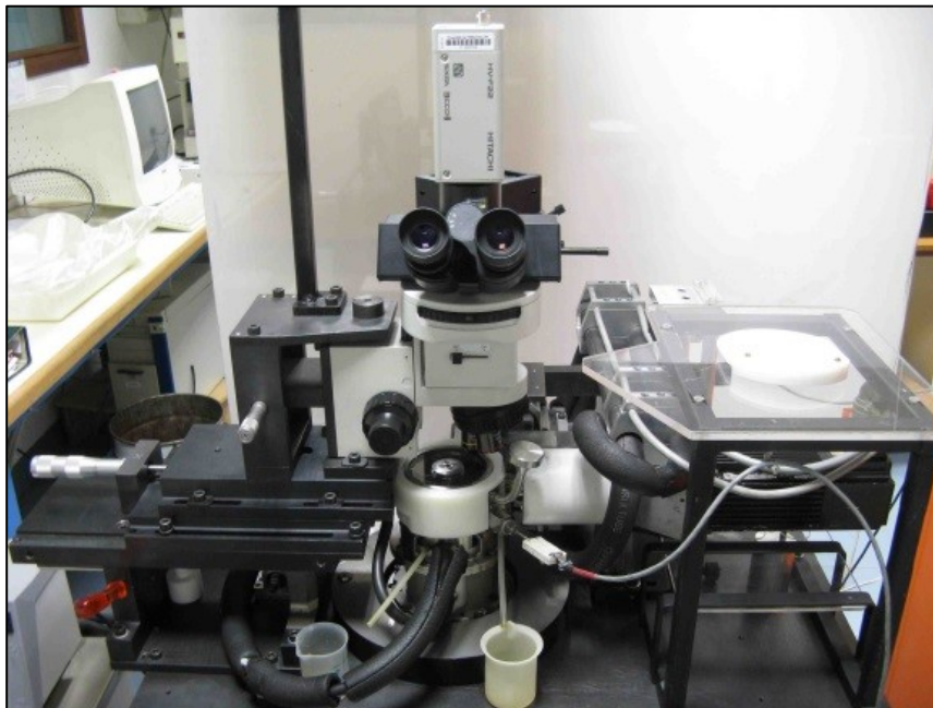
Figure 2.4. Jerotrib test rig.
