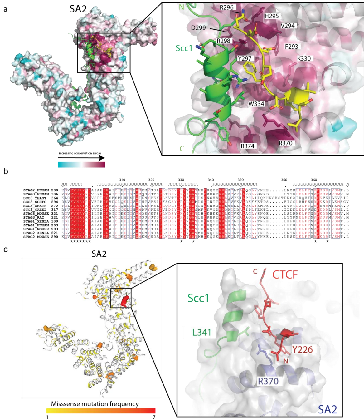
Figure 5.8 Analysis of the SA2-Scc1-CTCF structure. (a) Surface representation of the complex with SA2 surface rendered and colored according to sequence conservation. The inset shows a detailed view of conserved SA2 residues around the CTCF binding site. (b) Multiple sequence alignment of SA2 (STAG2) orthologs and paralogs. The key amino acid residues engaging CTCF are indicated by (*). (c) Missense mutation frequencies have been plotted onto the SA2 structure. The inset shows mutation hotspots R370 (SA2), Y226 and F228 (CTCF) and S334, L338 and L341 (Scc1).
