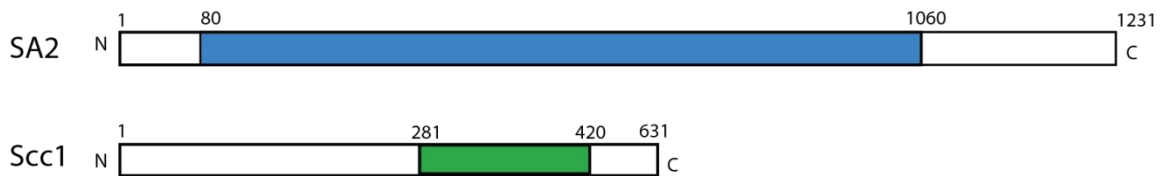
Figure 1.3 Structure of the human SA2-Scc1 complex and domain boundaries.
