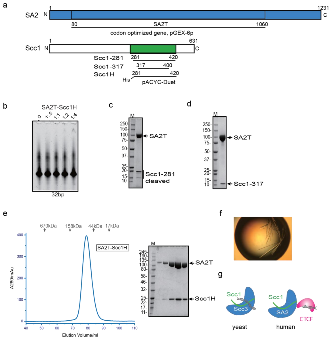
Figure 5.2 SA2-Scc1 constructs, purification and EMSA analysis. (a) Cartoon of human SA2-Scc1 constructs used for crystallization and interaction studies. (b) EMSA analysis of hSA2-Scc1 complex with a 32 bp dsDNA substrate (Table 4.1), showed no DNA binding for hSA2-Scc1. (c-d) SDS-PAGE analysis of hSA2 with different truncations of Scc1. The Scc1 construct (281-420) is partially degraded after expression/purification from E.coli . Construct (317-400), contains a truncation of the disordered regions. (e) Purification of SA2T-Scc1H complex used for crystallization and interaction analysis. (f) Crystal image of the SA2T-Scc1H complex used for peptide soaking. (g) Proposed model on how yeast and human Scc3 associate with DNA. In yeast, Scc3 binds with DNA
