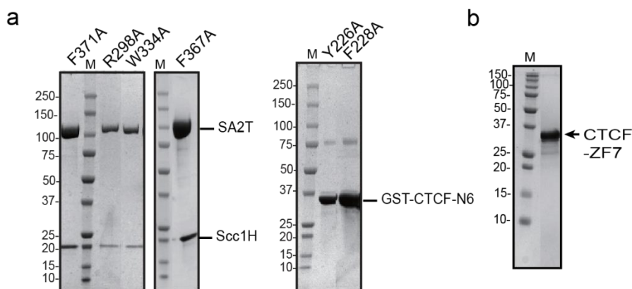
Figure 5.4 Purification of SA2-ScclH mutants, CTCF-N6 mutants and CTCF covering both SA2-Sccl1 binding region and zinc finger 1-7 (CTCF-ZF7), used for pull-down and EMSA.
