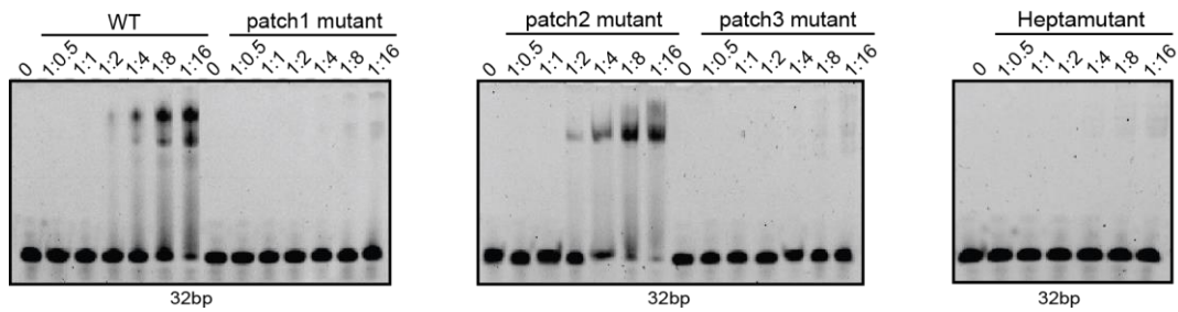
Figure 4.7 DNA binding affinity test of both Scc3T-Scc1K wild type and mutants via EMSA. The binding affinity difference is consistent with the fluorescence polarization experiment (Figure 4.8c).
