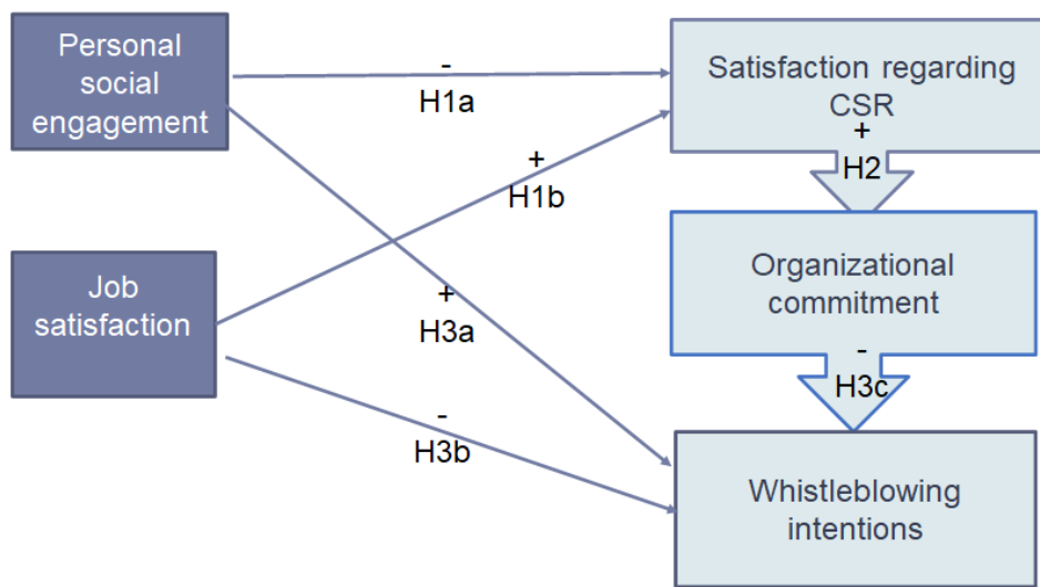
Figure 3: Theoretical model
