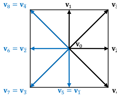
Figure 9: 2D Lattice Boltzmann model with 9 nodes: d_2Q_9
