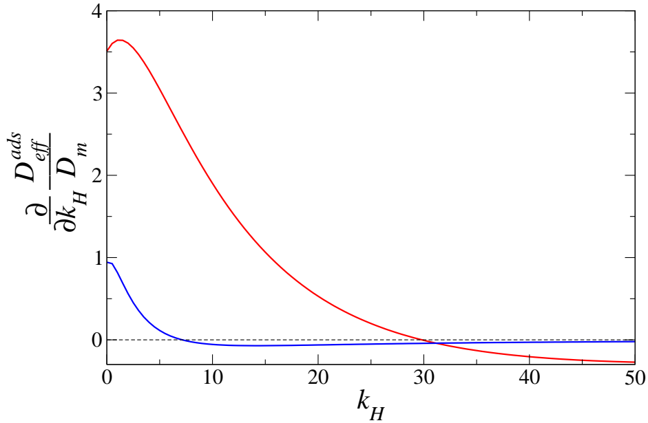
Figure 43: Effect of the adsorption/desorption ratio k_H on the dispersion coefficient D_{eff}^{ads}/D_m (note that to highlight this effect, we plot the derivative of the dispersion coefficient with respect to k_H ). The systems considered here correspond to the slit pore geometry with different characteristic lengths L_y (defined as the width between the two parallel plates). The data are for systems with a mean velocity U and a molecular diffusion coefficient D_m . The red and blue colors denote data obtained for L_y = 41\Delta x and L_y = 10\Delta x , respectively.
