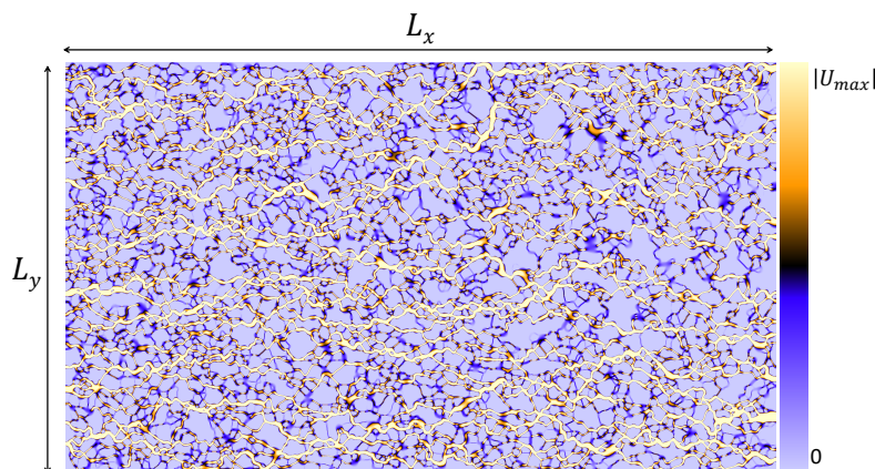
Figure 54: Velocity field obtained by solving Stokes equation using LBM-TRT in the micro-model ( L_x = 4000 and L_y = 2300 ).
