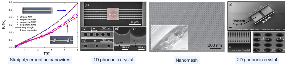
Figure 1.5: Some examples of material nanostructuring intended to reduce the lattice contribution to the thermal conductivity, for 1D and 2D systems. Images are reprinted with permission from Refs. 48–51. Importantly, the constrictions/holes are designed in such a way that their size match the material’s phonon mean free path or wavelength. For this reason, the efficiency of thermal conductivity reduction strongly depends on temperature.
