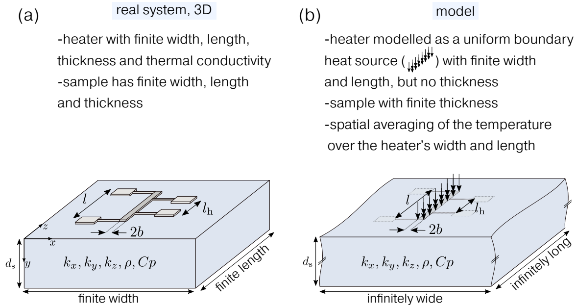
Figure 4.7: (a) System of interest sketched in 3D and (b) the model used to approximate it and calculate the temperature oscillation across the inner leads of the thermometer. As in the 2D model, the heat flux is approximated as a boundary condition, but this time the surface boundary condition is extended in the z direction as well. The thermal conductivity of the system can be anisotropic in all three directions of the cartesian coordinate system (x, y, z) .
