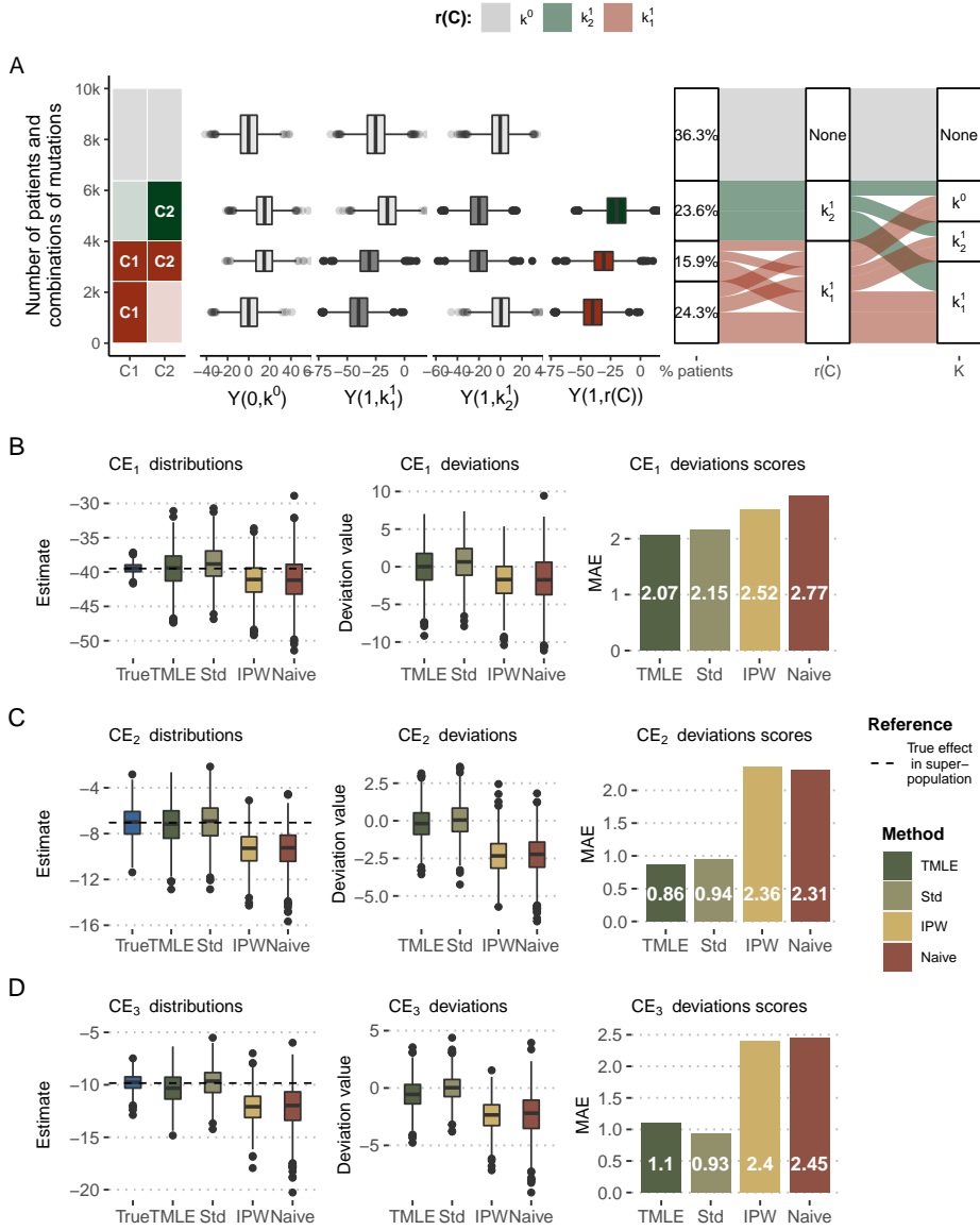
Figure 9.7: Causal effects of precision medicine strategy with simulated data. (A) Main variables and relations in the simulated super-population. From left to right: categories of patient based on their mutations; responses to k^0 , k_1^1 , k_2^1 and precision medicine K = r(C) ; repartition of patients regarding their precision medicine drug and their assigned treatment in observed data. (B) Distribution and deviation of CE 1 estimates based on different methods, deviation scores being computed based on mean absolute error (MAE). (C) Same for CE 2 . (D) Same for CE 3 .
