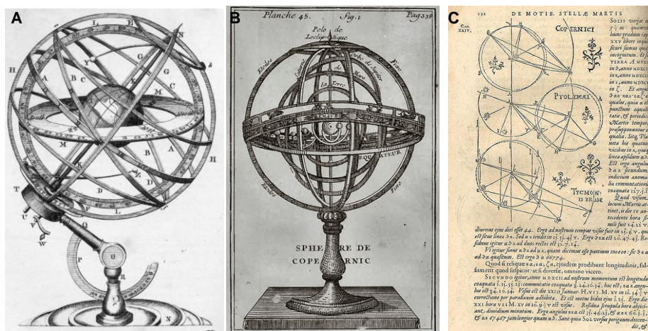
Figure 1.4: Orrery, planets and models. Physical models of planetary motion, either geocentric (Armillary sphere from Plate LXXVII in Encyclopedia Britannica , 1771) or heliocentric in panel B (Bion, 1751, catalogue Bnf ) and some geometric representations by Johannes Kepler in panel C (in Astronomia Nova , 1609)
