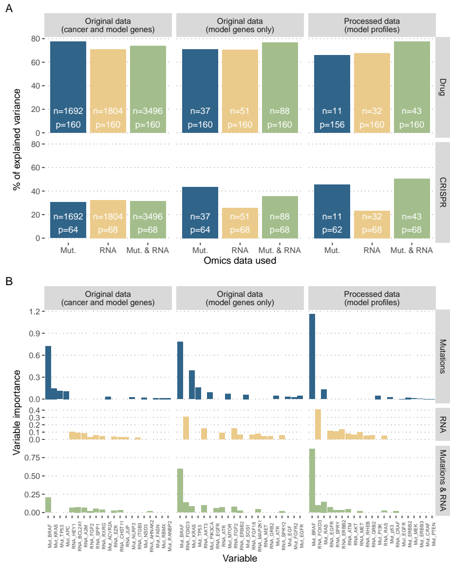
Figure 6.9: Random forests to predict and explain sensitivity to BRAF inhibition. (A) Performances of random forests for BRAF sensitivity prediction measured with percentage of explained variance; different learning task with unprocessed original data (thousands of genes), unprocessed original data for model-related genes only (tens of genes), and processed profiles of cell lines (tens of genes); n samples and p variables per learning task. (B) Variable importance for drug prediction only, with the 10 best variables with positive importance for each case.
