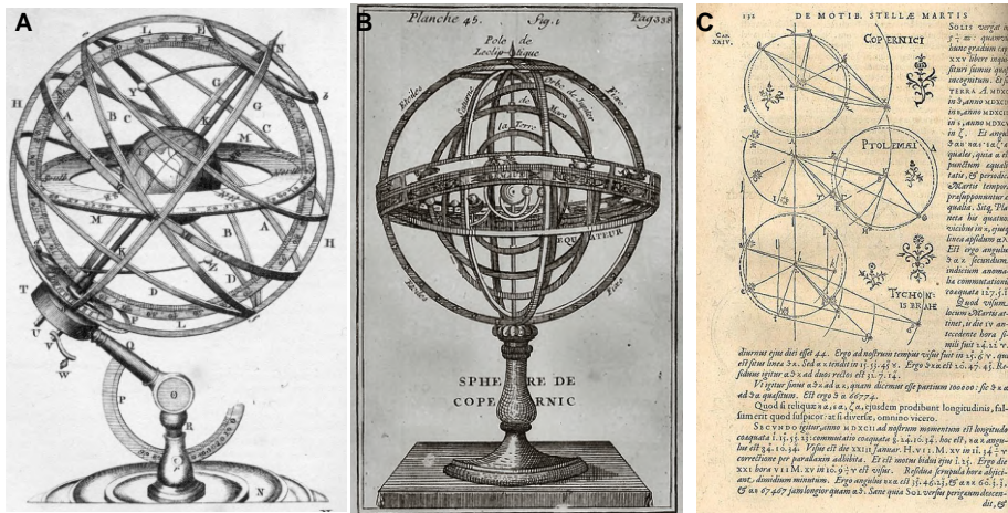
Figure 1.4: Orrery, planets and models. Physical models of planetary motion, either geocentric (Armillary sphere from Plate LXXVII in Encyclopedia Britannica , 1771) or heliocentric in panel B (Bion, 1751, catalogue Bnf ) and some geometric representations by Johannes Kepler in panel C (in Astronomia Nova , 1609)
