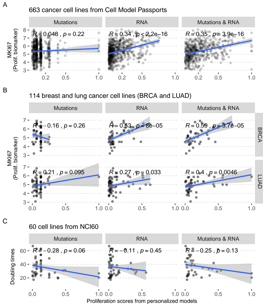
Figure 5.6: Validation of personalized Proliferation scores in cell lines. (A) Comparison with MKI67 proliferation biomarker for all cancer cell lines. (B) Same with breast (BRCA) and lung (LUAD) cancer only. (C) Comparison with doubling times in a subset of 60 cell lines.
