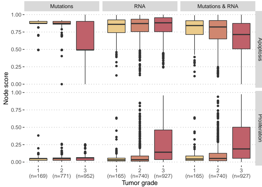
Figure 5.7: Comparison of personalized scores with tumor grades for breast cancer patients in METABRIC cohort. Comparisons are provided for different personalization strategies (with mutations and/or RNA) and two different model nodes ( Proliferation and Apoptosis ).
