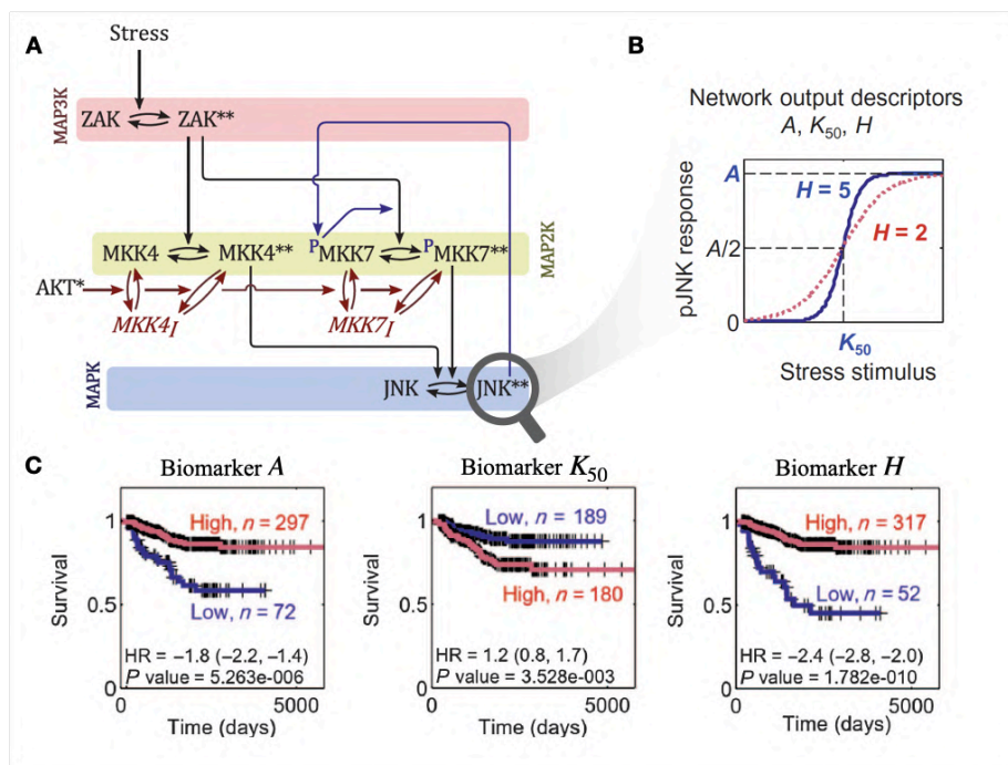
Figure 3.6: Mechanistic modeling of JNK pathway and survival of neuroblastoma patients , as described by Fey et al. [2015]. (A) Schematic representation, as a process description, for the ODE model of JNK pathway. (B) Response curve (phosphorylated JNK) as a function of the input stimulus (Stress) and characterization of the corresponding sigmoidal function with maximal amplitude A , Hill exponent H and activation threshold K_{50} . (C) Survival curves for neuroblastoma patients based on binarized A , K_{50} and H ; binarization thresholds having been defined based on optimization screening on calibration cohort.
