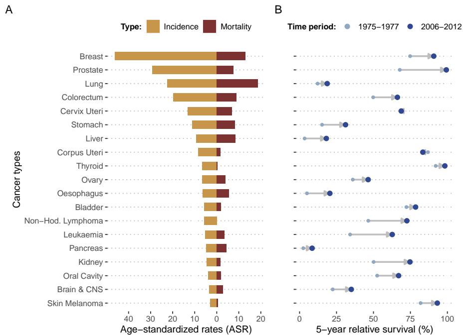
Figure 2.3: Incidence, mortality and survival per cancer types. (A) World incidence and mortality for the 19 most frequent cancer types in 2018, expressed with age-standardized rates (adjusted age structure based on world population); data retrieved from Global Cancer Observatory . (B) Evolution of 5-years relative survival for the same cancer types based on US data from SEER registries in 1975-1977 and 2006-2012; data retrieved from Jemal et al. [2017].
