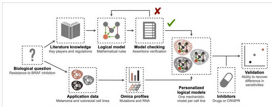
Figure 6.3: BRAF modeling flowchart: from a biological question to validated personalized logical models. Logical models are written with MaBoSS, and the checking model procedure is therefore provided in the same formalism. Cell line data are taken from Cell Model Passports [van der Meer et al., 2019].
