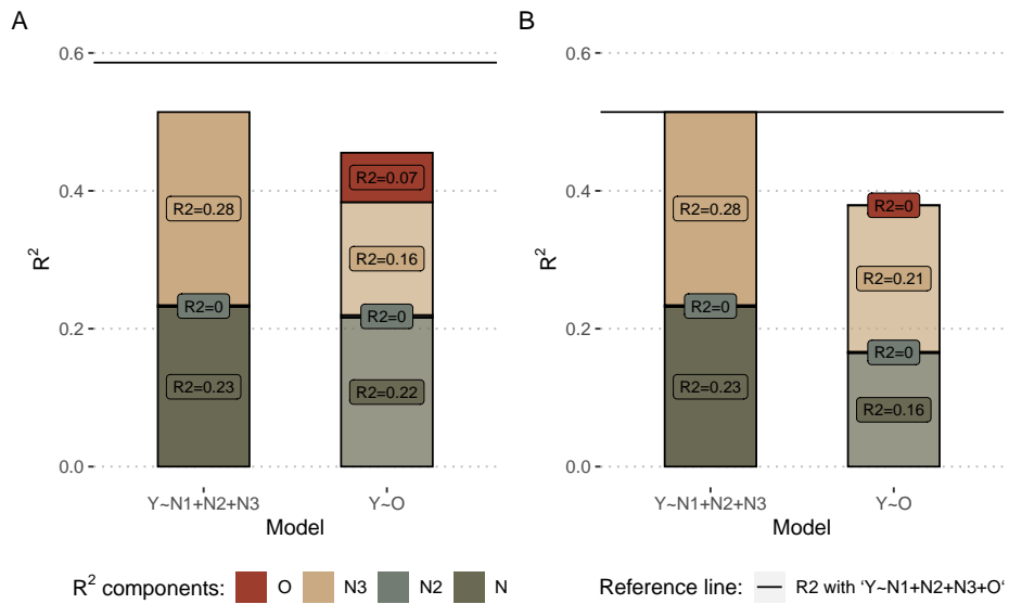
Figure 7.3: Decomposition of R^2 for inputs and output of example models. (A) Results for the non-linear model inputs and output O_{non-linear} as defined in Figure 7.2: the left column represents the R^2 decomposition of model Growth = \beta_0 + \beta_1 N_1 + \beta_2 N_2 + \beta_3 N_3 and the right column the R^2 decomposition of Growth = \beta_0 + \beta_4 O_{non-linear} . (B) Same with the linear model and the corresponding O_{linear} . For both (A) and (B), colors represent the origin of R^2 contribution according to the decomposition. In particular, for right columns (model Y \sim O ), the red share represent the proportion of the R^2 of the regressor O that does not come linearly from the inputs, and therefore its emerging part. The horizontal reference line corresponds to the maximal R^2 obtained from the model Growth = \beta_0 + \beta_1 N_1 + \beta_2 N_2 + \beta_3 N_3 + \beta_4 O
