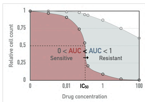
Figure A.2: Drug screening metrics in cell lines. Based on a tested drug concentration range, IC_{50} and area under the dose-response curve (AUC) can be computed. For a given drug, red AUC corresponds to a more sensitive cell line than blue AUC.
