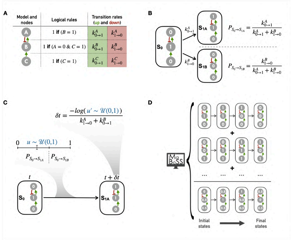
Figure 4.4: Main principles of MaBoSS simulation framework and Gillespie algorithm. (A) A logical model with regulatory graph, logical rules and transition rates. (B) A subset of the corresponding state transition graph with two possible transitions in asynchronous update for a given initial state; the probability probability associated with each transition comes from Gillespie algorithm. (C) Schematic diagram of the Gillespie algorithm applied to the asynchronous transition depicted in (B); random selection of a specific transition and time by the algorithm from two uniform random variables. (D) Schematic representation of a logical model simulation with MaBoSS: average trajectory obtained from the mean of many individual stochastic trajectories, each resulting from the succession of transitions as represented in (C).
