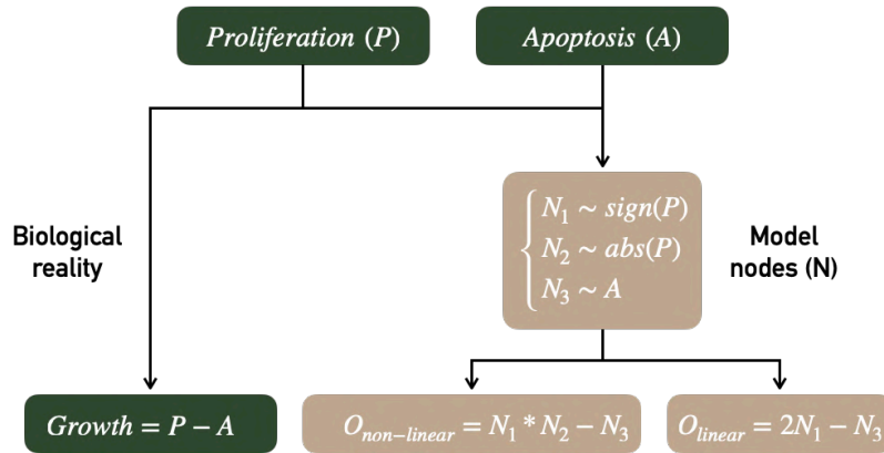
Figure 7.2: Evaluation of a mechanistic model. Adapted from Figure 1.6.
