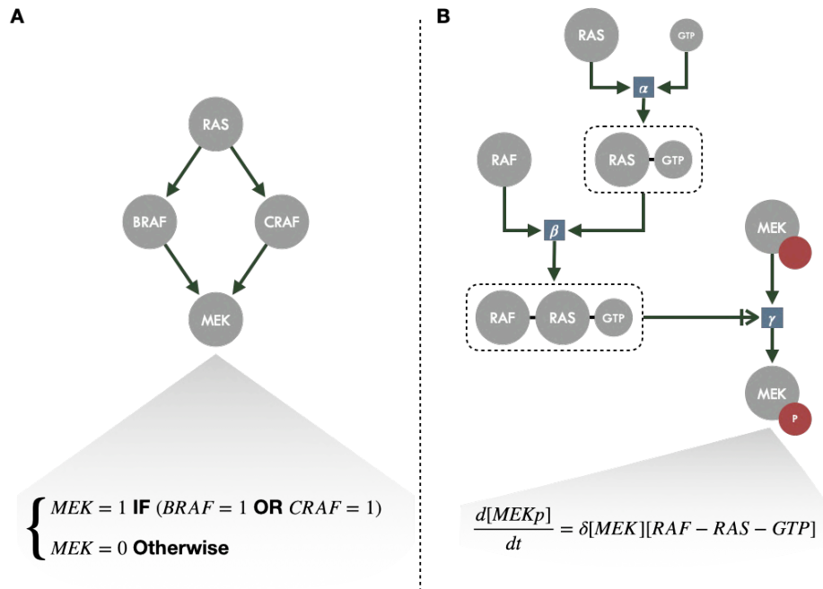
Figure 3.5: Schematic example of logical and ODE modeling around MAPK signaling. (A) Activity flow diagram of a small part of MAPK signaling, each node representing a gene or protein, with an example of logical rule for MEK node for the corresponding logical model. (B) Process description of the same diagram with BRAF and CRAF merged in RAF for the sake of simplicity; each square representing a reaction and the corresponding rate; an example differential equation is provided for the phosphorylated (active) form of MEK.
