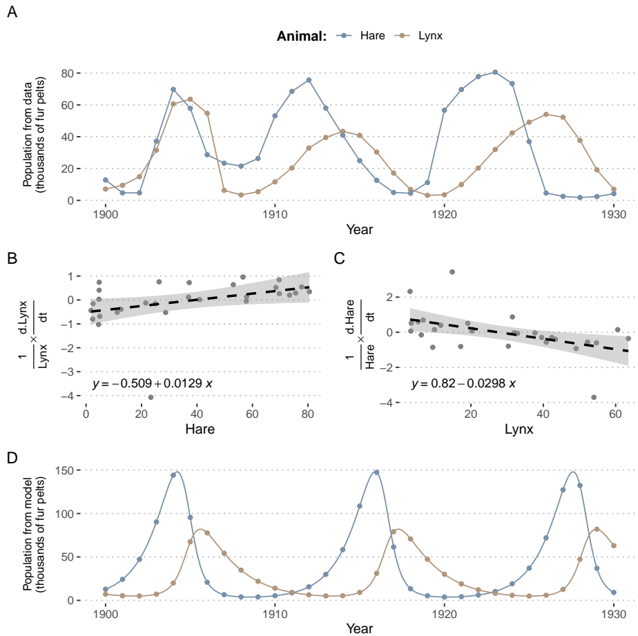
Figure 1.7: Some analyses around Lotka-Volterra model of a prey-predator system. (A) Evolution of lynx and hares populations based on Hudson Bay Company data about fur pelts. (B) and (C) Linear regression for estimation of parameters. (D) Evolution of lynx and hare populations as predicted by the model based on inferred parameters and initial conditions.
