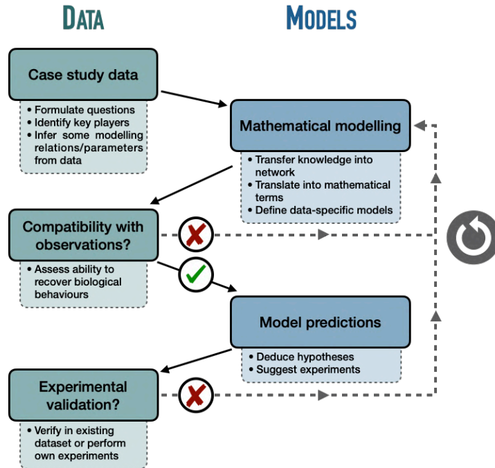
Figure 3.4: Modeling a biological network: an iterative and cyclical process. Reprinted from [Béal et al., 2020]. A different and simpler version of this cycle is described in [Le Novère, 2015].
