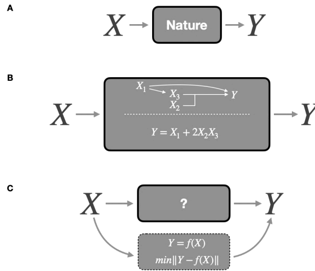
Figure 1.6: Different modeling strategies. (A) Data generation from predictors X to response Y in the natural phenomenon. (B) Mechanistic modeling defining mechanisms of data generation inside the box. (C) Statistical modeling finding the function f that gives the best predictions. Adapted from Breiman [2001b].
