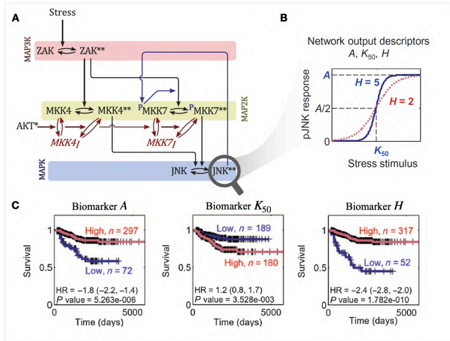
Figure 7.4: Mechanistic modeling of JNK pathway and survival of neuroblastoma patients , as described by Fey et al. [2015]. (A) Schematic representation (as a process description [Le Novere, 2015]) for the ODE model of JNK pathway. (B) Response curve (phosphorylated JNK) as a function of the input stimulus (Stress) and characterization of the corresponding sigmoidal function with maximum amplitude A , Hill exponent H and activation threshold K_{50} . (C) Survival curves for neuroblastoma patients based on binarized A , K_{50} and H ; binarization thresholds having been defined based on optimization screening on calibration cohort.
