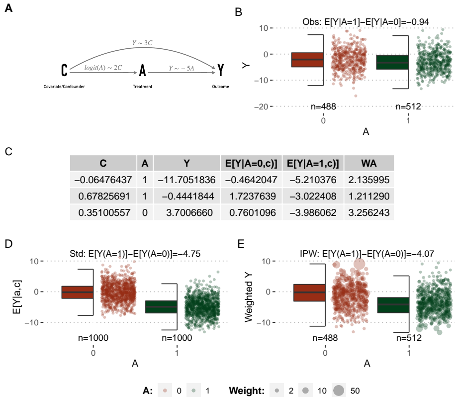
Figure 8.5: Causal inference methods on a simple example. (A) Directed acyclic graphs with causal relations between variables and parameters used to simulate data. (B) Association between A and Y from observed data. (C) Some simulated samples/patients with their original variables ( C , A and Y ), variables from outcome model ( E[Y|A = 0, c] , E[Y|A = 1, c] ) and weights from treatment model ( W^A ). (D) Standardized causal effect of A on Y based on and outcome modeling. (E) IPW causal effect of A on Y based on weights derived from treatment modeling; in this panel weights are taken into account in boxplots and estimations.
