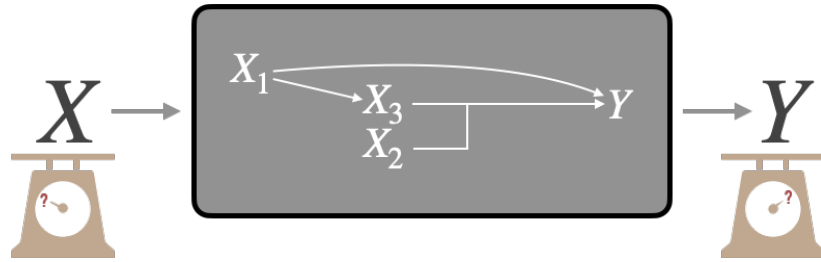
Figure 7.1: Evaluation of a mechanistic model. Adapted from Figure 1.6.
