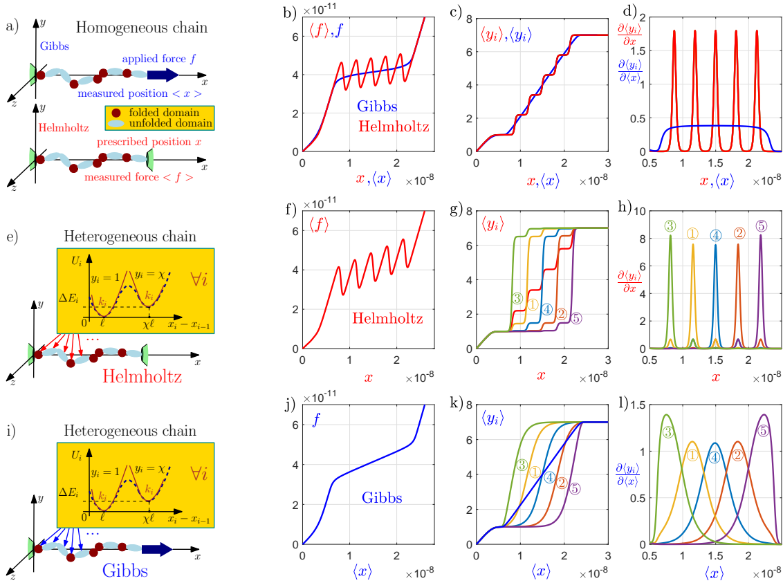
Figure 5.3 – Folding/unfolding processes in homogeneous and heterogeneous chains. Panel a): Gibbs and Helmholtz conditions in homogeneous chains. Panel b): force-extension response for isentensional (blue) and isometric (red) conditions. Panel c): average spin variables (homogeneous chain). All spins have the same behaviour (no unfolding pathway). Panel d): plot of the quantities \partial\langle y_i \rangle / \partial x (or \partial\langle y_i \rangle / \partial \langle x \rangle ) versus x (or \langle x \rangle ) for homogeneous chains (proportional to the probability density of the position of the unfolding transition of the i -th unit). Panel e): Scheme of an heterogeneous chain under isometric condition (different \Delta E_i and k_i ). Panel f): Helmholtz force-extension response, slightly modified by the heterogeneity. Panel g): the average spin variables under isometric condition show the pathway given by the ascending order of the values \Delta E_i : ③, ①, ④, ②, ⑤ (in this example \Delta E_3 < \Delta E_1 < \Delta E_4 < \Delta E_2 < \Delta E_5 ). Red curve: mean value \frac{1}{N} \sum_{i=1}^N \langle y_i \rangle of the averaged spins. Panel h): plot of the quantities \partial\langle y_i \rangle / \partial x , confirming the symmetry breaking induced by the heterogeneity. Panel i): scheme of an heterogeneous chain under isentensional condition (different \Delta E_i and k_i ). Panel j): Gibbs force-extension response, slightly modified by the introduction of the heterogeneity. Panel k): the average spin variables under isentensional condition show the unfolding pathway given by the ascending order of the values \Delta E_i : ③, ①, ④, ②, ⑤ (in this example \Delta E_3 < \Delta E_1 < \Delta E_4 < \Delta E_2 < \Delta E_5 , as before). Blue curve: mean value \frac{1}{N} \sum_{i=1}^N \langle y_i \rangle of the averaged spins. Panel l): plot of the quantities \partial\langle y_i \rangle / \partial \langle x \rangle , confirming the symmetry breaking induced by the heterogeneity. We adopted the following parameters: N = 5 , \ell = 0.5\text{nm} , T = 300\text{K} , \chi = 7 , k_i = 0.04\text{N/m} \forall i , \Delta E_i = 30k_B T \forall i in the homogeneous chain and \Delta E_1 = 27.5k_B T , \Delta E_2 = 32.5k_B T , \Delta E_3 = 25k_B T , \Delta E_4 = 30k_B T , \Delta E_5 = 35k_B T in the heterogeneous case [4].
