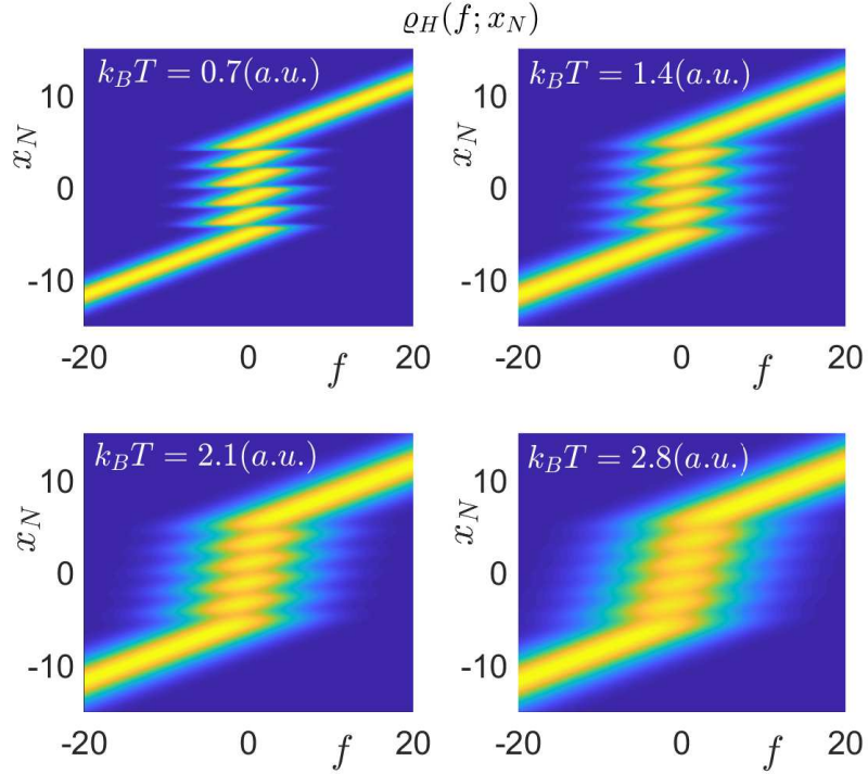
Figure 2.23 – Two-dimensional representation of the Helmholtz density \rho_H(f; x_N) (see Eq.(2.120)) obtained with N = 5 , \ell = 1 (a.u.), k = 15 (a.u.) and k_B T = 0.7, 1.4, 2.1, 2.8 (a.u.) [3].
