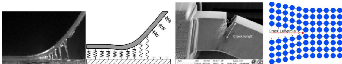
Figure 7.3 – Microinstabilities in the peeling process (left) and in the crack propagation (right) [243, 244].
