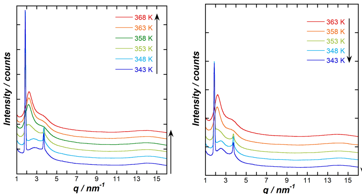
Figure S.II-14. SAXS diffractograms for [\text{Mn}_{12}\text{O}_{12}(\text{CF}_3\text{COO})_8(\text{L}^4)_8(\text{H}_2\text{O})_4] : (left) on 3 rd heating from 343 to 368 K and (right) on 3 rd cooling from 363 to 343 K.
