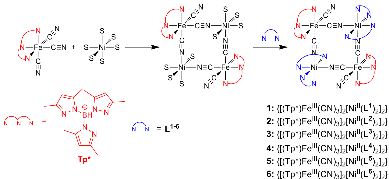
Scheme IV-4. Synthetic scheme of the approach used to obtain cyanido-bridged \{Fe^{III}_2Ni^{II}_2\} molecular squares. Charges on metal ions and counter-ions omitted for clarity.
