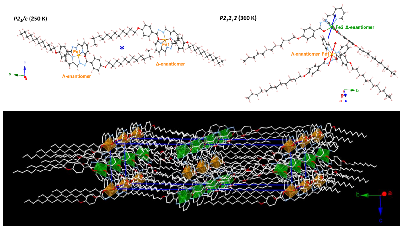
Figure III-35. (Top) Views of the two [Fe(L^4)_2] enantiomers at 250 K (left) and 360 K (right). The blue star represent the inversion center of symmetry relating the two crystallographically equivalent enantiomers in the P2_1/c space group. The blue and red vectors represent the 2-fold symmetry axes crossing the two non-equivalent isomers in the P2_12_12 space group. (bottom) projection of the packing at 360 K, emphasizing the distribution of LS (orange) and HS (green) species in the space. H-atoms are omitted for clarity.
