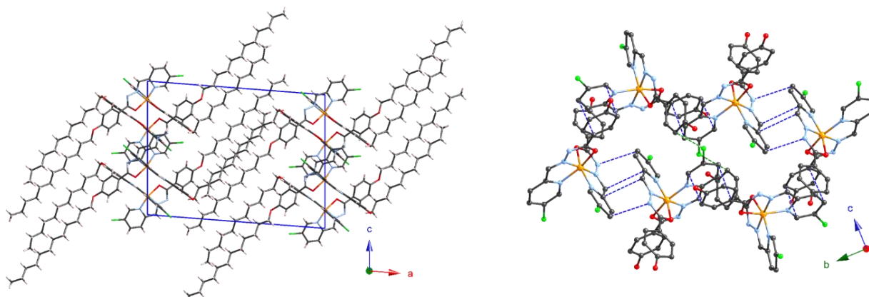
Figure III-39. Projection of the packing for [Fe(L^5)_2] at 120 K viewed along b -axis (left) and a -axis (right). The \pi - \pi and Cl \cdots \pi interactions are shown as blue and green dashed lines, respectively. In the right figure, dodecyl chains, hydrogen atoms and other C \cdots X interactions ( X = O, N, \pi ) are omitted for clarity.
