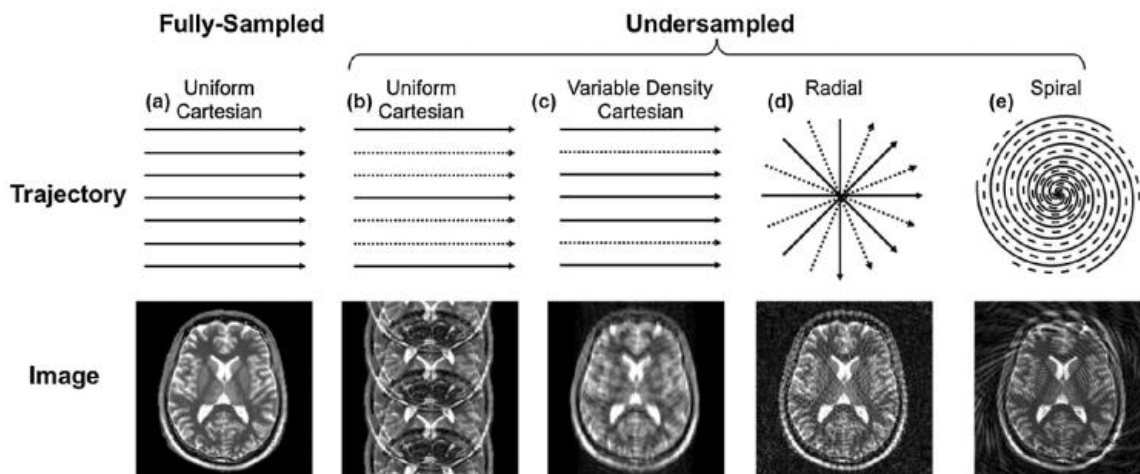
Figure 2.18 – Examples of different k-space trajectories and their associated aliasing artifacts, adapted from [114].
