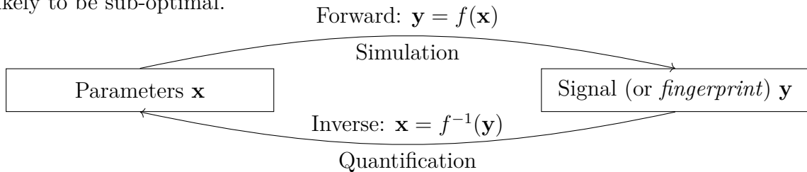
Figure 3.1 – Magnetic resonance fingerprinting as an inverse problem.
