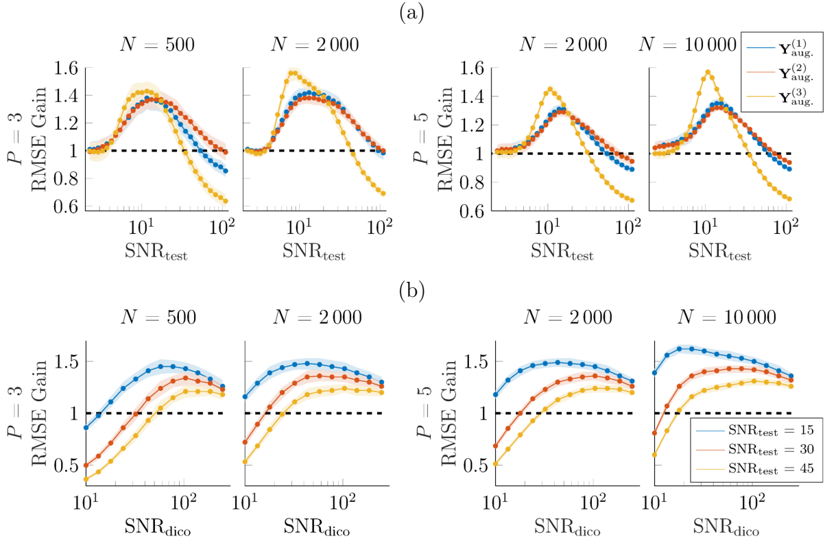
Figure 3.5 – RMSE gains for different data augmentations and noise levels on dictionary signals.
