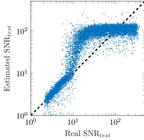
Figure 4: Estimated \text{SNR}_{test} as a function of real \text{SNR}_{test} , using the dictionary-based learning (DBL) method. The dashed line represents the identity function (perfect estimation).
