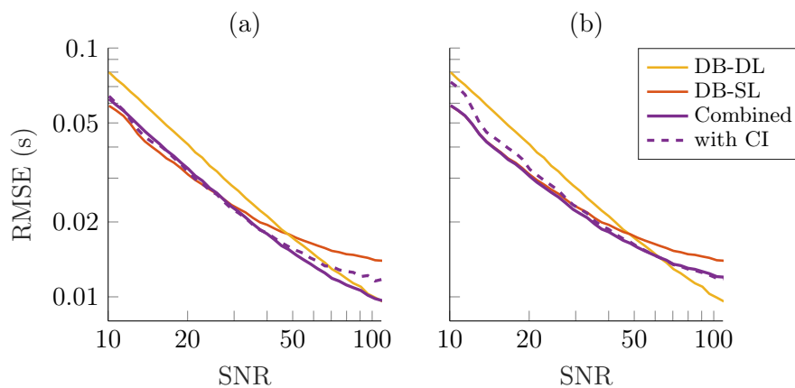
Figure 4.10 – Combination of statistical and deep learning methods, using synthetic scalable signals.
