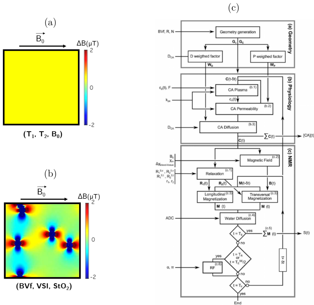
Figure 2.27 – Sketch of the simulation algorithm, adapted from [152].
