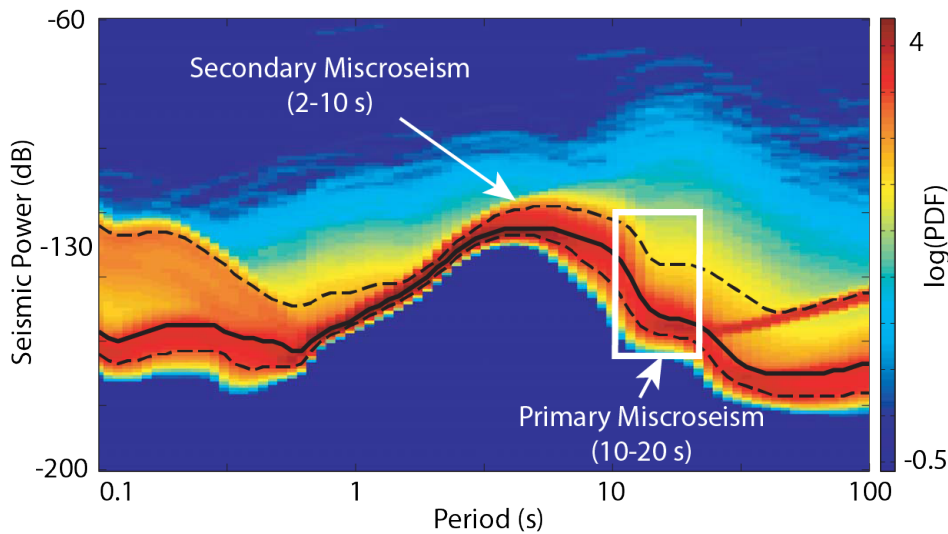
Figure 7.2: Probability density function of power spectral density (PSD) for the vertical-component of South Pole station QSPA (146 m borehole) for December 2007–December 2012. Adapted from Anthony et al. (2015).
