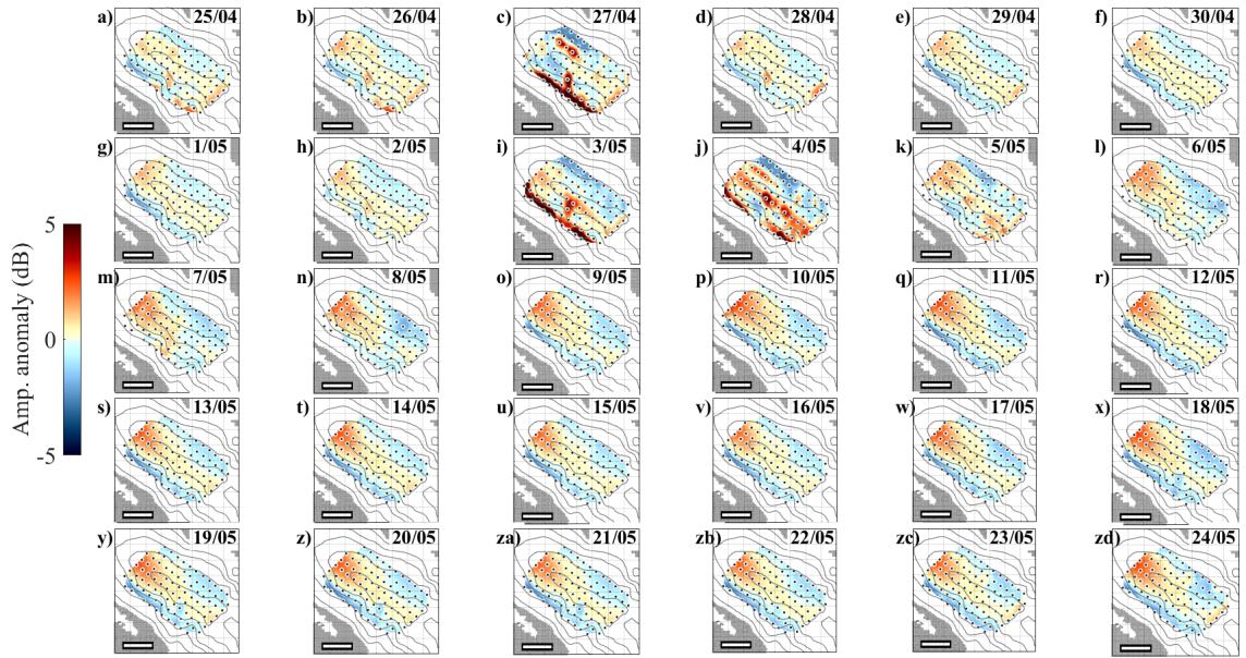
Figure 10.1: 2D maps of the seismic amplitude anomaly associated with subglacial water flow. Temporal evolution of the spatial pattern of the amplitude anomaly obtained for the 5 \pm 2 Hz frequency range. All maps are daily average of 2 hours-amplitude anomalies. Colour scales ranges are equal for each time window and represent the amplitude anomaly in decimal logarithmic (dB) relative to (\text{m.s}^{-1})^2 \cdot \text{Hz}^{-1} . Contour lines show ice thickness as presented in Figure 1. Grey shaded areas show ice-free areas and scale is 200 m for the white stripes. For graphical purpose I linearly interpolated the seismic power at each sensor over a sub-meter grid that covers the seismic-array.
