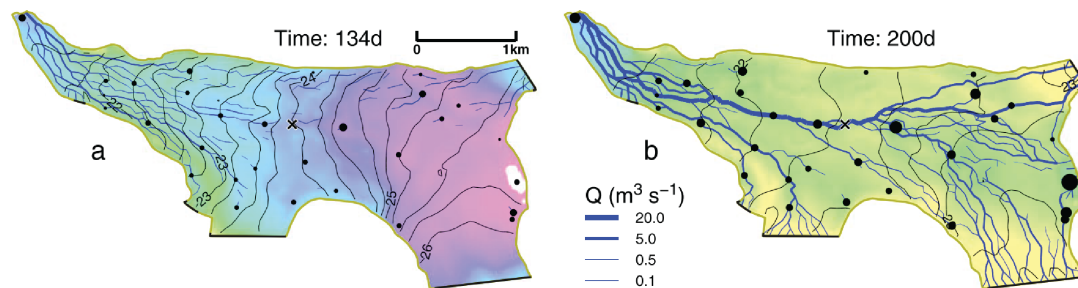
Figure 1.7: From Werder et al. (2013) Simulation 2007 melt season for Gornergletscher. Snapshot of the trunk on (a) 14 May and on (b) 19 July at the time of peak input, showing contours of hydraulic potential \phi (MPa), effective pressure N , the channel discharge Q , moulin input (dots), and inflow boundaries (black lines).
