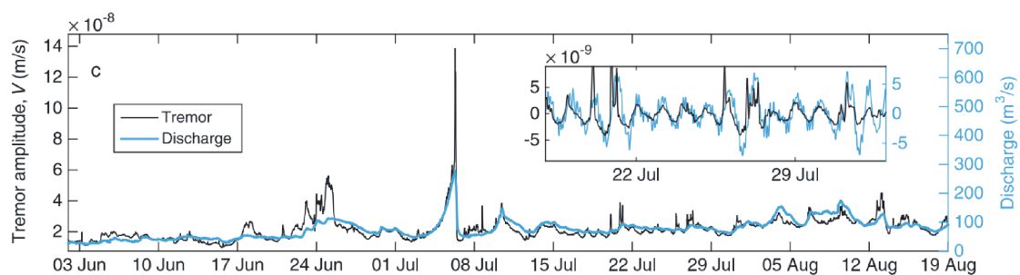
Figure 1.9: From Bartholomaeus et al. (2015a) Tremor amplitude and water discharge into Mendenhall Lake in which terminates Mendenhall glacier. Tremor is calculated within [1.5-10] Hz.
