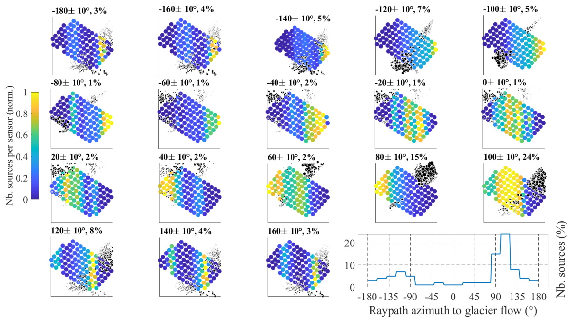
Figure 11.2: Number of events seen by each station for a given sources-to-station ray path azimuth with respect to glacier flow, i.e. azimuth 0° is along glacier flow. Color indicates the relative number of event number of events and each panel represent a 20° azimuth range. Black dots show event location whose size corresponds to how much the illuminate the array. Colorbar is scaled for each azimuth to the number of raypath analyzed within the given azimuth. The relative number of ray path per azimuth is shown in the last panel.
