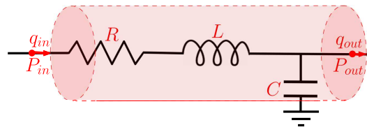
Figure 5.2: A single compartment circuit illustration.
