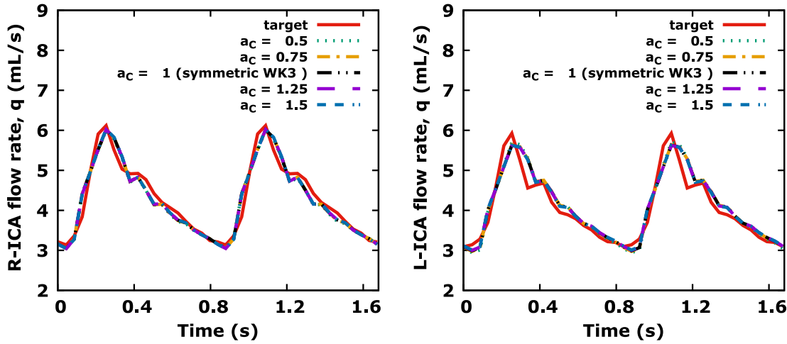
Figure 4.19: Comparison of the model simulated blood flow rate waveform using WK3 with the same resistances and different compliances for left and right pairs of ICAs' terminal compartments.
