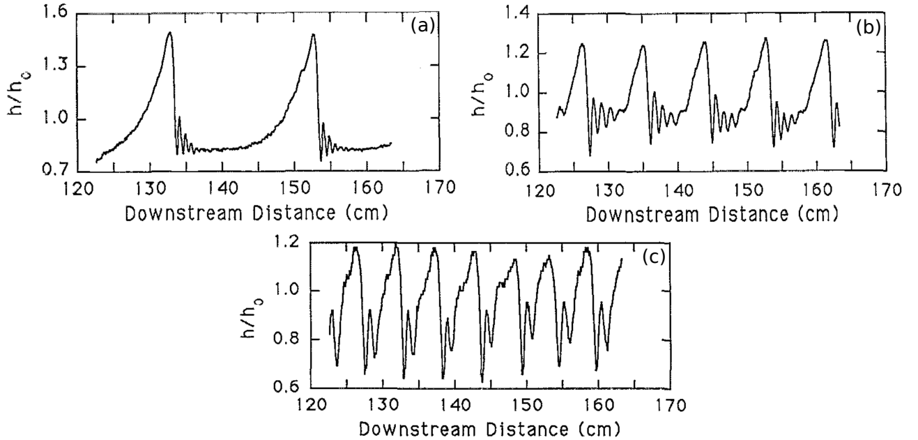
Figure 3.8: Dimensionless water depth as a function of the downstream distance \tilde{x} for different frequencies : (a) \tilde{f} = 1.5Hz , (b) \tilde{f} = 3.0Hz and (c) \tilde{f} = 4.5Hz in the experiments of Liu & gollub [57]. Figures reprinted from J. Liu and J. P. Gollub. “Solitary wave dynamics of film flows”. In: Physics of Fluids 6.5 (1994), pp. 1702–1712, with the permission of AIP Publishing.
