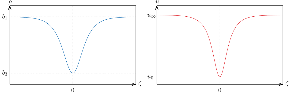
Figure 2.1: Overall shape of the gray soliton solution in terms of the variables \rho and u for arbitrary values of the parameters b_1 and b_3 at t = 0
