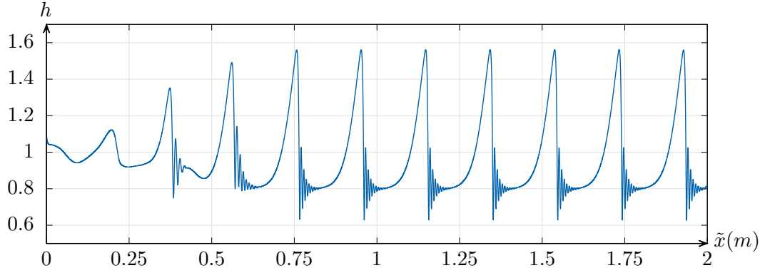
Figure 3.7: Dimensionless water height as a function of space (dimensioned), in the setting of the Liu & Gollub experiment, for an imposed frequency of 1.5Hz . (Obtained through numerical simulation). Parameters used here are : Re = 19.33 , \kappa = 1.440 \cdot 10^{-4} , Fr = 0.8476 , \theta = 6.4^\circ
