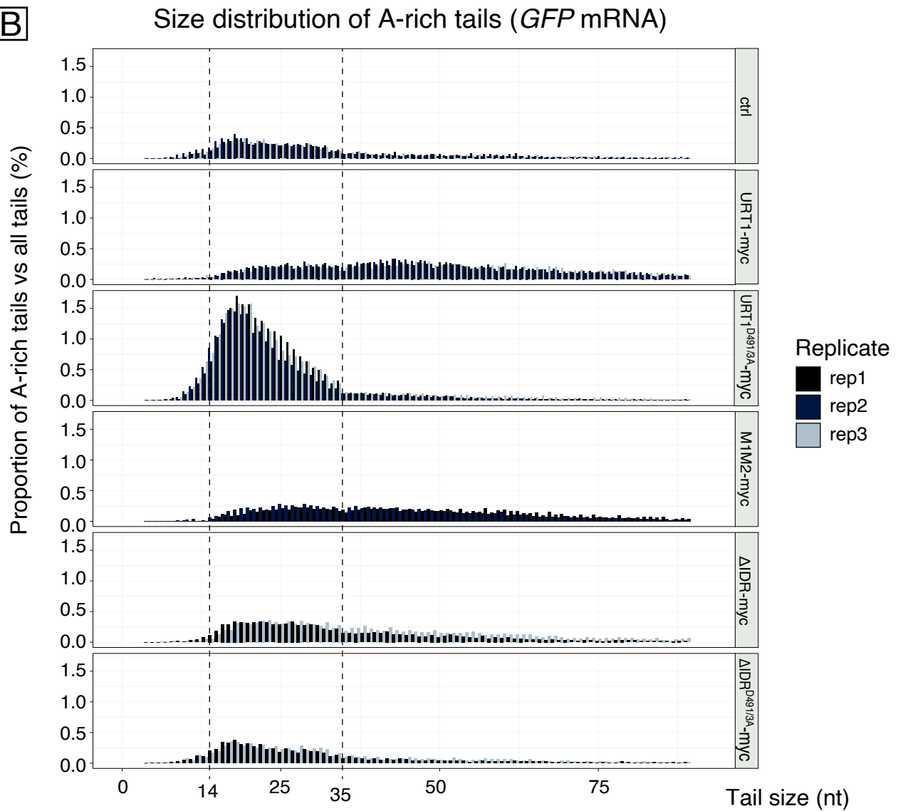
Figure 23: Expression of URT1 D491/3A -myc leads to accumulation of short A-rich tails.
