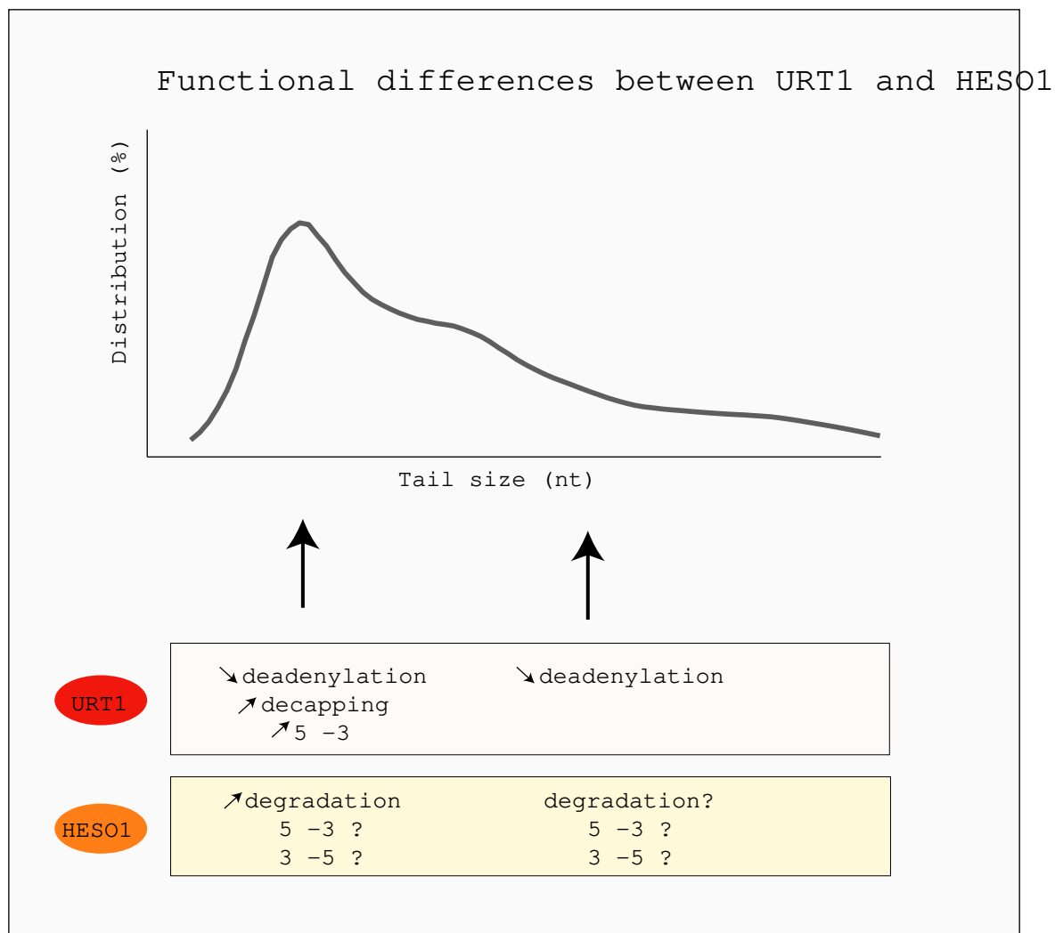
Figure 42: Summary chart of the possible functions of URT1 and HES01. URT1 uridylylated preferentially short, but also longer polyA tails. The main function is down deadenylation. It is also promoting the decapping and degradation from 5' to 3' short polyA tails of 10-20 nucleotides. Thus, URT1 prevents the accumulation of ex-lated mRNAs (<10 nucleotides). HES01 is preferentially targeting short polyA tails to promote their fast degradation if HES01 promotes the degradation from 5' - 3' or from 3' - 5'.
