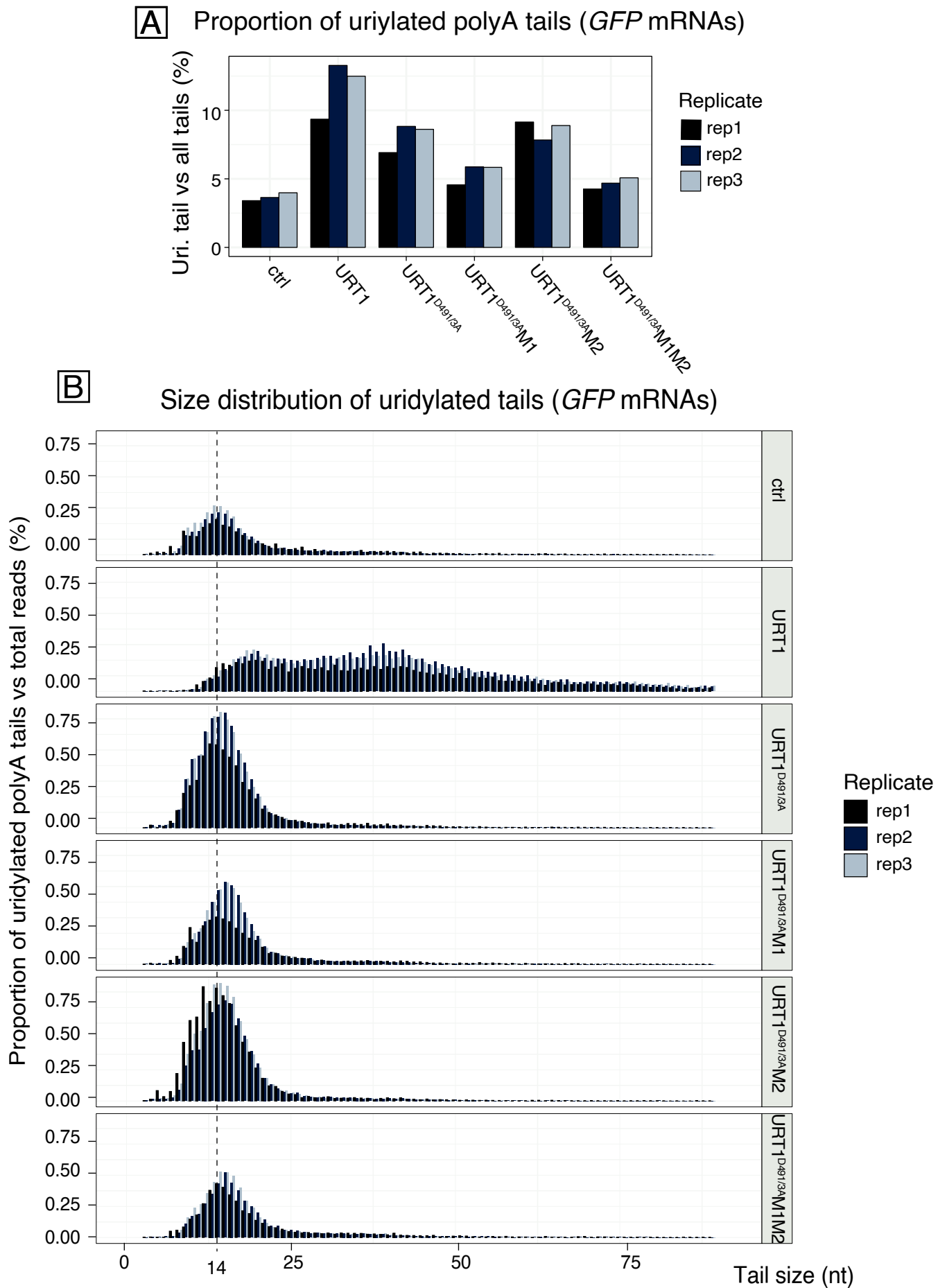
Figure 31: Size distribution of uridylated polyA tails of GFP mRNA.
