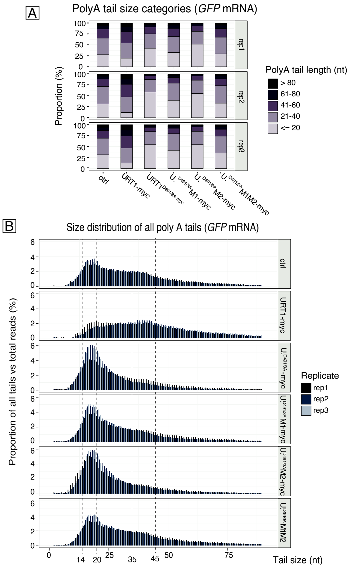
Figure 30: Size distribution of all tails of GFP mRNAs.
