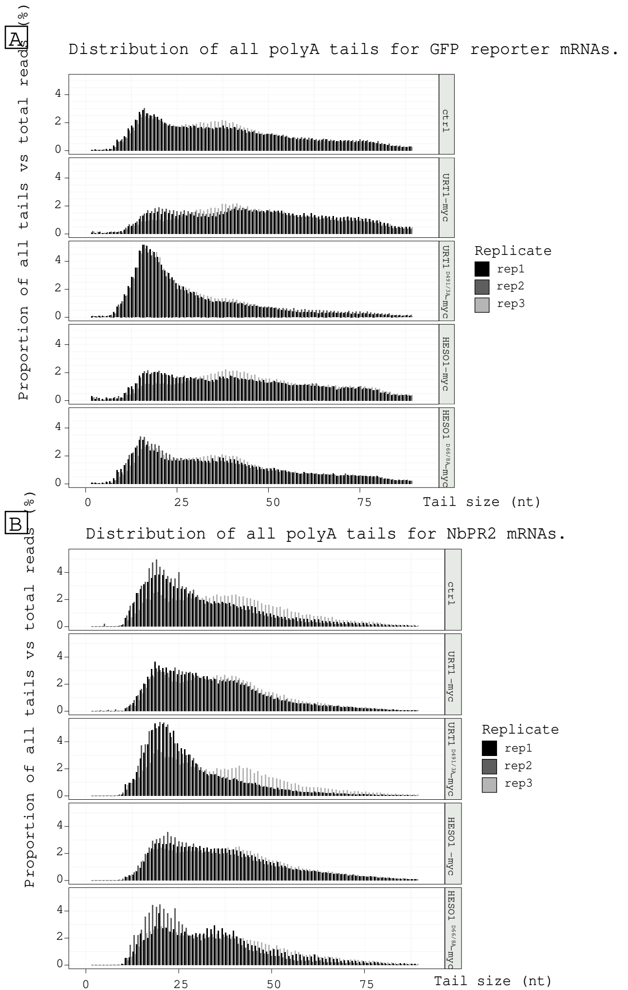
Figure 40: Distribution of all polyA tails for GFP and NbPR2 mRNAs.
