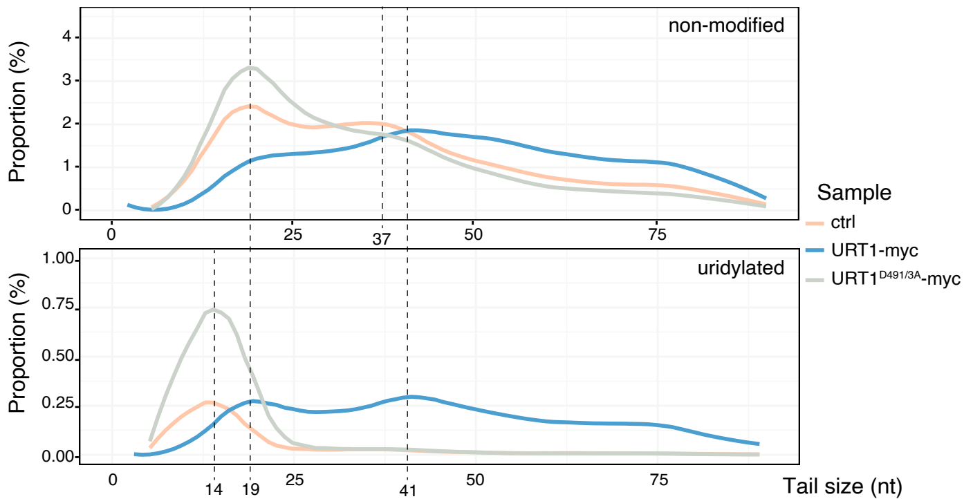
Figure 19: Size distribution of unmodified polyA tails and uridylated polyA tails.
