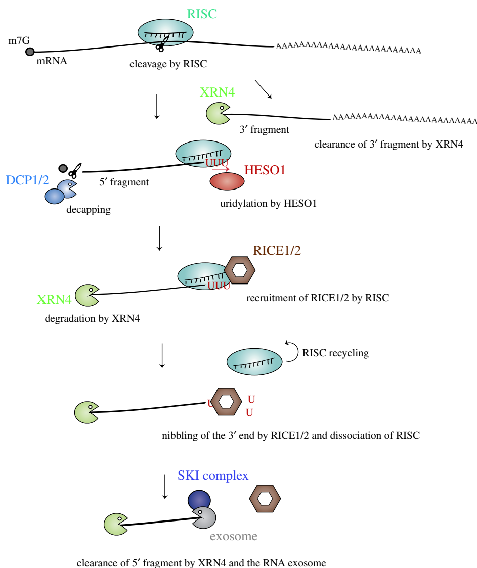
Figure 8. Uridylation by HESO1 promotes degradation of 5' fragments of RISC-cleaved mRNAs. RISC cleavage of mRNAs generates a 3' cleavage fragment that is degraded by XRN4, and a 5' cleavage fragment. The 5' cleavage fragment is uridylated by HESO1, which binds RISC, but can also be decapped by the DCP1/2 complex. The exoribonucleases RICE1/2, which are recruited by RISC, nibble the uridylated 5' cleavage fragment. This nibbling helps RISC dissociation and RISC recycling. Finally, the 5' cleavage fragment is degraded by XRN4 and the RNA exosome.
