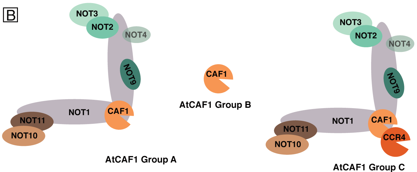
Figure 10: Plant CCR4/NOT complex.
