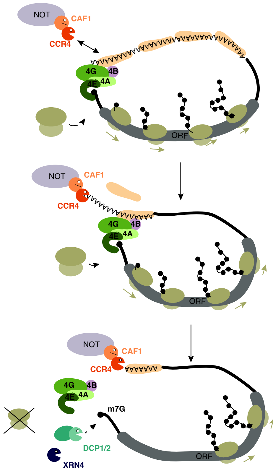
Figure 8: mRNA de-circularisation by deadenylation.
