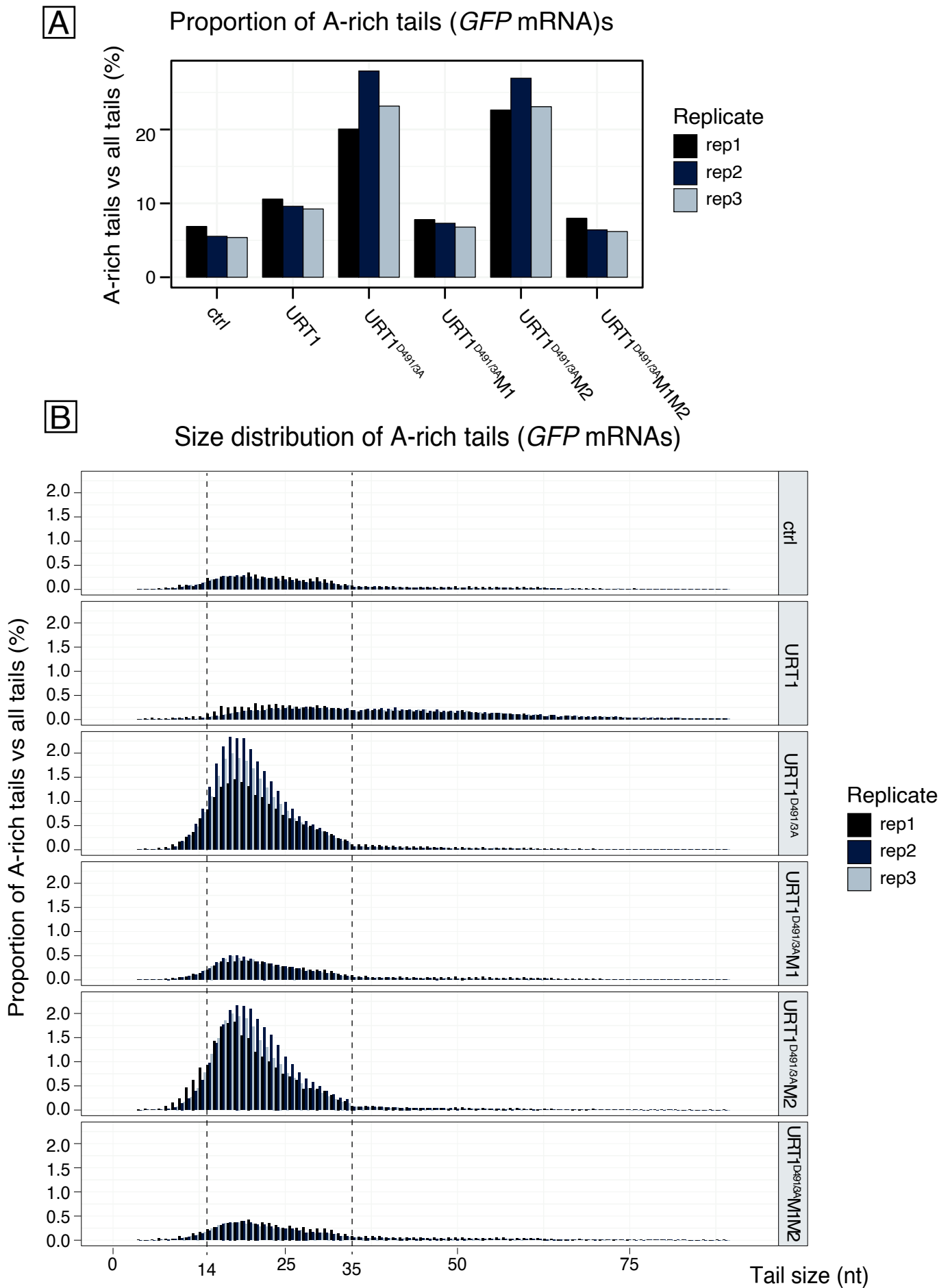
Figure 32: Size distribution of A-rich tails of GFP mRNAs.
