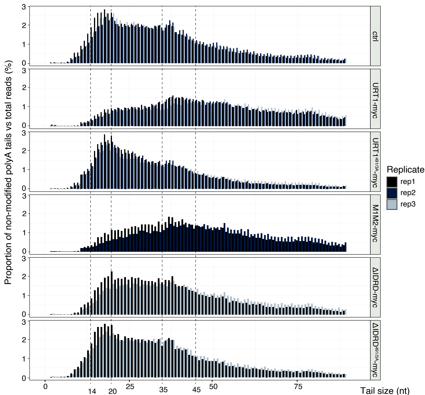
Figure 22: The N-terminal IDR is important for the regulation of polyA tail sizes by URT1.
