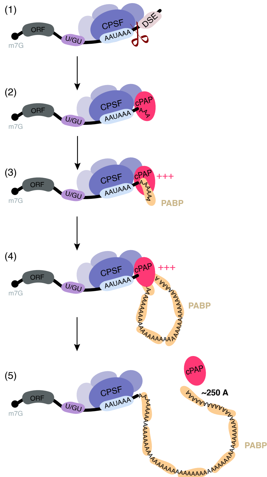
Figure 2: Polyadenylation of mRNAs in humans.
