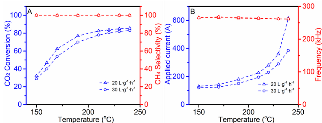
Fig. 5. CO 2 conversion and CH 4 selectivity as a function of reaction temperature (A) and corresponding applied current and frequency (B) with different GHSV (STP) = 20 L·g cat -1 ·h -1 and 30 L·g cat -1 ·h -1 under IH mode on the 40Ni/Al 2 O 3 catalyst. Reaction conditions: 0.4 g catalyst, H 2 -to-CO 2 ratio (v/v.) of 4 and 0.1 MPa.
