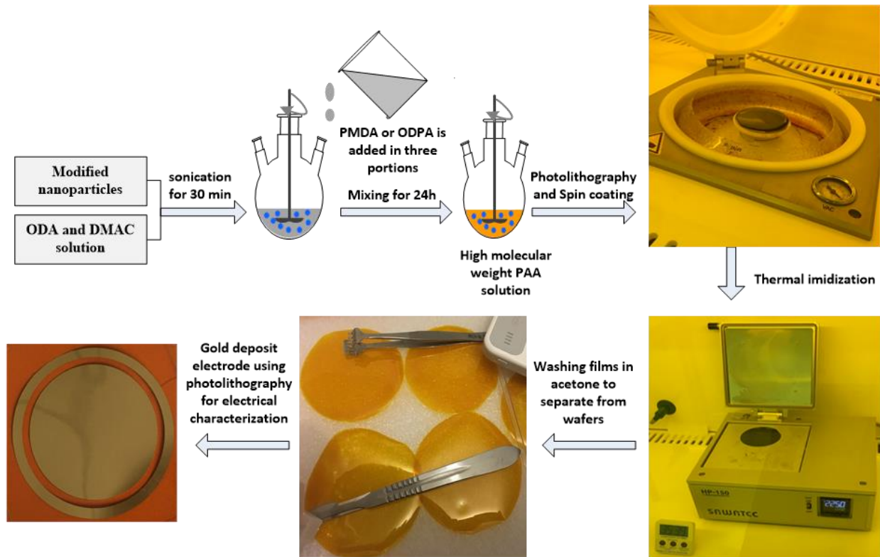
Figure 2.9 Polyimide films synthesis process
