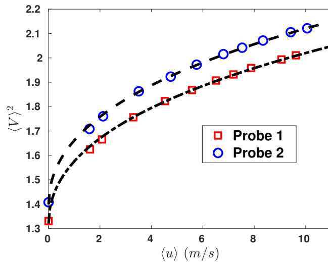
Fig. A.2 The mean voltage across the filament of hot-wire probes versus the mean velocity perpendicular to the filament. Probe 1 (red squares) and Probe 2 (blue circles). Black dashed and dotted dashed lines denote the fit using eqn.(A.1).
