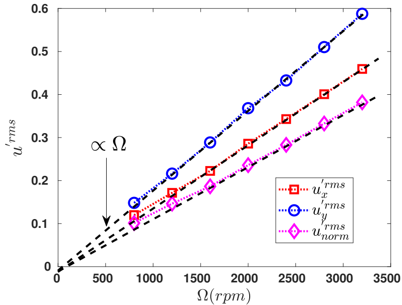
Fig. III.24 The RMS of velocity along x , y axes denoted by u_x'^{rms} (red squares), u_y'^{rms} (blue circles) and the RMS of the norm of velocity u_{norm}'^{rms} (magenta diamonds) versus the rotation rate of motors \Omega . Black dashed line denote linear dependence.
