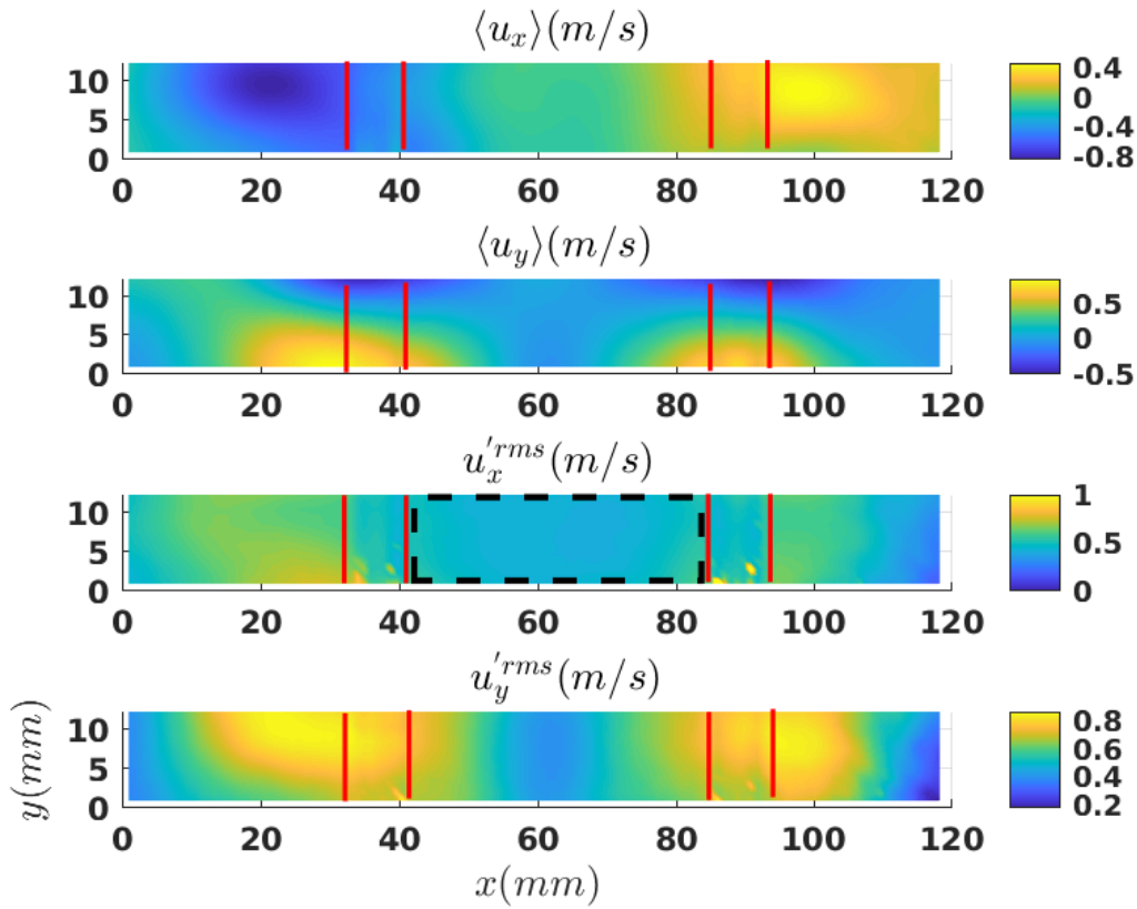
Fig. III.23 Mean and RMS of velocity fluctuations for \Omega = 3200 rpm. From top to bottom: \langle u_x \rangle , \langle u_y \rangle , u_x'^{rms} and u_y'^{rms} . Red lines mark the outlines of the axes. Black dashed box denotes the area in which homogeneity for u_x'^{rms} is observed.
