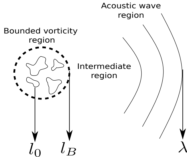
Fig. IV.2 Sketch of weakly compressible flow with region of bounded vorticity, intermediate region and region with acoustic waves.
