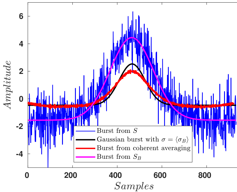
Fig. II.26 Blue: The sample of the noisy bursting signal S with one burst that is chosen to initialize the process of coherent averaging. Black: A Gaussian burst with standard deviation of \sigma = \sigma_B . Red: The burst obtained after the method of coherent averaging. Magenta: The sample of the bursting signal S_B with one burst.
