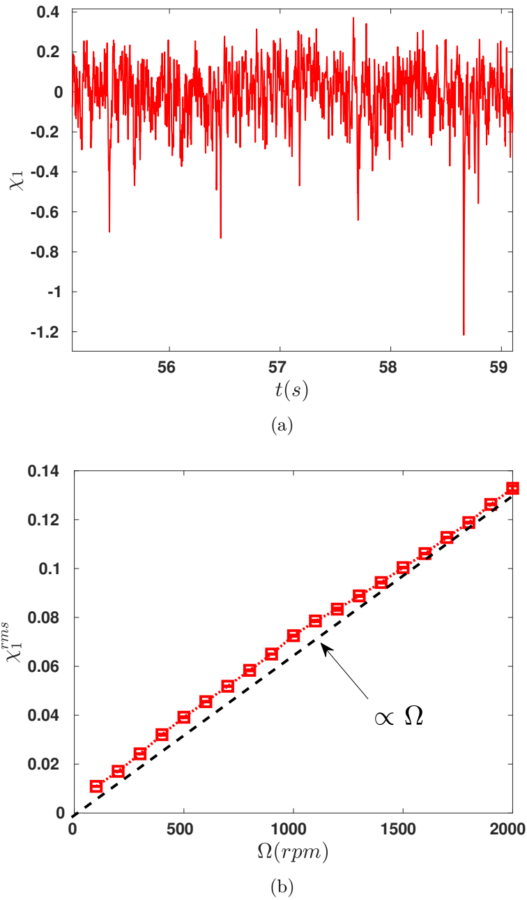
Fig. IV.12 (a) Time series of log-amplitude fluctuations for \Omega = 2000\text{rpm} . Note that the signal displays sharp negative peaks. (b) Scaling of RMS of log-amplitude fluctuations \chi_1^{rms} with the rotation rate \Omega . Dashed line shows the scaling as predicted from dimensional analysis.
