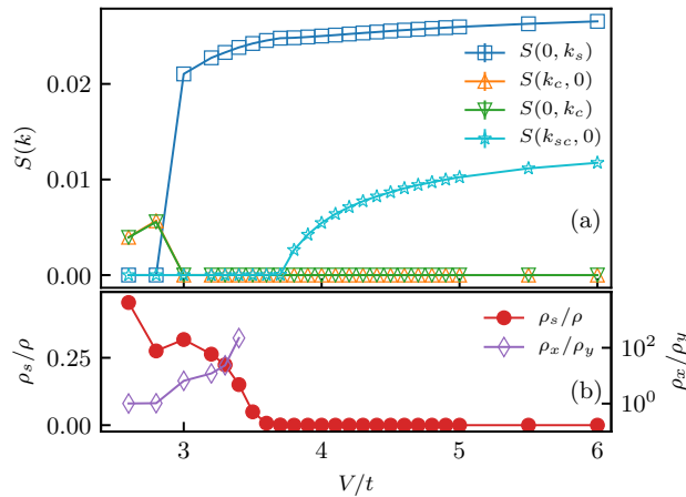
Figure 1.10.: Panel (a): Structure factor S(\mathbf{k}) as a function of V/t for values of lattice wave vector \mathbf{k} = (k_c, 0) (up-pointing triangles), (0, k_c) (down-pointing triangles), (0, k_s) (squares), (k_{sc}, 0) (stars) characteristic of the IS, SS, and SC ordered phase, respectively (see text). Here k_c = 2\pi \times 7/24 and k_s = 2\pi \times 1/3 . Panel (b): Superfluid fraction \rho_s/\rho (circles), and ratio between the superfluid responses \rho_x/\rho_y along the x horizontal and y vertical axis (diamonds). Data taken from calculations with N = 96 \times 96 , \rho = 1/6 , and T/t = 1/20 .
