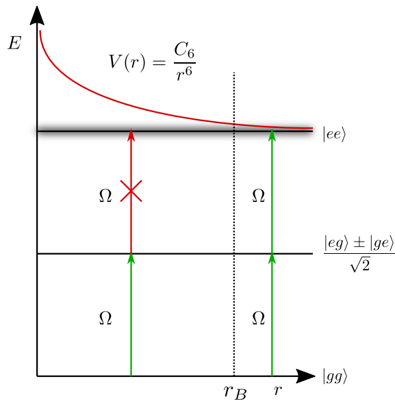
Figure C.1.: Representation of the dipole blockade: due to the shift caused by the ( van der Waals ) interaction between two Rydberg-excited atoms, the formation of a doubly excited pair is forbidden. The blockade effect extends within a blockade radius, that depends on the parameters of the excitation process.
