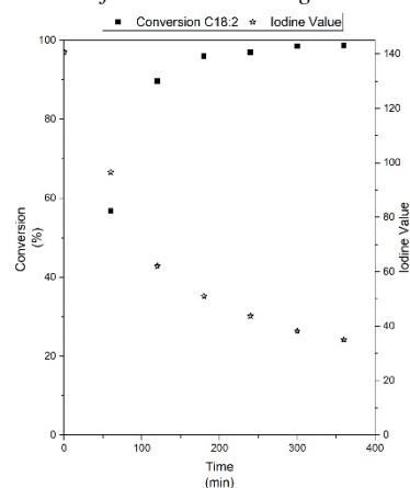
Figure A-285 Test 79 conversions of C18:2, and Iodine Value trend
