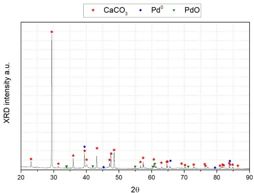
Figure 3-3 XRD spectra of Lindlar catalyst with \text{CaCO}_3 , \text{Pd}^0 , and \text{PdO} principal rays reported.
