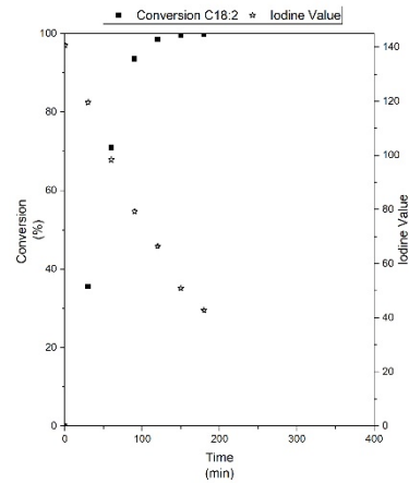
Figure A-258 Test 70 conversions of C18:2, and Iodine Value trend
