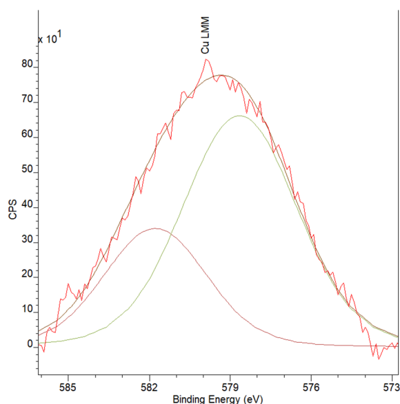
Figure 3-32 XPS \text{Cu}_{10}\text{Pd}_1\text{SiO}_2\text{AE} reduced Cu LMM.
