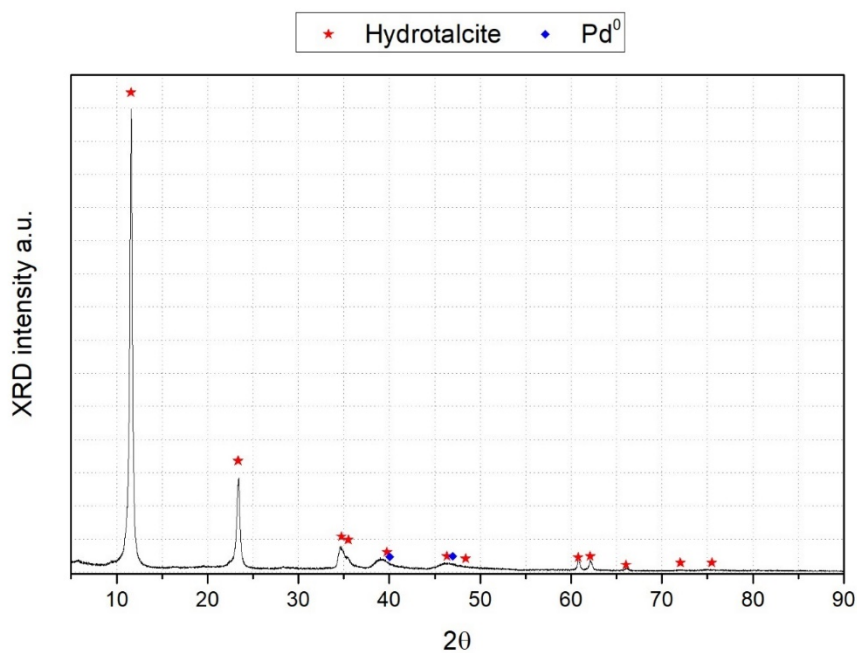
Figure 3-6 XRD spectra of Pd/HT catalyst with hydrotalcite phase ( C_{0.167}Al_{0.333}Mg_{0.667}O_{3.001} ) and Pd 0 rays highlighted.
