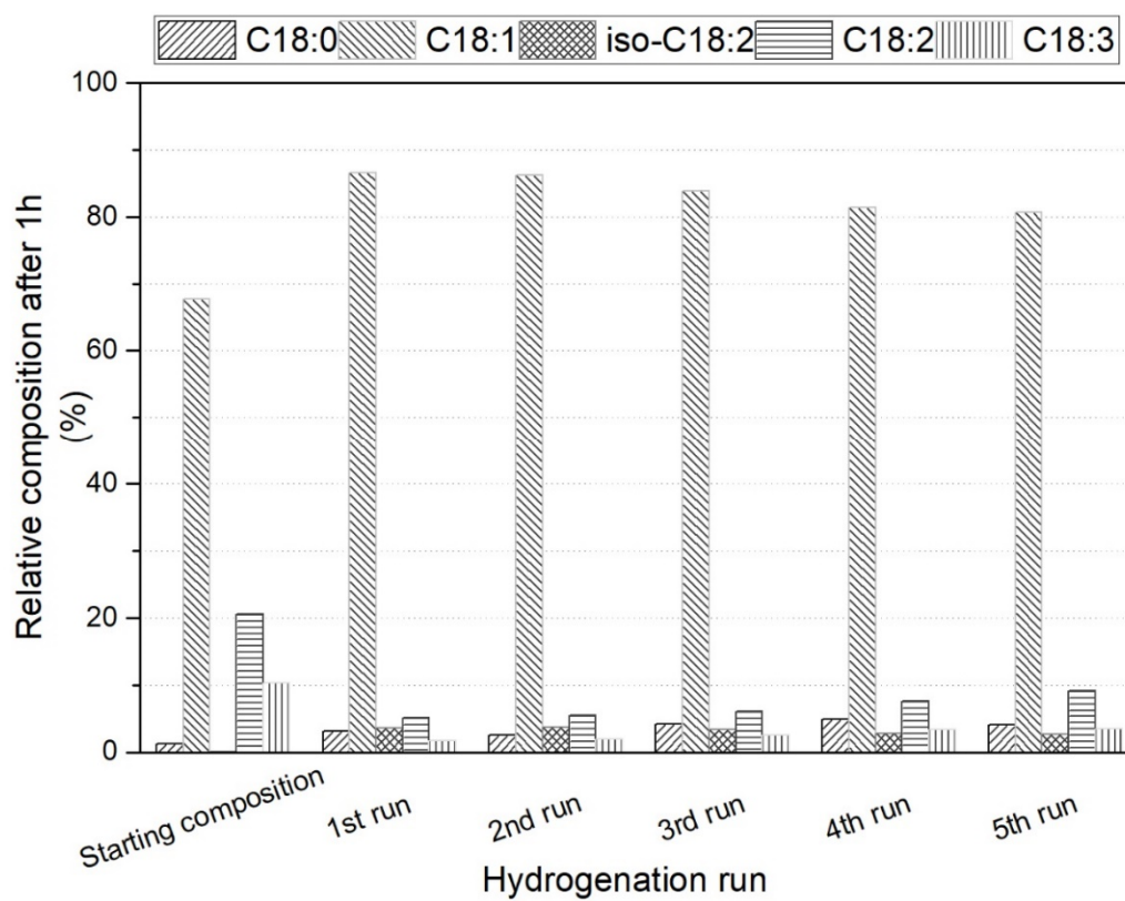
Figure 4-4 Hydrogenated oil composition at 1h over five cyclic tests at 180°C under 4 bar pressure (test 09-13)
