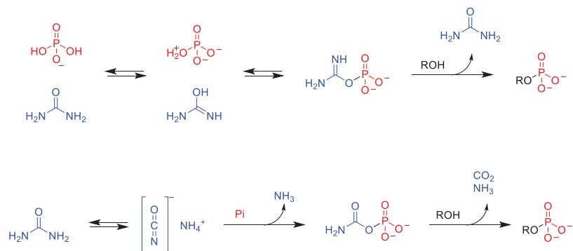
Scheme 2.16 Urea-promoted phosphorylation of alcohols. Top: through a rare phosphate tautomer with catalytic urea. Bottom: through an isocyanate with urea consumption.
