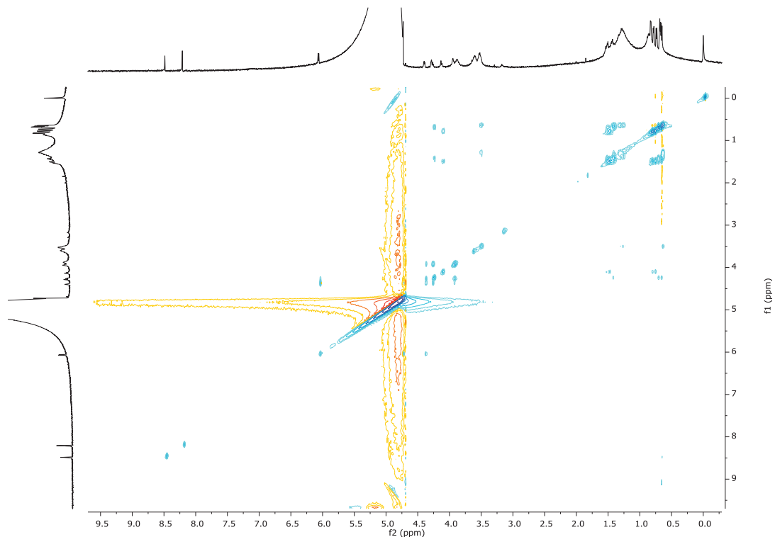
Figure S 32 ^1\text{H} - ^1\text{H} DIPSY NMR ( \text{D}_2\text{O} , 500 MHz) of Leu3A embedded in LA/MLG membranes after gel filtration separation. Lipids did not give cross-signals likely because of too fast translational relaxation (short T_2 ).
