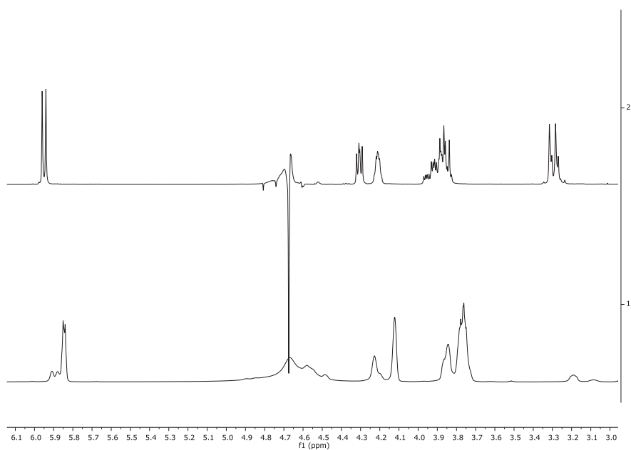
Figure S3 Stacked view of ^1\text{H} NMR spectra ( \text{D}_2\text{O} , 500 MHz) of pure Val 2 A in bicarbonate buffer (top) and in borate buffer (bottom). The broadening of the signals in borate is caused by the formation of a complex between borate ions and the 2'-3' diol of the nucleotide. This effect was also evidenced by NMR by Benner and coll. 464
