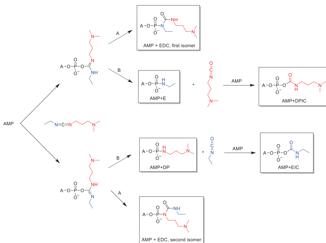
Scheme 3.7 Mechanistic proposition for the formation of by-products from EDC-activated nucleotides. Pathway A represents the usual rearrangement leading to stable N-phosphorylureas. Pathway B was postulated to yield stable phosphoramidates and isocyanates that further reacted to give carbamoyl phosphates. Each pathway could apply to the two isomers of EDC-activated AMP, leading to a total of 6 by-products. All the corresponding species have been observed in LC/MS analysis.
