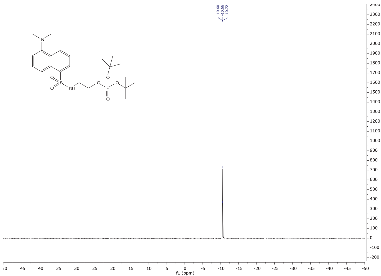
^{31}\text{P} NMR (MeOD, 120 MHz) of (31)
