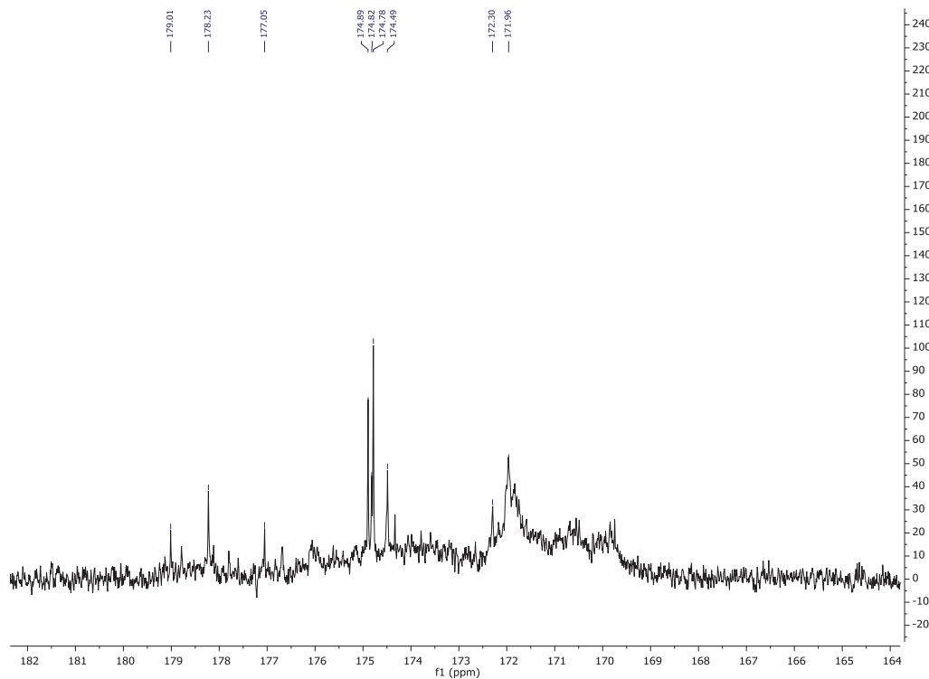
Figure S25 ^{13}\text{C} NMR ( \text{H}_2\text{O} , 100 MHz) for an assay involving saturated butanol and 200 mM 1\text{-}^{13}\text{C} glycine in the presence of 500 mM acetaldehyde. The butyl ester peak was not detected. The broad, unresolved aspect of the spectrum is consistent with the formation of a dark brown tar in the sample.
