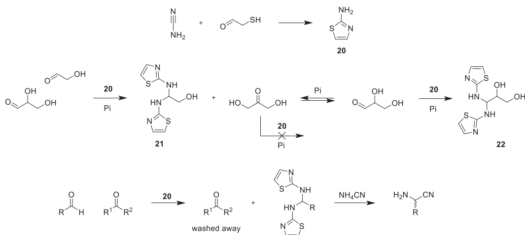
Scheme 2.8 Selective precipitation of aldehydes as amins of 2-aminothiazole (20). Top: formation of (20). Middle: stepwise precipitations of glycolaldehyde and glyceraldehyde depletes dihydroxyacetone. Bottom: selective formation of \alpha -aminonitriles of aldehydes in the presence of ketones.
