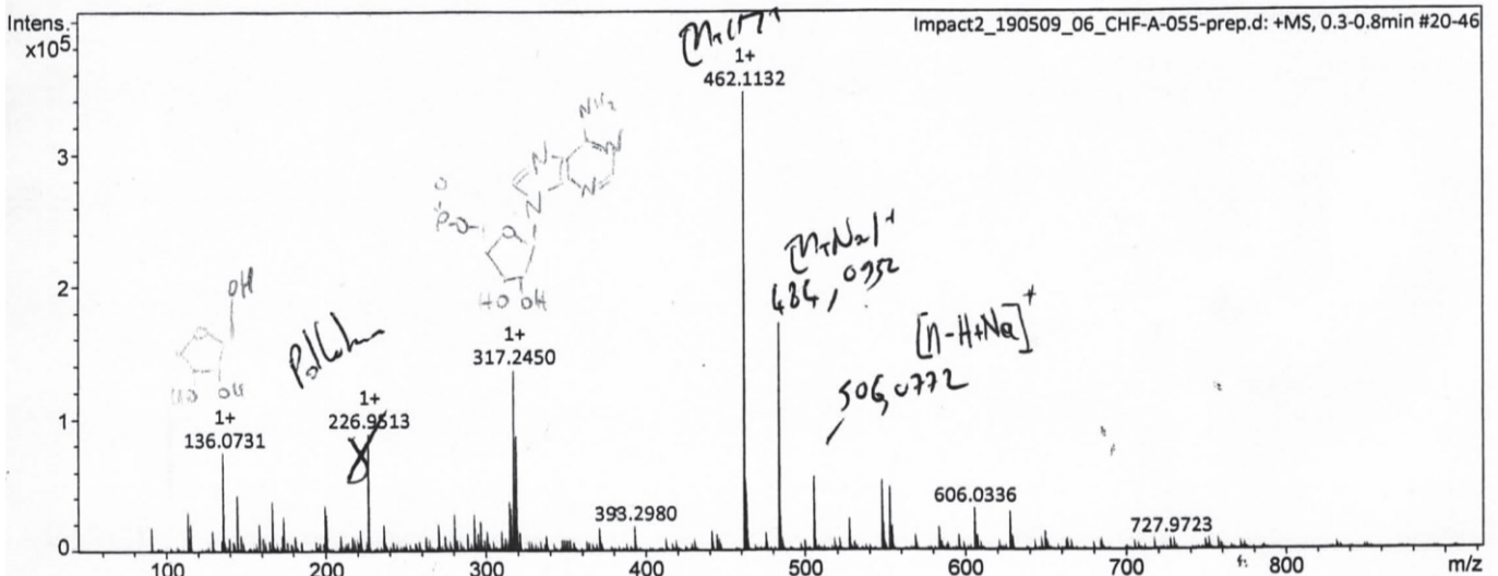
HRMS (+MS) of Gly 2 A. The fragments visible at 136 (adenine) and 317 (dehydrated AMP) are typical from peptido-AMP.
