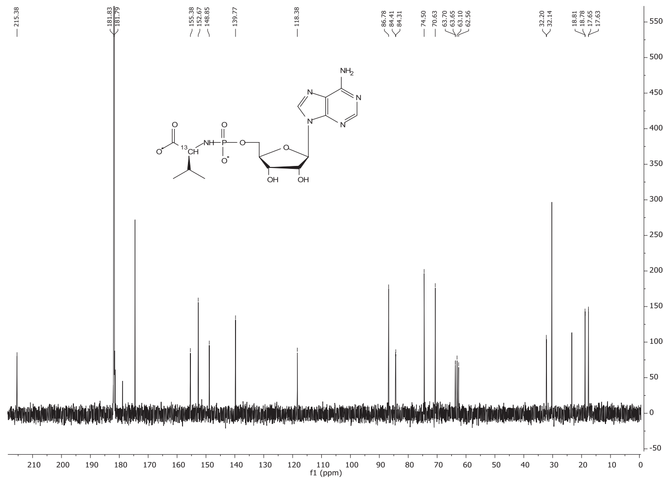
^{13}\text{C} NMR spectrum ( \text{H}_2\text{O} , 100 MHz) of Val*A.
