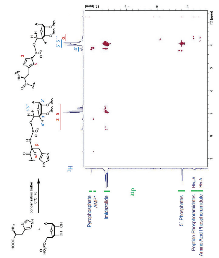
Figure 2.16 The growing use of ^1\text{H} - ^{31}\text{P} HMBC to attribute ^{31}\text{P} peaks in complex mixtures. Left: attribution of many product classes in a general condensation reaction. Reproduced from the SI of the original manuscript 61 under Creative Commons License. Right: determination of the regio- and chemoselectivity of a phosphorylation reaction. Reproduced from the SI of the original manuscript 61 under Creative Commons License.
