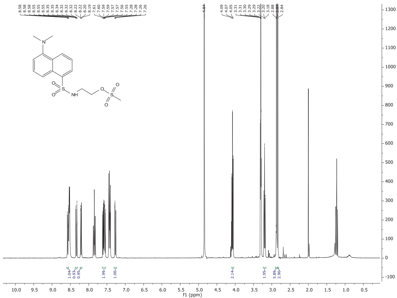
^1\text{H} NMR (MeOD, 300 MHz) of (30) showing traces of EtOAc and pyridine that were deduced from the yield.
