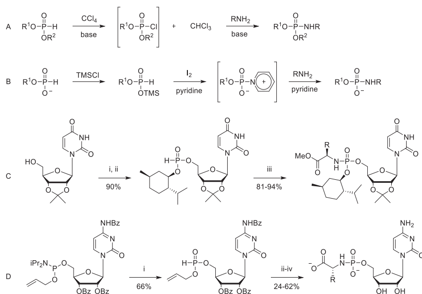
Scheme 2.39 Atherton-Todd inspired strategies to prepare phosphoramidates and phosphoramidates. A: the classical Atherton-Todd reaction. B: a variation used in the synthesis of phosphoramidate analogues of nucleotides. C: Synthesis of uridine phosphoramidates through an Atherton-Todd coupling. i: \text{PCl}_3 10 eq, \text{Et}_3\text{N} , \text{CH}_2\text{Cl}_2 , 0^\circ\text{C} , 3h. ii: menthol 1 eq, t\text{BuOH} 1 eq, \text{Et}_3\text{N} 2 eq, \text{CH}_2\text{Cl}_2 , 10 min. iii: amino acid methyl ester 1.3 eq, \text{Et}_3\text{N} , \text{CCl}_4 , water, \text{CH}_3\text{CN} , rt, 10 min. D: synthesis of cytidine phosphoramidates through an Atherton-Todd coupling. i: water, tetrazole, \text{CH}_3\text{CN} , rt. ii: amino acid methyl ester, \text{CCl}_4 , \text{Et}_3\text{N} , \text{CH}_2\text{Cl}_2 , rt. iii: \text{Pd}(\text{PPh}_3)_4 , \text{PPh}_3 , morpholine, \text{CH}_2\text{Cl}_2 , rt. iv: \text{MeONa} , \text{MeOH} , \text{NaOH} , rt.
