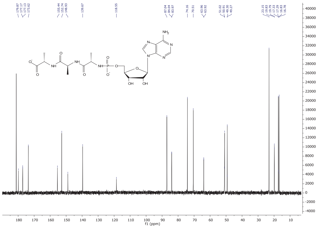
^{13}\text{C} NMR spectrum ( \text{D}_2\text{O} , 125 MHz) of Ala 3 A
