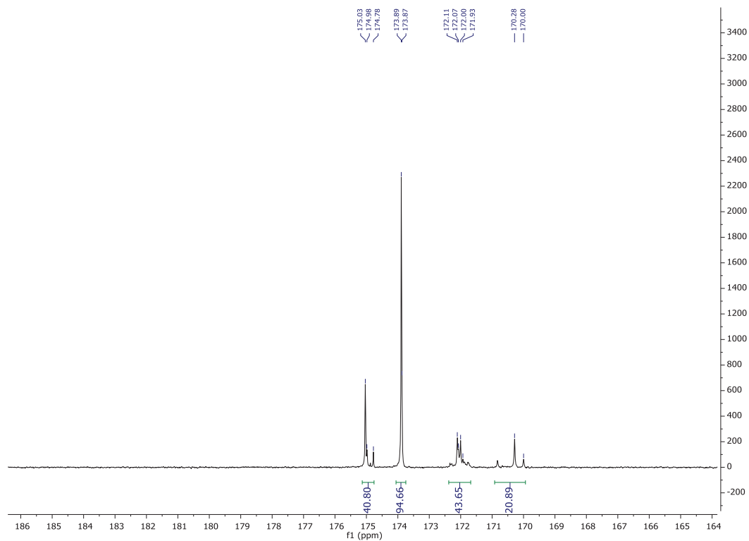
Figure S24 ^{13}\text{C} NMR ( \text{H}_2\text{O} , 100 MHz) for an assay involving saturated butanol and 200 mM 1\text{-}^{13}\text{C} glycine in MES buffer at pH 6. The butyl ester peak was not detected.
