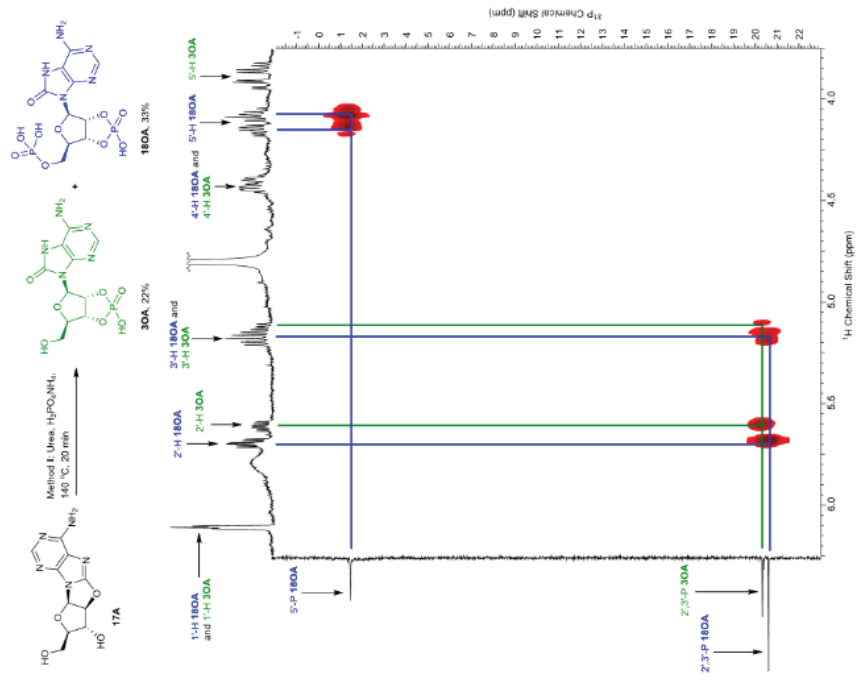
Figure 2.16 The growing use of ^1\text{H} - ^{31}\text{P} HMBC to attribute ^{31}\text{P} peaks in complex mixtures. Left: attribution of many product classes in a general condensation reaction. Reproduced from the SI of the original manuscript 61 under Creative Commons License. Right: determination of the regio- and chemoselectivity of a phosphorylation reaction. Reproduced from the SI of the original manuscript 61 under Creative Commons License.
