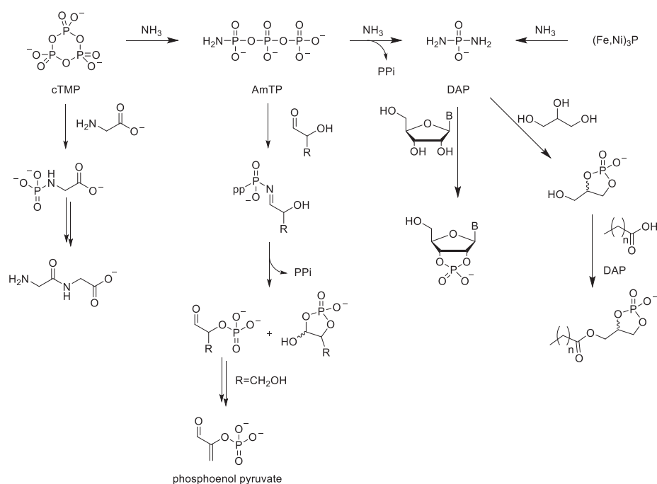
Scheme 2.17 Prebiotic phosphorylations with polyphosphates and amidophosphates.
