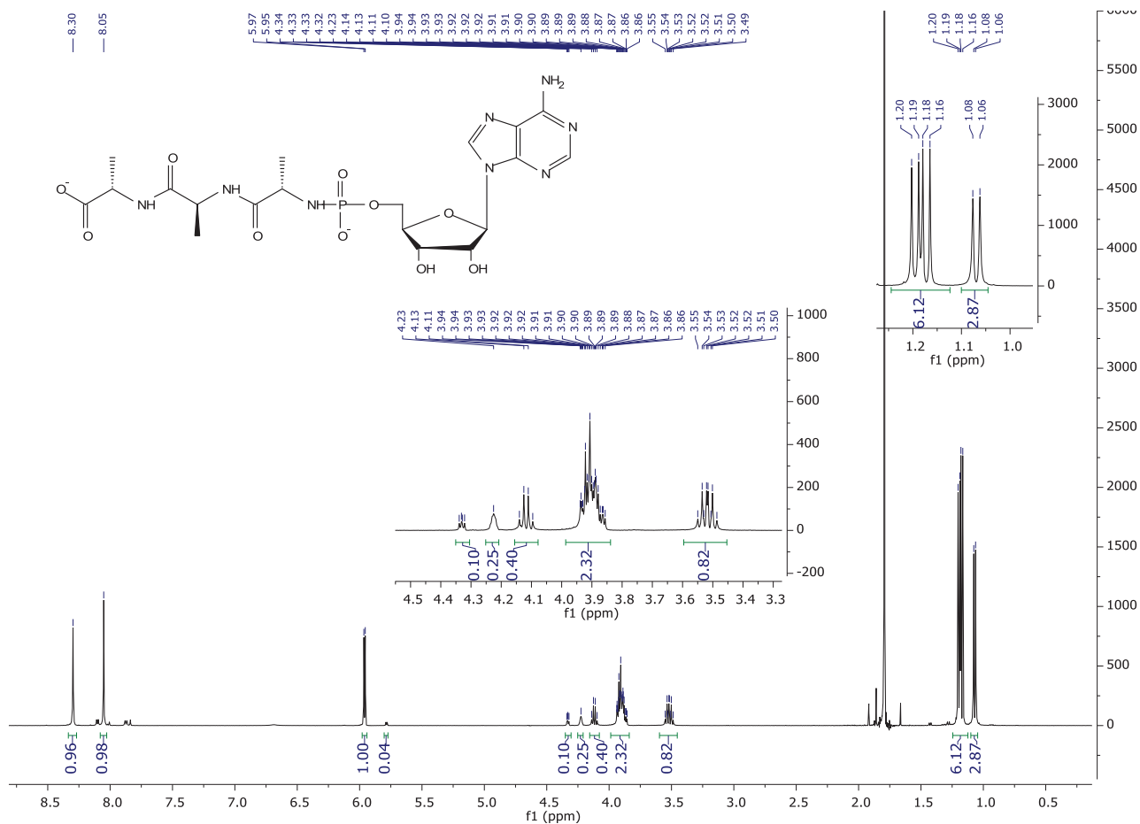
^1\text{H} NMR spectrum ( \text{D}_2\text{O} , 500 MHz) of Ala 3 A
