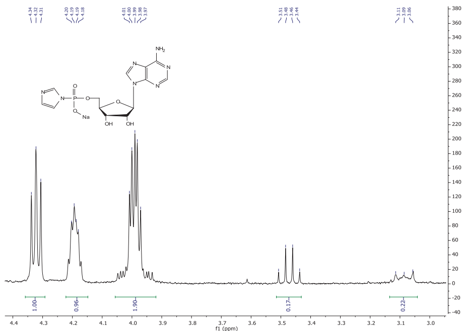
Figure S2 Enlarged view of the ^1\text{H} NMR of ImpA (300 MHz, \text{D}_2\text{O} ) showing the residual signals for triethylamine (3.47 ppm, integral = 0.17 for 6H, 2.8 mol%) and tetrabutylammonium (3.09 ppm, integral = 0.22 for 8H, 2.7%), confirming that the exchange to the sodium salt by precipitation is efficient.
