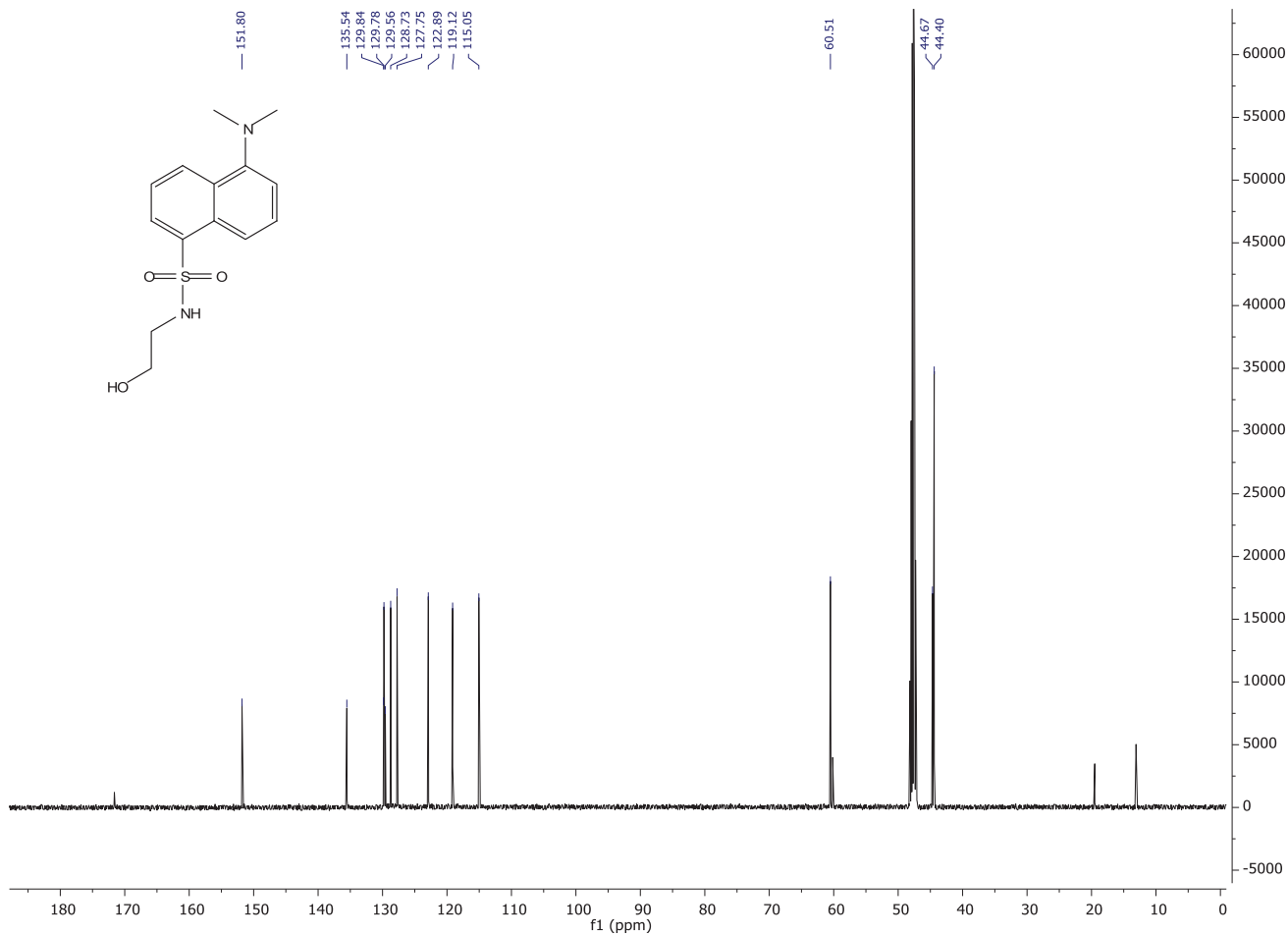
^{13}\text{C} NMR spectrum (MeOD, 125 MHz) of compound (29)
