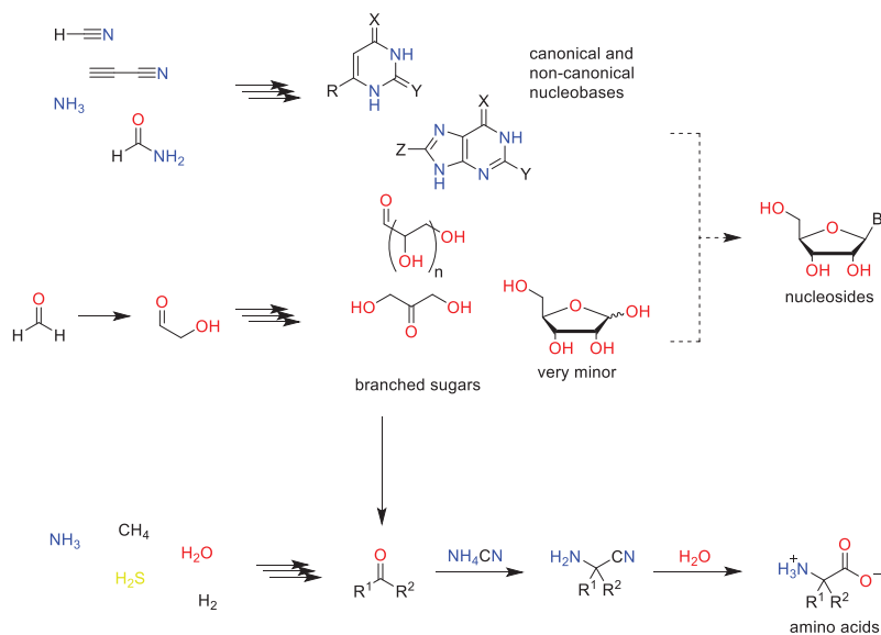
Scheme 2.2 Overview of the classical prebiotic syntheses of nucleosides, carbohydrates and amino acids. The limited interactions between the different domains (nitrogenous and oxygenous chemistry) highlight the lack of chemical compatibility between the routes.
