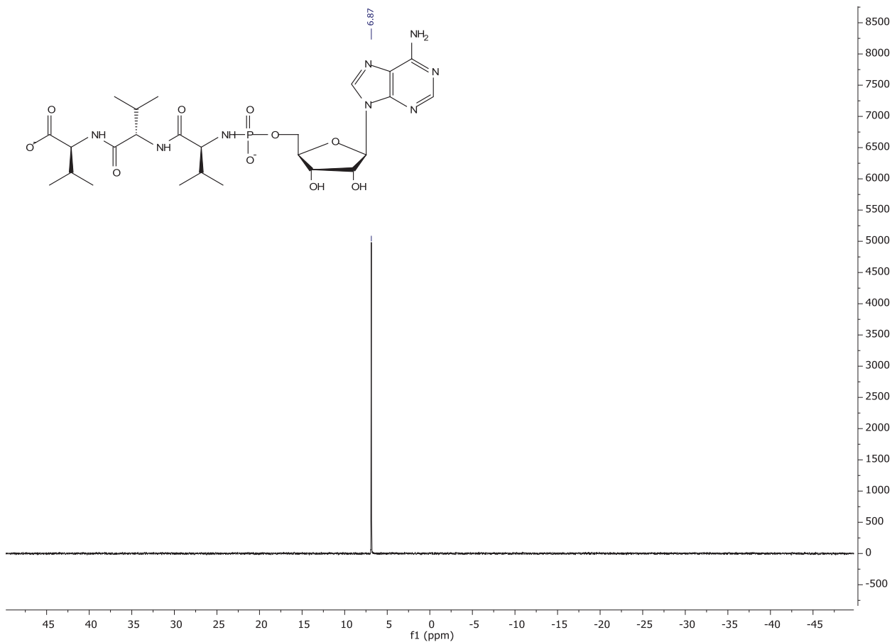
31 P NMR spectrum (H 2 O, 200 MHz) of Val 3 A.
