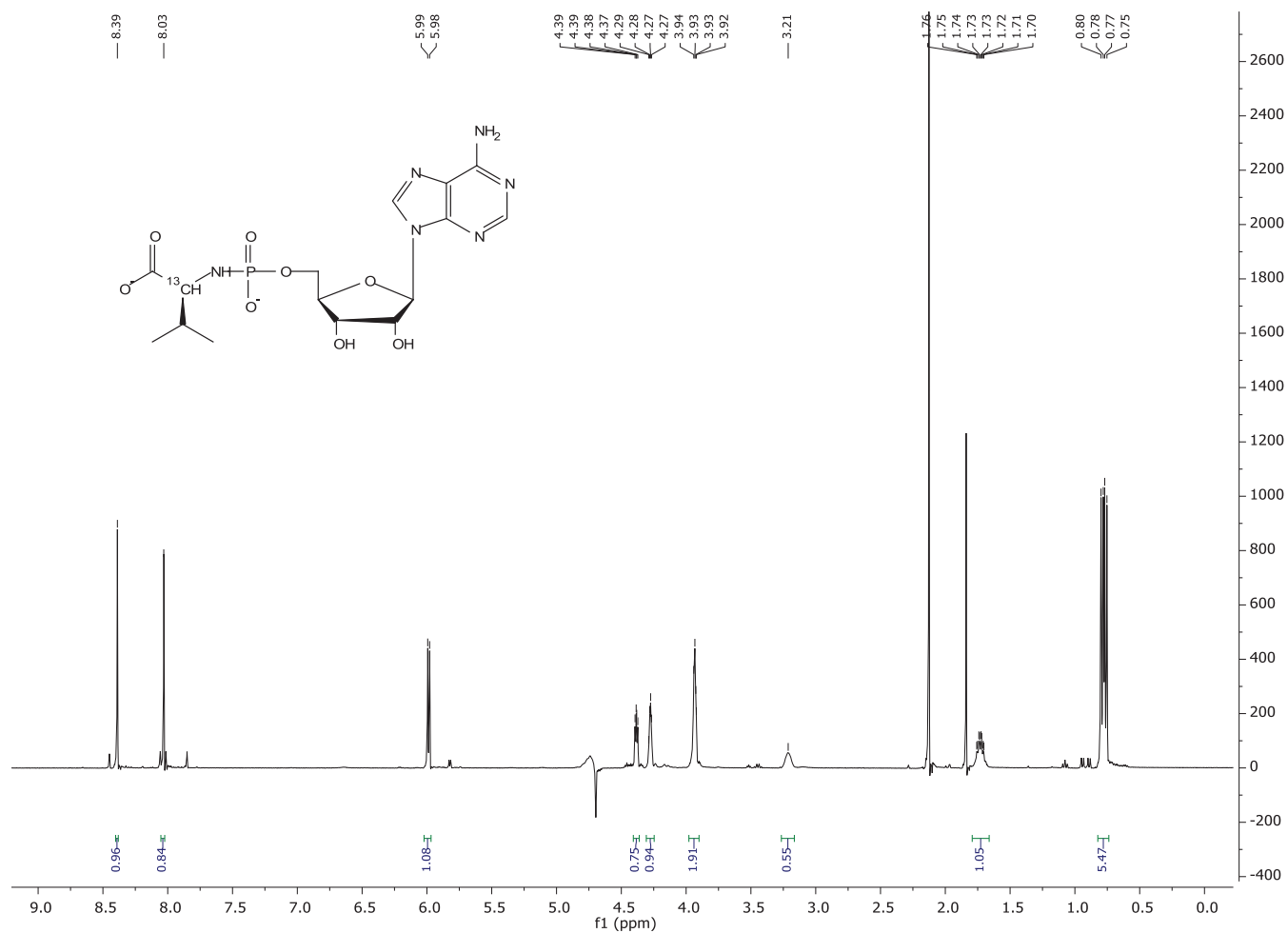
^1\text{H} NMR spectrum ( \text{H}_2\text{O} , 400 MHz) of Val*A. The presaturation sequence impacted the integration of the neighboring peaks.
