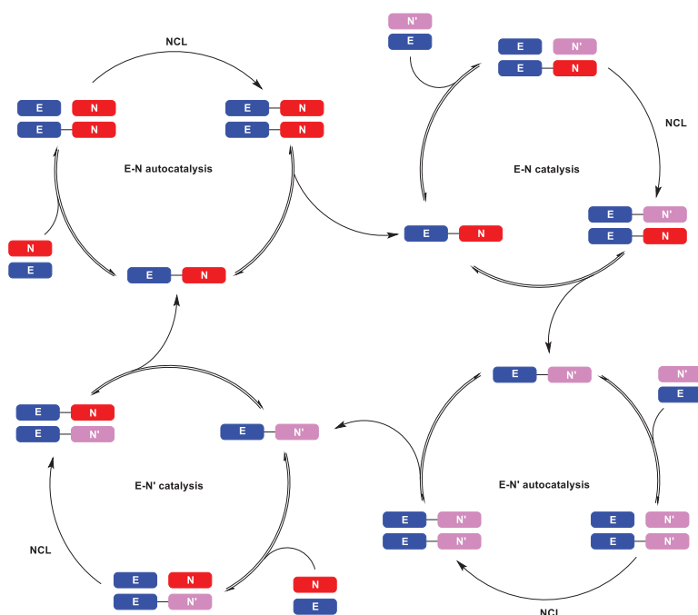
Scheme 2.24 Autocatalytic production of E-N and E-N' were interconnected by the cross-catalytic production of E-N catalyzed by E-N' and reciprocally, in a proto-symbiotic network.
