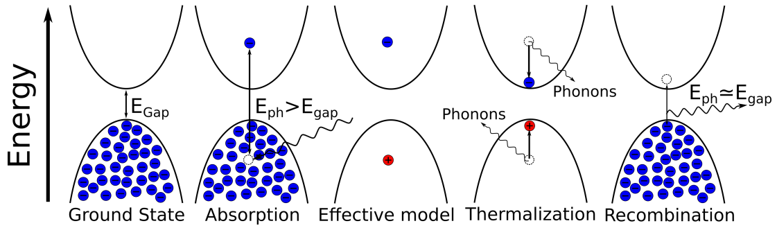
Figure 1.3: Different solar cell process as seen from a an energetic point of view. In the ground state, the valence band at the bottom contains the electrons (in blue), and the conduction band is empty. The forbidden region between the band is the semiconductor bandgap. Through absorption of a photon of greater energy than this gap, an electron can jump into the conduction band, and leaves a hole at it's original position. Because electrons are not discernible particles, we only need to follow the behaviour of the hole left behind by the electron, and not that of all the electrons in the valence band. The problem becomes a two particles problem, with one negative electron in the conduction band, and one hole in the valence band. These particles then cool down to the band edges, via emission of phonon, during the thermalization process, and can eventually undergo recombination.
