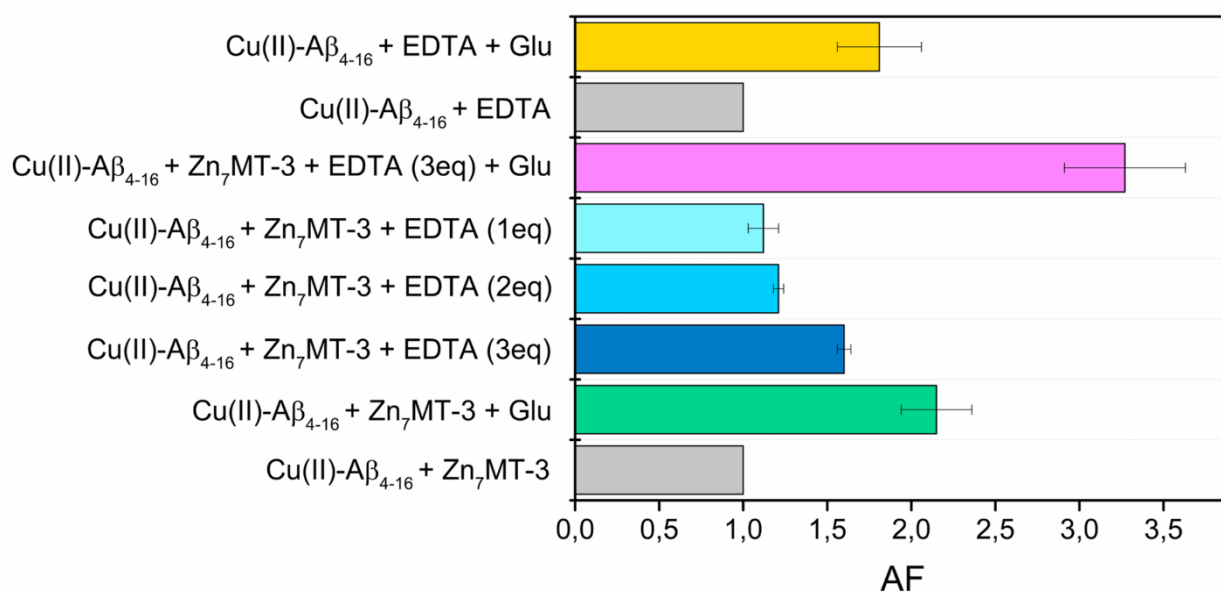
Fig 19 - Acceleration factors (AFs) calculated with respect to the reactions Cu(II)-A \beta_{4-16} + Zn(II) 7 -MT-3 (in case of the reactions in the presence of Zn(II) 7 -MT-3) and Cu(II)-A \beta_{4-16} + EDTA (for the reaction Cu(II)-A \beta_{4-16} + EDTA + Glu). AFs are reported with the corresponding standard deviation error (reactions performed in triplicate).
