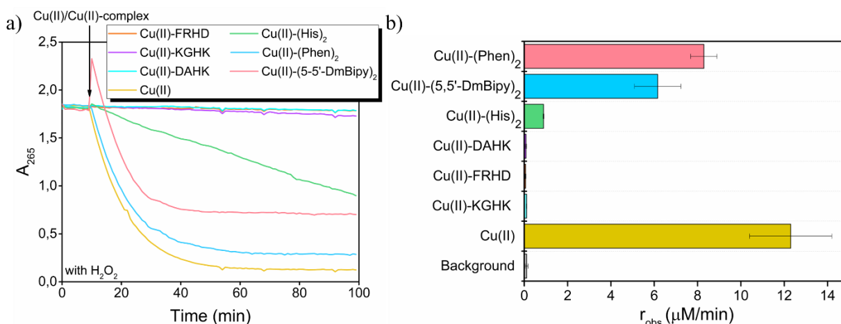
Fig 28 - a) Time course of AscH - oxidation: evolution of the AscH - absorption ( \lambda_{\max} = 265 nm) as a function of time, after exposure to Cu(II), Cu(II)-XZH, Cu(II)-(His) 2 , Cu(II)-(5,5'-DmBipy) 2 , and Cu(II)-(Phen) 2 complexes, with H 2 O 2 . AscH - oxidation was started by the addition of free Cu(II) or the preformed Cu(II)-complex after 10 min. Experimental conditions: Cu(II) 10 μM, XZH peptide/ligand 12 μM/24 μM, AscH - and H 2 O 2 100 μM, in PB 50 mM, pH 7.4. b) Histogram of the corresponding molar AscH - oxidation rates (μM/min). Measurements were performed in triplicate, with different solutions at different days, thus average values of r_{\text{obs}} (μM/min) with standard deviations have been calculated.
