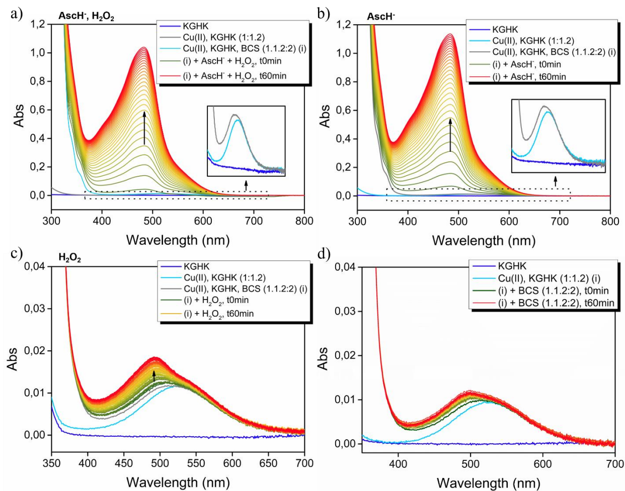
FigS 15 - Uv-Vis spectra for the reaction of Cu(II)-KGHK (ratio 1:1.2, Cu(II):KGHK) with a) \text{AsCH}^- and \text{H}_2\text{O}_2 , b) \text{AsCH}^- , c) \text{H}_2\text{O}_2 , d) blank (i.e. with no \text{AsCH}^- and/or \text{H}_2\text{O}_2 ) in the presence of BCS. Experimental conditions: Cu(II) 100 \mu\text{M} , KGHK 1200 \mu\text{M} , \text{AsCH}^- and \text{H}_2\text{O}_2 10 mM, BCS 200 \mu\text{M} , in PB 50 mM, pH 7.4. Reactions were monitored over 1h, collecting intermediate spectra at 2 min intervals.
