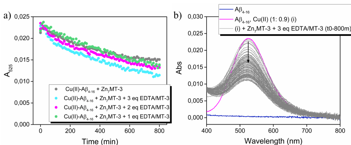
Fig 21 - a) Time course of Cu(II) release from Cu(II)-A \beta 4-16 to Zn(II) 7 -MT-3 (grey profile), Zn(II) 4 -MT-3 (cyan profile), Zn(II) 5 -MT-3 (purple profile), Zn(II) 6 -MT-3 (green profile) monitored by absorbance spectroscopy at \lambda_{\text{max}} = 525 nm. 3, 2 and 1 eq of EDTA/MT-3 were respectively added together with Zn(II) 7 -MT-3 to the preformed Cu(II)-A \beta 4-16 complex to generate the desired partially Zn(II)-loaded species. b) Source of UV-Vis spectra for the reaction of Cu(II)-A \beta 4-16 with Zn(II) 7 -MT-3 and 3 eq EDTA/MT-3. Reactions conditions: A \beta 4-16 250 \mu M, Cu(II) 225 \mu M, Zn(II) 7 -MT-3 50 \mu M (ratio A \beta 4-16 /Cu(II)/Zn(II) 7 -MT-3, 1:0.9:0.2), EDTA 150 \mu M (3 eq/MT-3)/EDTA 100 \mu M (2 eq/MT-3)/EDTA 50 \mu M (1 eq/MT-3), PB 50 mM, pH 7.4.
