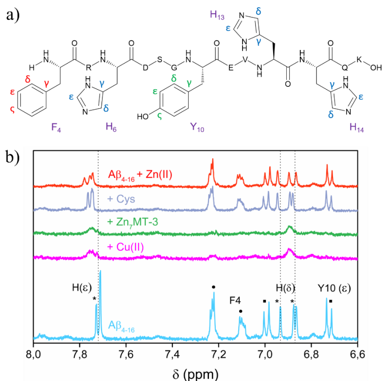
Fig 15 - a) A \beta 4-16 peptide sequence (FRHDSGYEVHHQK-NH 2 ) with the aromatic amino-acid residues nomenclature. b) 1 H-NMR displaying the Zn(II) binding to A \beta 4-16 . Aromatic region of the spectrum of A \beta 4-16 (light blue line) and after the addition of (i) Cu(II) (purple line), (ii) Zn(II) 7 -MT-3 (green line), (iii) Cys (grey line); control of A \beta 4-16 after the direct addition of 0.6 eq. of Zn(II) (red line). Reaction conditions: A \beta 4-16 300 \mu M, Cu(II) 270 \mu M, Zn(II) 7 -MT-3 60 \mu M, Cys 3 mM (ratio A \beta 4-16 /Cu(II)/Zn(II) 7 -MT-3, 1:0.9:0.2). Spectra were obtained from 10% D 2 O/90% H 2 O solutions in PB 50 mM, pH 7.4, at \nu = 400MHz.
