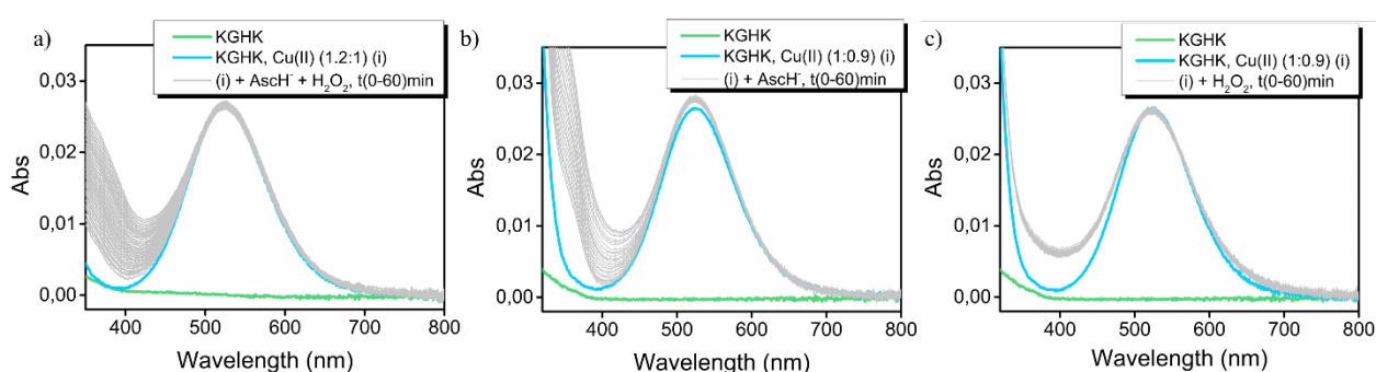
Fig 29 - UV-Vis spectra for the reaction of Cu(II)-KGHK (ratio 1:1.2, Cu(II):KGHK) with a) AscH - and H 2 O 2 , b) AscH - and c) H 2 O 2 . Reaction conditions: Cu(II) 250 \mu M, KGHK 300 \mu M, AscH - and H 2 O 2 5 mM, in PB 50 mM, pH 7.4.
