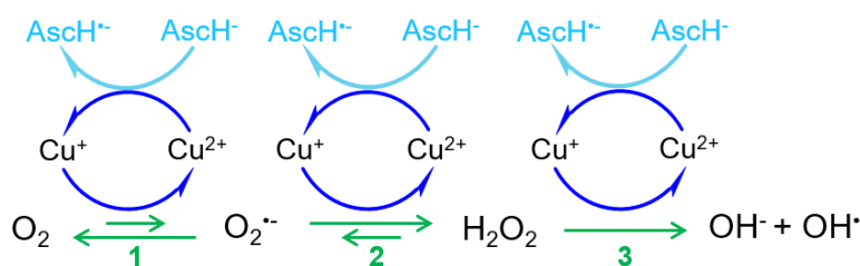
Fig 2 - Mechanism of Cu-catalyzed ROS production in the presence of \text{O}_2 and a reducing agent like \text{AscH}^- . The electron flow goes from \text{AscH}^- to the \text{O}_2 species, catalyzed by Cu.
