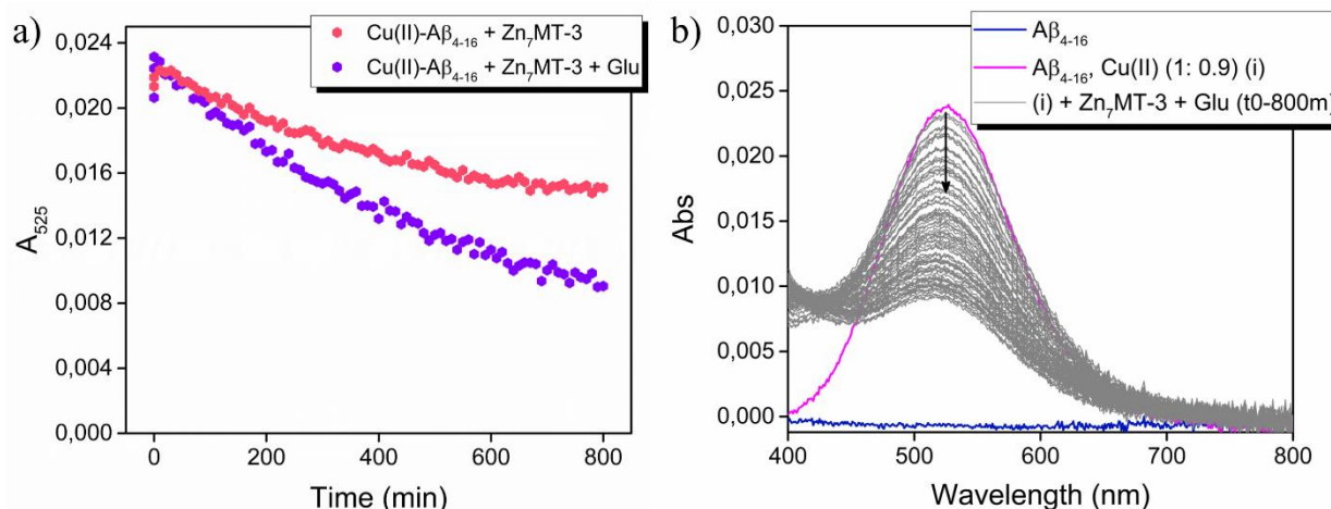
Fig 16 - a) Time course of Cu(II) release from Cu(II)-A \beta 4-16 to Zn(II) 7 MT-3 in the presence and absence of Glu in the reaction mixture, monitored by absorbance spectroscopy at \lambda_{\text{max}} = 525 nm. b) Source of UV-Vis spectra for the reaction of Cu(II)-A \beta 4-16 with Zn(II) 7 MT-3 and Glu, added together at t(0m) to the preformed Cu(II)-A \beta 4-16 complex (purple profile). Reactions conditions: A \beta 4-16 250 \mu M, Cu(II) 225 \mu M, EDTA 150 \mu M, \pm Glu 5 mM, PB 50 mM, pH 7.4.
