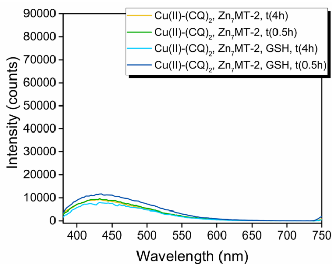
FigS 34 - a) Low-temperature luminescence spectra obtained after the addition of Zn(II) 7 -MT-1 with or without GSH to the preformed Cu(II)-(CQ) 2 complex. Experimental conditions: 10 \mu M Cu(II)-CQ (ratio 1:2), 2.5 \mu M Zn(II) 7 -MT-1 (ratio Cu-complex: Zn(II) 7 -MT-1, 1:0.25), 3 mM GSH in HEPES 50 mM, pH 7.4.
