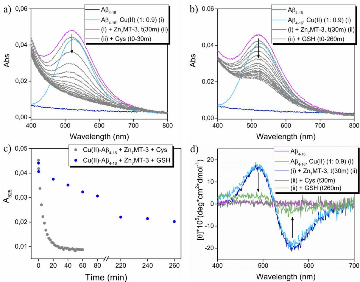
Fig 13 - Evidence of Cu(II) reduction and release from Cu(II)-Aβ 4-16 in the presence of Zn(II) 7 -MT-3. In a) and b) absorption spectroscopy for the reaction with Cys and GSH respectively is shown. Each intermediate spectrum was collected at 2 min intervals in a) and at 10 min intervals in b). c) Corresponding kinetics for the two reactions with Cys and GSH: absorbance at λ max = 525 nm versus time. d) Circular dichroism (Vis-region, 400-700 nm) for the reaction with Cys (grey profile) and GSH (green profile). Reaction conditions for Uv-Vis and CD experiments: Aβ 4-16 500 μM, Cu(II) 450 μM, Zn(II) 7 -MT-3100 μM (ratio Aβ 4-16 /Cu(II)/Zn(II) 7 -MT-3, 1:0.9:0.2), a) Cys 3 mM, b) GSH 3 mM, PB 50 mM, pH 7.4.
