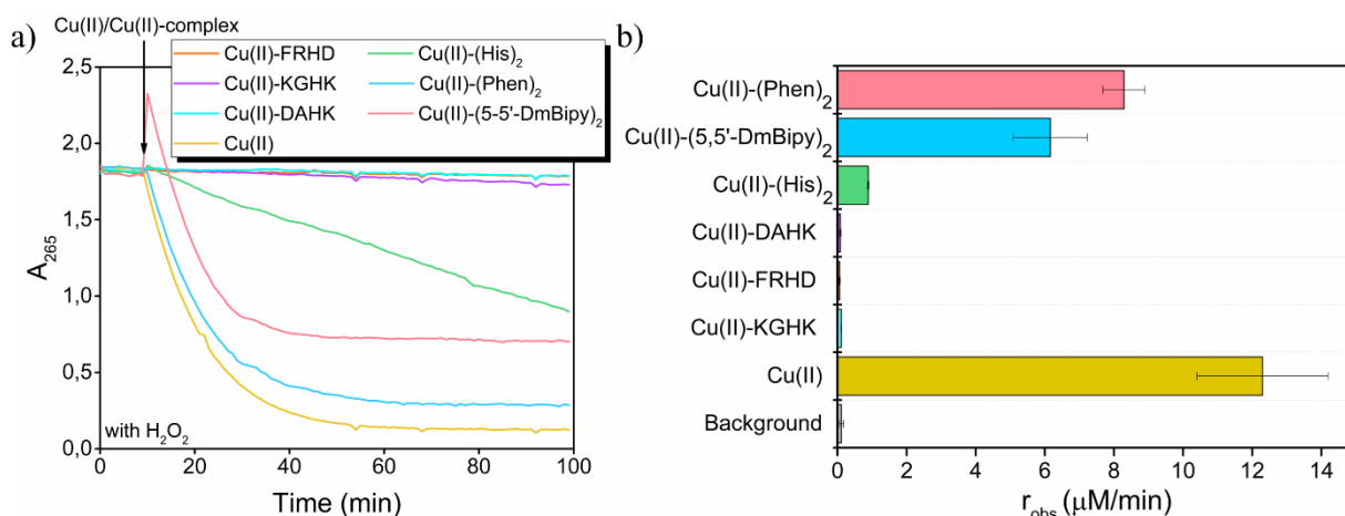
Fig 28 - a) Time course of AsCH - oxidation: evolution of the AsCH - absorption ( \lambda_{max} = 265 nm) as a function of time, after exposure to Cu(II), Cu(II)-XZH, Cu(II)-(His) 2 , Cu(II)-(5,5'-DmBipy) 2 , and Cu(II)-(Phen) 2 complexes, with H 2 O 2 . AsCH - oxidation was started by the addition of free Cu(II) or the preformed Cu(II)-complex after 10 min. Experimental conditions: Cu(II) 10 μM, XZH peptide/ligand 12 μM/24 μM, AsCH - and H 2 O 2 100 μM, in PB 50 mM, pH 7.4. b) Histogram of the corresponding molar AsCH - oxidation rates (μM/min). Measurements were performed in triplicate, with different solutions at different days, thus average values of r_{obs} (μM/min) with standard deviations have been calculated.
