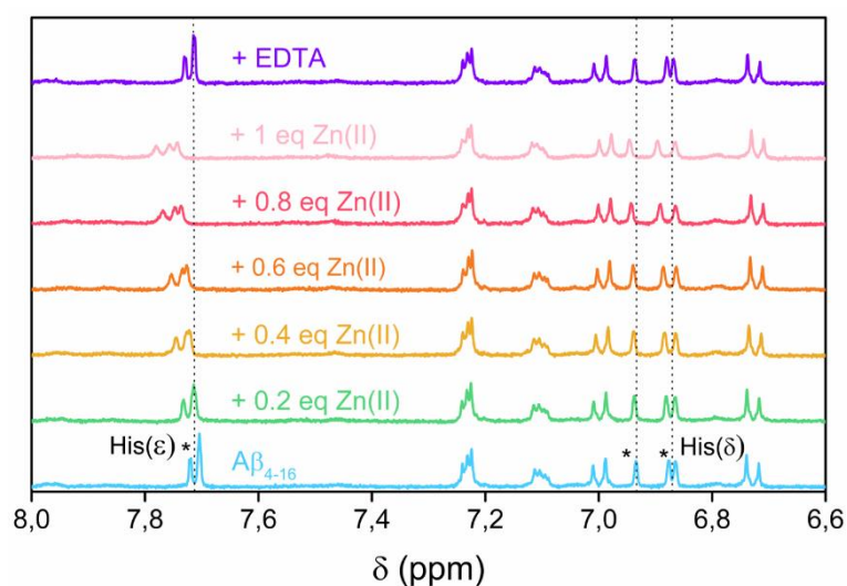
FigS 3 - Zn(II) titration of A \beta_{4-16} peptide followed by ^1\text{H} -NMR, through the aromatic region of the spectra, and addition of EDTA to the 1:1 complex Zn(II)-A \beta_{4-16} (violet profile). Experimental conditions: a 300 \mu\text{M} A \beta_{4-16} solution (600 \mu\text{l} ) was titrated with 2 \mu\text{l} aliquots of a 36 mM stock solution of Zn(II) (0.2 eq Zn(II)/A \beta_{4-16} ); to the 1:1 complex Zn(II)-A \beta_{4-16} (light pink profile) a concentrated solution of EDTA (50 mM, pH 7.4) was added to reach the final concentration of 300 \mu\text{M} .
