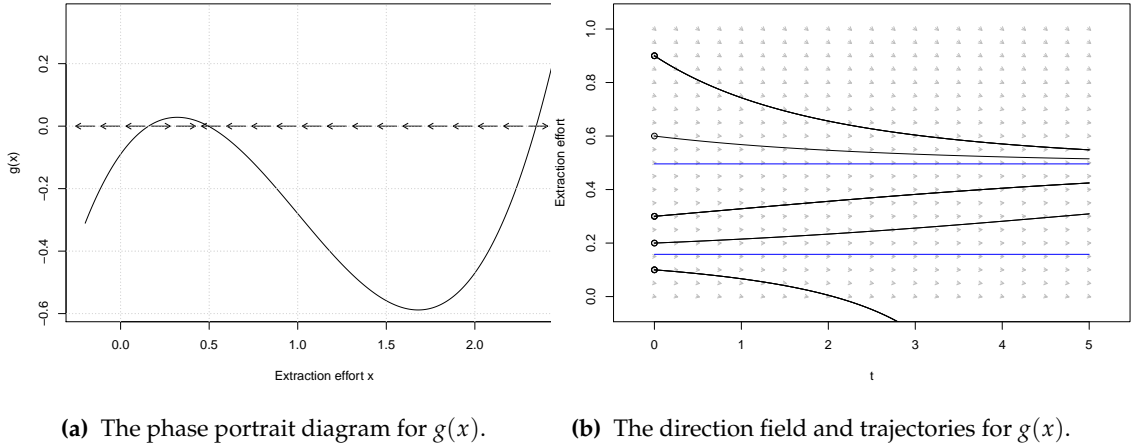
Figure 3.3: Phase diagram and trajectories for g(x) .
