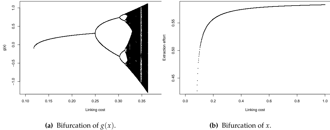
Figure 3.5: Bifurcation diagram of g(x) and extraction effort x with different \nu .
