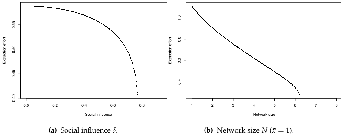
Figure 3.6: Bifurcation diagram of x with different \delta and N .
