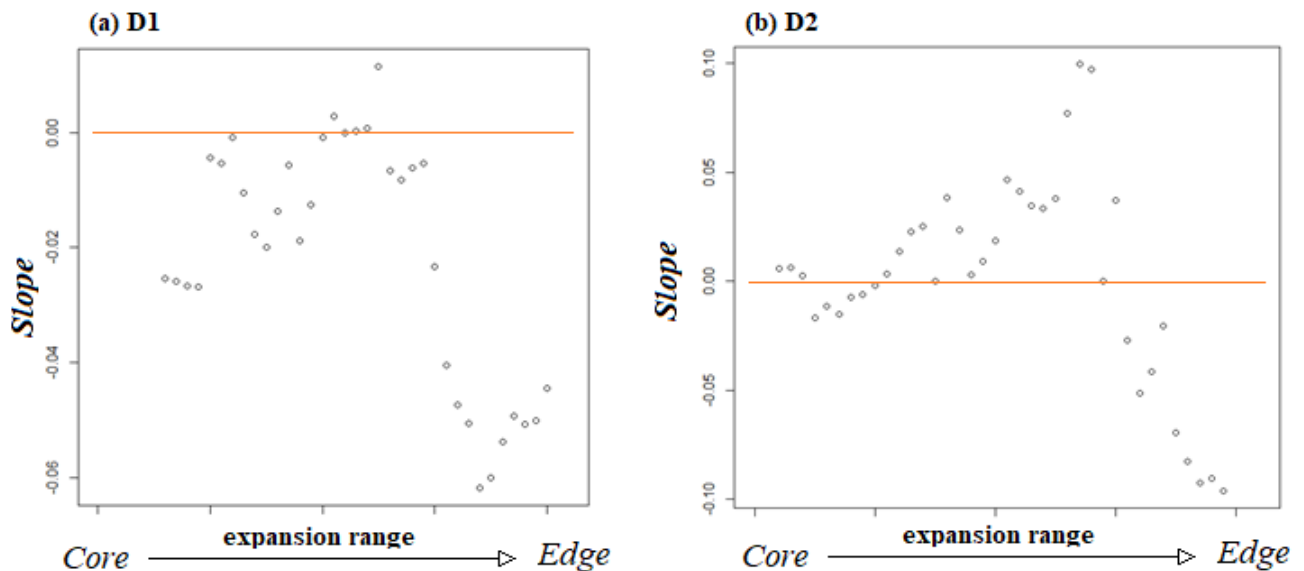
Figure 5.10: Evolution of the relationship between body size and time (slope) along the colonization front, on D1 (a) and D2 (b).
