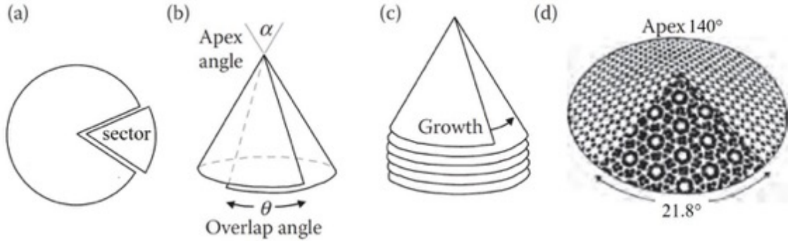
Figure 7: Sketch of the cone-helix mode: (a) from removing a sector with an angle noted \theta_{\text{sector}} from a graphene disc, (b-c) the cone is formed by an overlapping of the graphene layer. (d) the overlapping angle noted \theta_{\text{overlap}} will impact the apex angle of the cone noted \alpha . modified from [27Dimovski2017] and [34Double1974].
