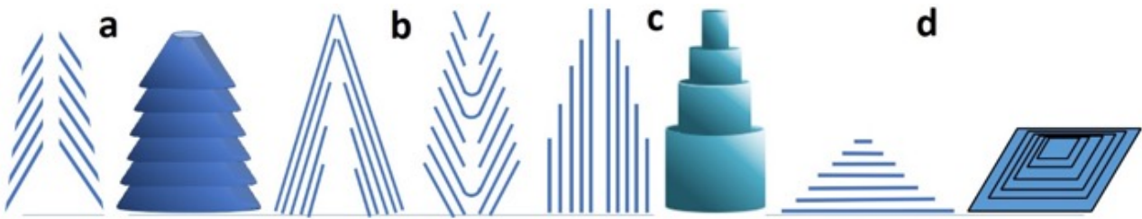
Figure 12: Sketch of the three ways to generate graphenic morphologies whose conical forms are driven by the texture, i.e., the orientation of the graphene layers with respect to the cone axis. (a) and (b) three different textures for graphene sheets oblique to the cone axis; (c) graphene sheets parallel to the cone axis; (d) graphene sheets perpendicular to the cone axis. The line-drawings aside the 3D models sketch the way the inner texture of overall conical morphologies may look like when seen as projected images such as obtained by HRTEM. Although the 3D models in (a), (c), (d) hypothesize a stack configuration, the projected textures would look the same in case of a cone-helix configuration.
