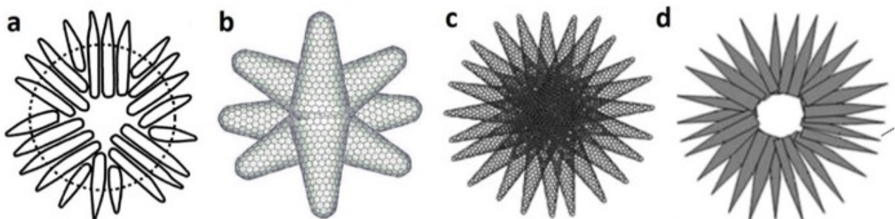
Figure 4: Various models from the literature proposed for a ball-like nanoparticle made from aggregated nanohorns such as that imaged in Fig.3 . (a) from [41Iijima1999]; (b) from [47Pagona2007]; (c) from NEC website; (d) From [48Shi2017].
