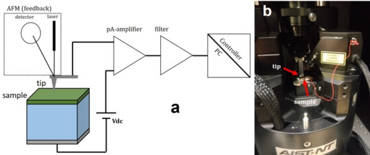
Figure 24: (a) Schematic of a C-AFM working principle in tapping mode. A bias voltage is applied from the sample to the tip or vice-versa. Then, the analogous current signal is converted into a digital voltage by using the amplifier and a filter. (b) The AIST-NT, SPM 1000 model AFM microscope used for our C-AFM tests. It is operated in tapping mode called point by point ( I top mode), allowing current from few pA to \mu A. The voltage applied for I/V curves can go from -8 to +8 V.
