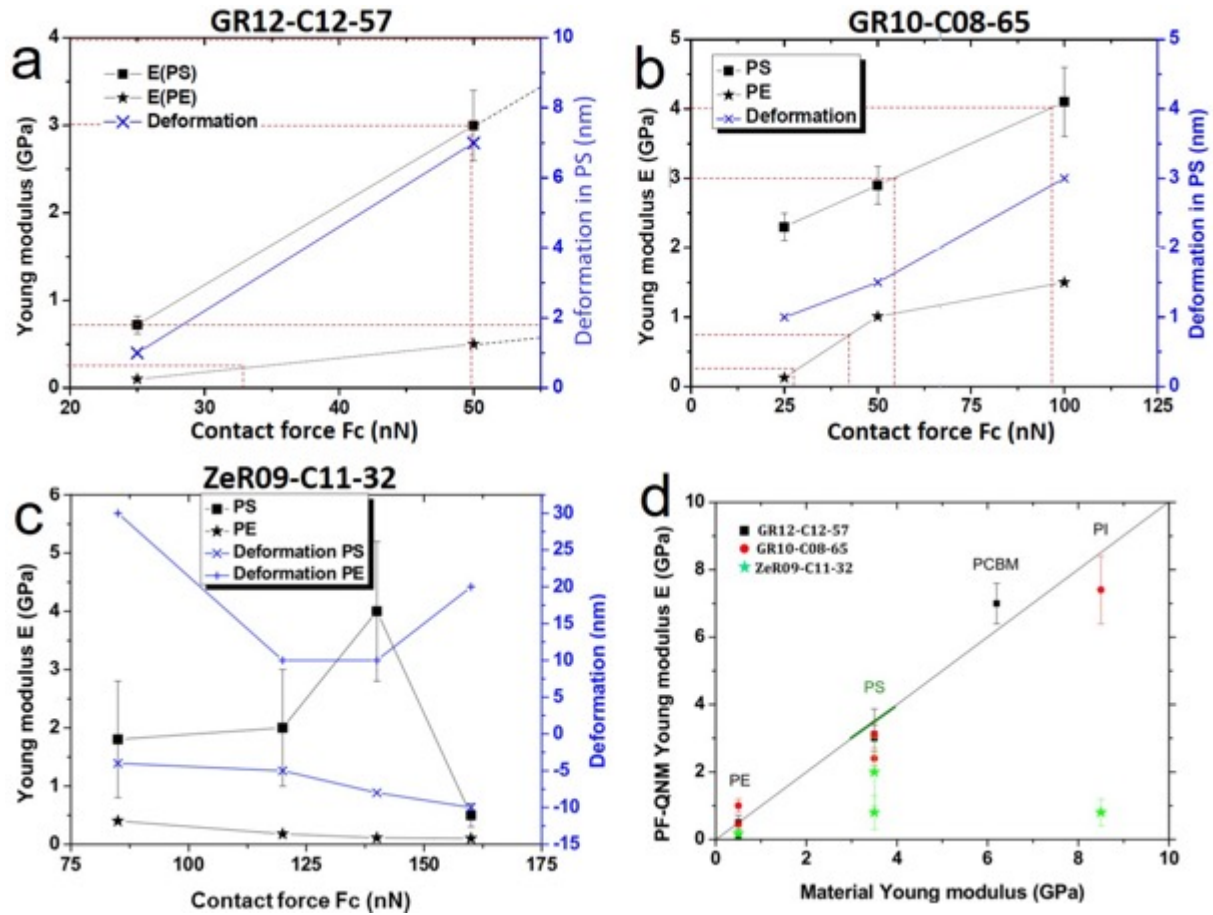
Figure22: (a) to (c) Young Modulus and polymer deformation variation with respect to the contact force F_c for each carbon probe. (d) represents the Young modulus values of different polymers determined with the nanocone probes through PFQNM compared with the theoretical values.
