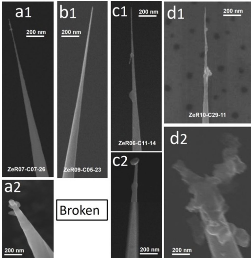
Figure 34: SEM images of the nanocone probes before (a1 to d1) and after (a2 to d2) the C-AFM tests. From the apex radius of the tips after test, it is estimated that the probe ZeR07-C07-26 was shortened by 800 nm, the probe ZeR06-C11-14 was shortened by 1 \mu\text{m} , and the probe ZeR10-C29-11 was shortened by about 3 \mu\text{m} . (Photo credit: R. Cours, A. C. Torres-Dias, M. Kandara).
