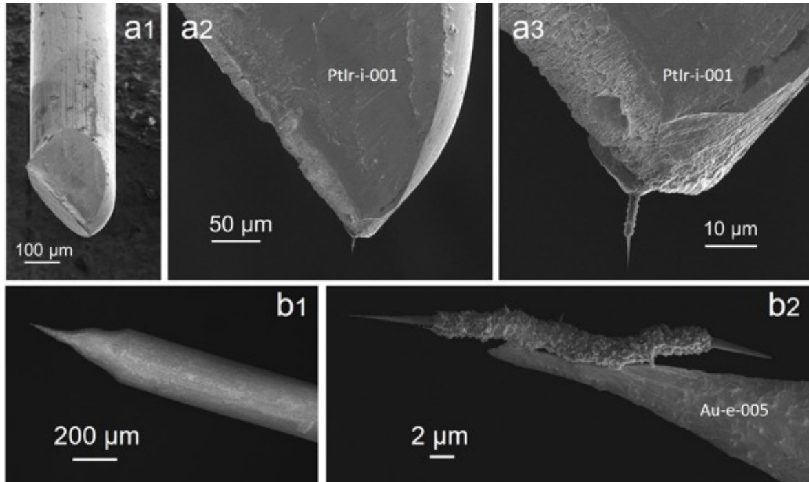
Figure 13. SEM images of SSF-based STM probes prepared following the same procedure as described by Fig.12 . (a) Welding with Pt by FIBID onto a mechanically cut Pt-Ir wire (Probe #PtIr-i-001). (b) Welding with W by FEBID onto an electrochemically tapered Au wire (Probe #Au-e-005).
