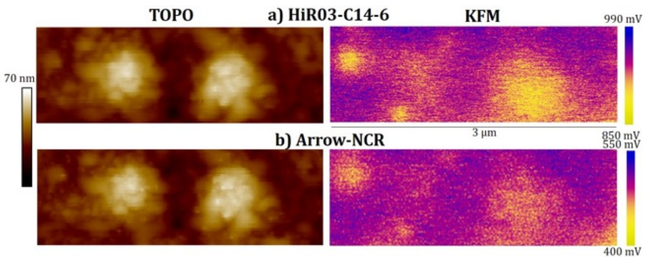
Figure 50: Higher magnification of the area framed in Fig.49 . Intermetallic particles in an aluminum alloy (A2024) matrix surface. Topography (left) and KFM (right) images for (a) the carbon nanocone probe HiR03-C14-6 ; (b) the reference Si probe.
