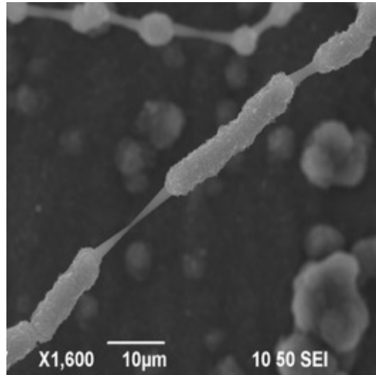
Figure 16: Example of the LGCF morphology formed as a secondary phase at position #10 in the experiment with a similar \text{CH}_4 as for Tab3b , but with a total flow rate in-between FLOW7 ( Tab 4d ) and FLOW8 ( Tab 4e ).
