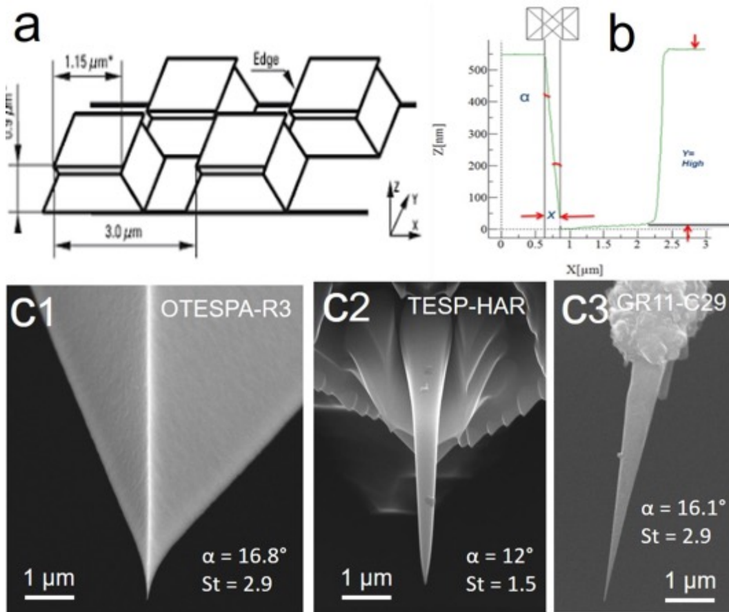
Figure 15: Methodology to obtain the apex angle of the probe tip from imaging a calibration substrate. (a) sketch of the calibration substrate used (TGX1 from NT-MDT). (b) measurements can be drawn from the AFM profile. (c) Examples of three AFM probes tested, and parameter values obtained from the AFM profiles of the calibration substrate ( \alpha = half apex angle. st = standard deviation). Considering the visual, it was expected that the geometric characteristics obtained for the carbon nanocone (c3) would be similar to that of the commercial TESP-HAR probe (c2), but it appeared to be similar to that of a commercial, standard probe (c1) instead.
