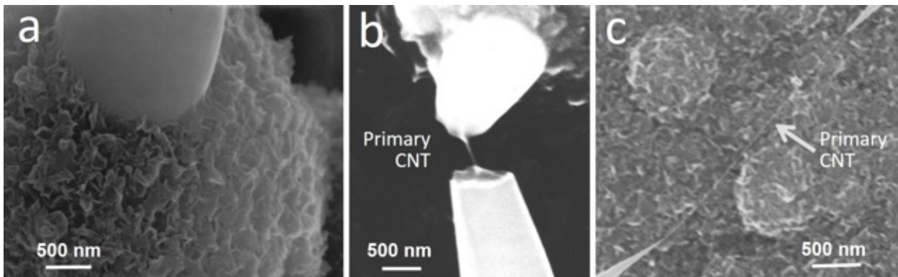
Figure 4: Scanning electron microscopy image of cone-related sub-morphologies. (a) The bead (rough surface) cone (smooth surface) interface showing that the former overlaps the latter. (b) Evidence for the presence of a primary CNT as the axial core of the cone sub-morphology, made visible upon the incidental breaking of a cone-to-cone junction. (c) From the presence of the primary carbon nanotube joining two opposed cones from two different aligned SBs (out of the picture frame), it is also demonstrated that the cones grow onto the CNT. From [21Allouche2005].
