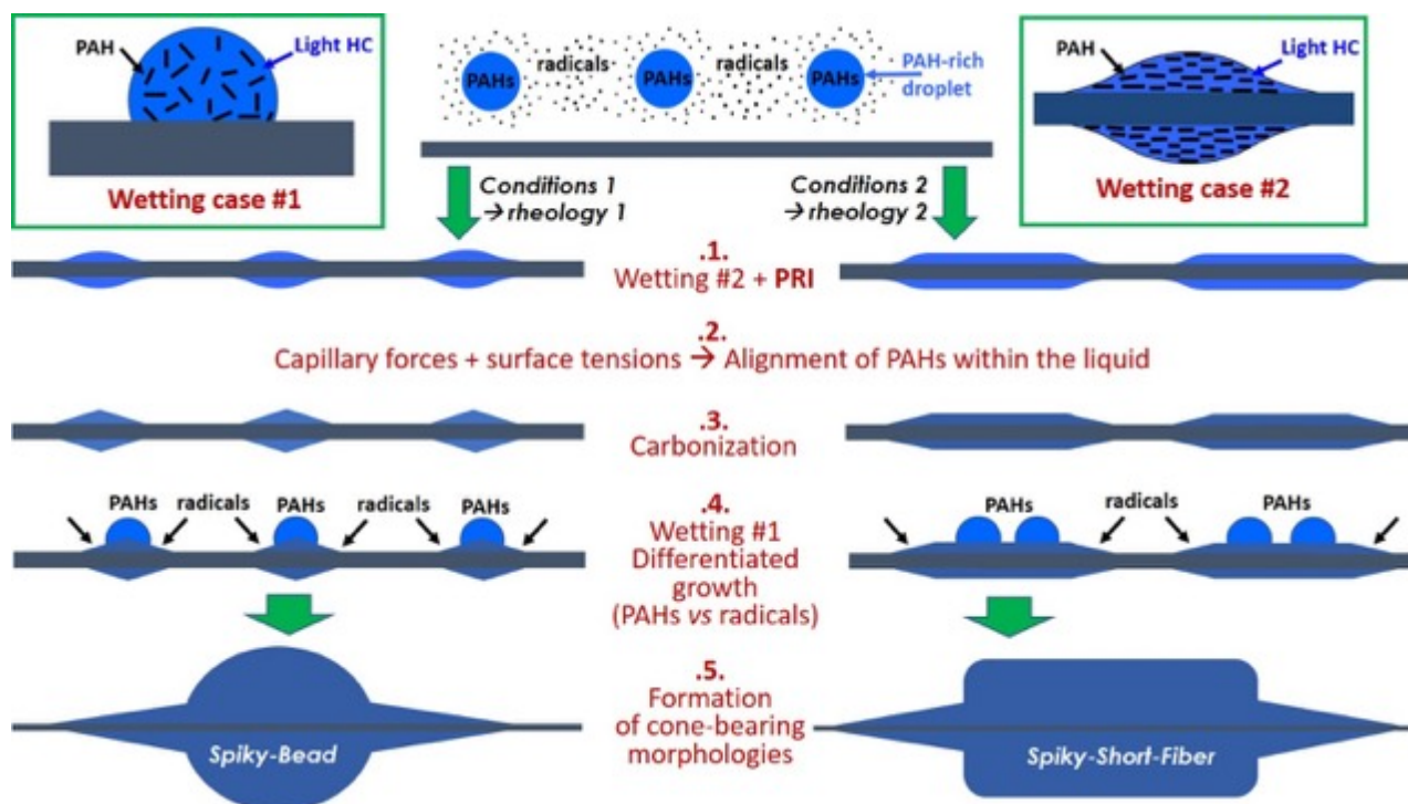
Figure 19: Sketch of a possible scenario accounting for the various morphologies formed as illustrated in Fig.2 . The two wetting cases refer to Figs.10 and 17a . The sketches focus on the formation of SB (left) and SSF (right) morphologies, but starting from closer "droplets" at step 1 would result in the PNBf (left), and LGCF (right) morphologies. Finally, starting from even closer droplets would result in the BF morphology.
