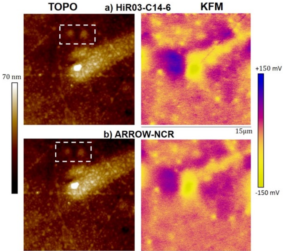
Figure 49: Intermetallic particles in an aluminum alloy (A2024) matrix surface. Topography (left) and KFM (right) images for (a) the carbon nanocone probe HiR03-C14-6 ; (b) the reference Si probe.
