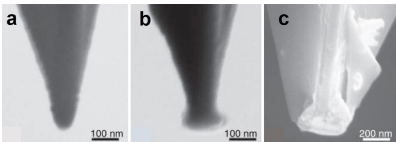
Figure 25: SEM images showing the evolution of a metal-coated tip (CoCr): (a) Before conducting any C-AFM test. (b) After at least 10 scans and I-V measurements. (c) Example of a worn and damaged tip [23Benstetter2017].
