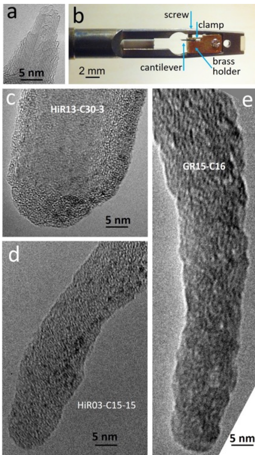
Figure 20. (a) HRTEM image of the apex of an as-synthesized carbon cone, for comparison with images (c) to (e) at the same scale; an enlarged version is provided in Ch.2-Fig.22d . (b) Detail of the modified TEM holder used to investigate carbon cones when mounted as SPM probes. (c) to (e) Examples of HRTEM images of carbon probe apices when mounted: (c) and (d) using the FIBID process in the HELIOS SEM-FIB; dark spots in both images are assumed to be gallium atoms or clusters, preferably to Pt or W (the welding materials); (e) using the gluing process. Images in (a), (c), and (d) were taken with a FEI TITAN FEG-SACTEM operated at 80 kV (INA, Saragoza. Image credit: R. Arenal). Images in (d) and (e) were taken with a FEI TECNAI F20 FEG-SACTEM operated at 100kV (image credit: S. Joulié, CEMES).
