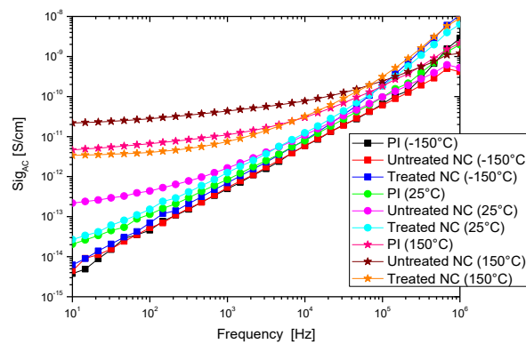
Figure 4-7. The frequency dependence of the AC conductivity for neat polyimide, untreated and silane-treated nanocomposites at -150 °C, 25 °C and 150 °C
