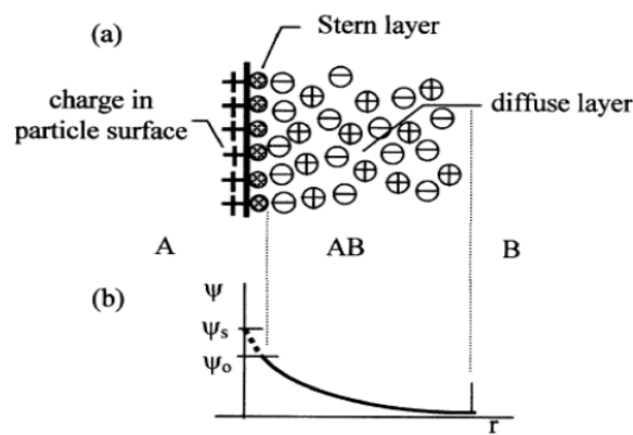
Figure 1-15. (a) The diffuse electrical double layer produced by a charged particle A in a matrix B containing mobile ions, and (b) the resulting electrical potential distribution \Psi(r)
