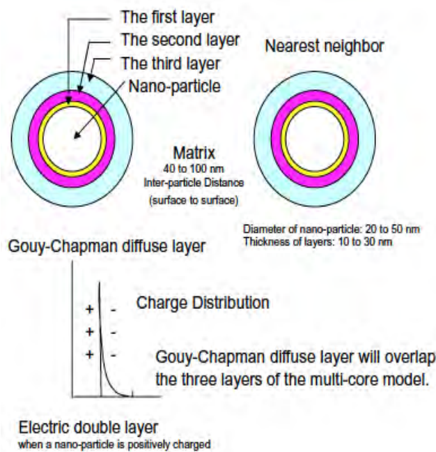
Figure 1-16. Multi-core model for nanoparticle / polymer interphase
