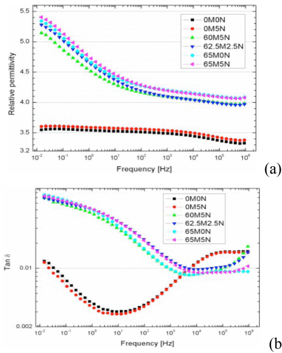
Figure 1-5. (a) Dielectric permittivity and (b) losses factor spectra at 60°C
