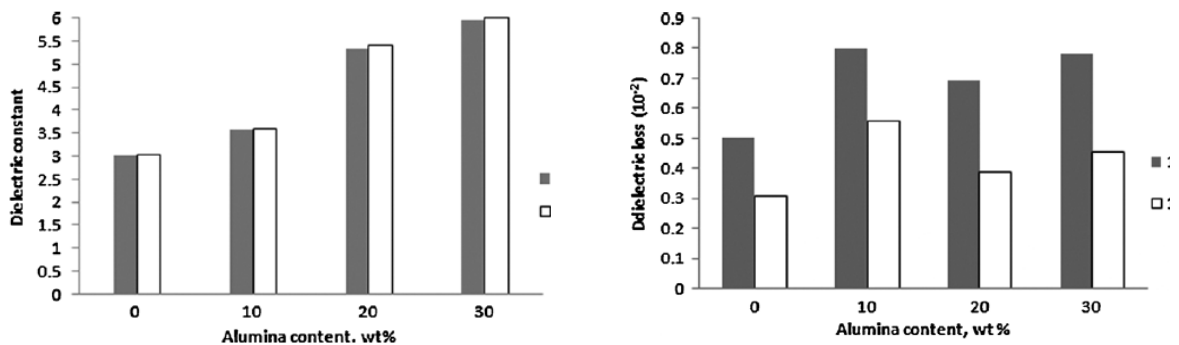
Figure 1-3. PI/ \text{Al}_2\text{O}_3 (0,5 \mu\text{m} ) Permittivity and loss factor
