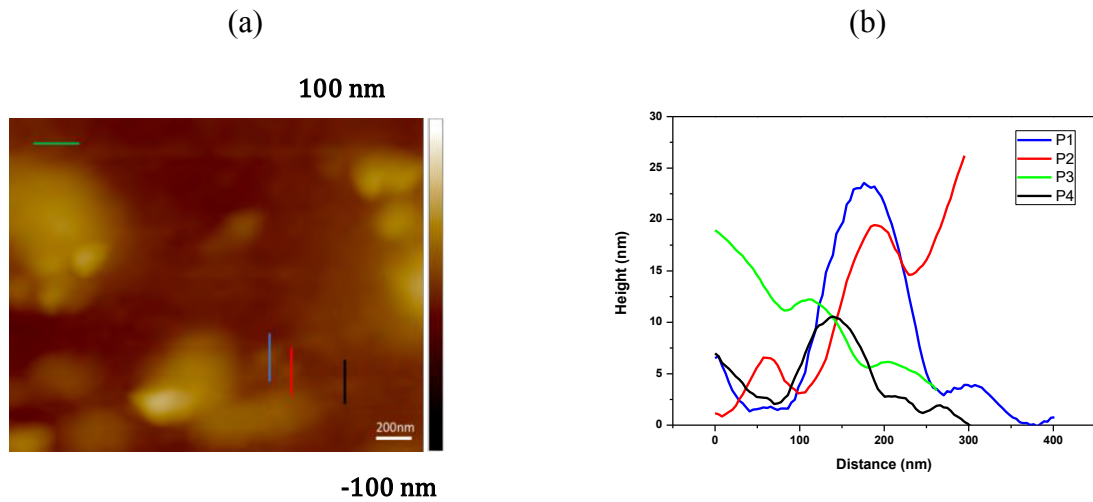
Figure 3-12. (a) AFM Topography image of treated NC scan size of 2\mu\text{m}^2 , (b) height particles profiles
