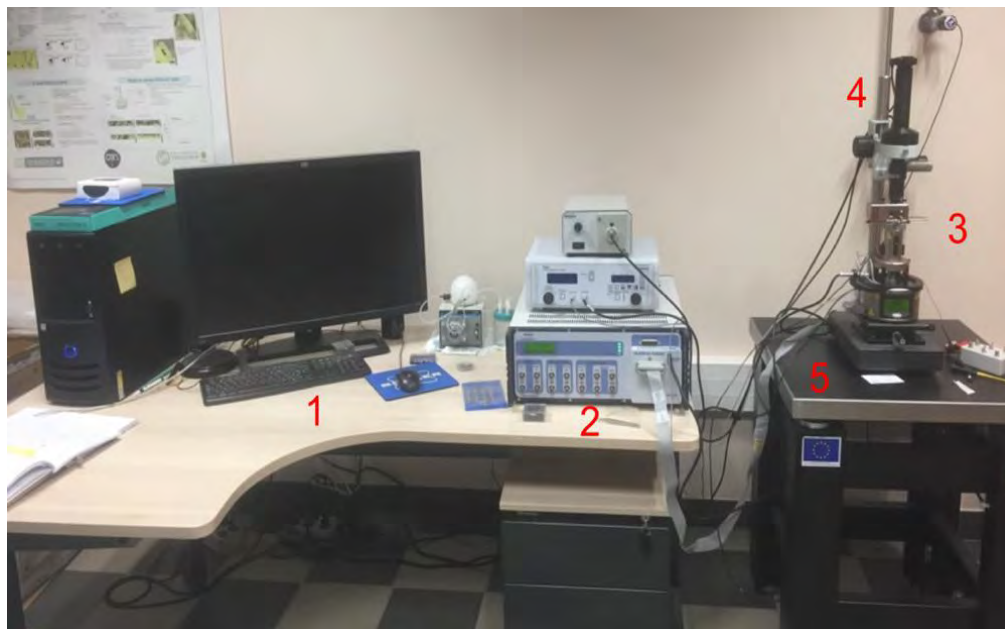
Figure 2-22. Bruker multimode8 complete hardware setup. 1: PC (monitor, CPU, keyboard and mouse), 2: Nanoscope V controller, 3: Multimode V8 Scanning Probe Microscope (SPM), 4: The OMV-UNIV optical viewing system (helps for aligning Multimode SPMs), 5: VT-102-2 which is an air table for vibration isolation to set the SPM on.
