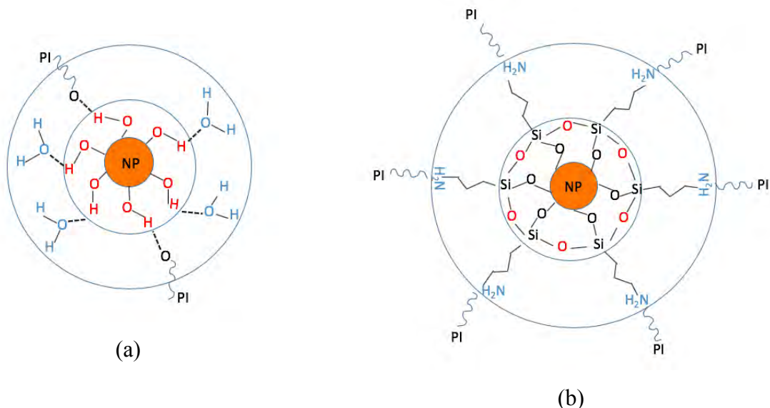
Figure 4-20. The effect of silane treatment on the interphase chemical treatment: (a) untreated particles and (b) treated particles (not to scale)
