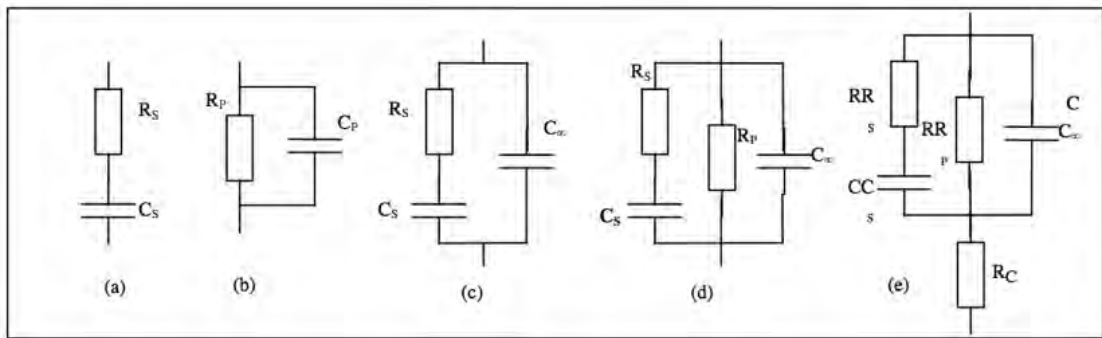
Figure 2-10. Equivalent electrical circuits of the dielectric behavior of an insulator. C_\infty is a capacity representing any other physical process independent of frequency
