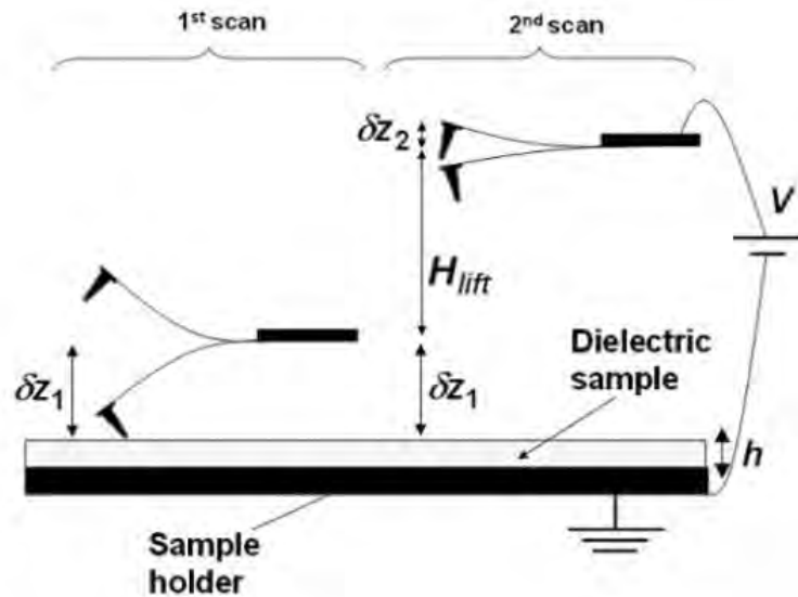
Figure 2-24. Principle of the double-pass method
