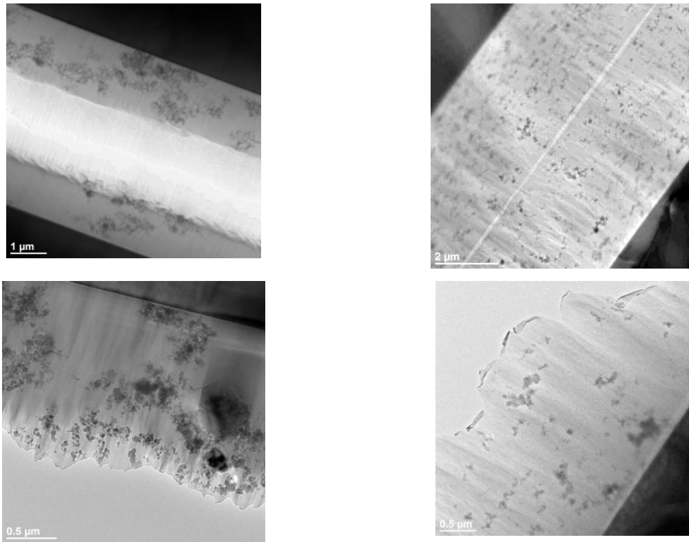
Figure 3-6. PI-nanocomposite TEM images for (left) untreated and (right) treated Si 3 N 4 nanoparticles
