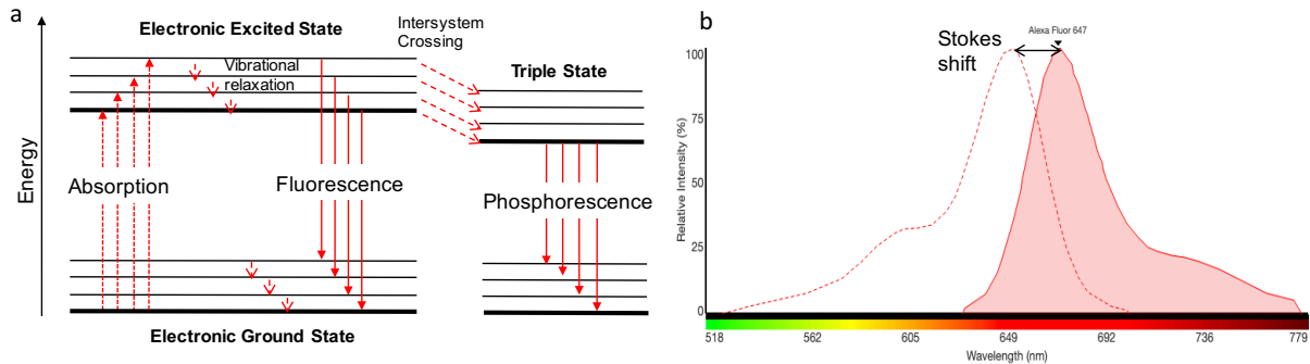
Figure 11. The Principle of fluorescence. (a) Jablonski Diagram representing the fluorescence timeline and the different energetic levels in which a molecule can transit through. (b) The excitation (dotted line) and emission (solid red line) spectra of the Alexa Fluor 647 dye. The loss of energy of a fluorescent molecule due to the vibrational relaxation and internal conversion results in a wavelength shift of the emission spectrum (the Stokes Shift).
