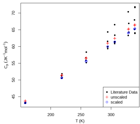
(j) propyne
