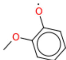
(c) Radical C_7H_7O_2^{\#}Z
