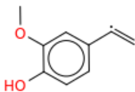
(g) 4 - Vinyl Guaiacol radical C_9H_9O_2^{\#}Z
