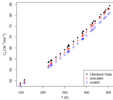
(i) propane
