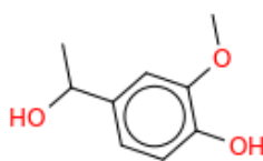
(b) 4 - (1 - Hydroxyethyl )-guaiacol C_9H_{12}O_3^{\#}Y
