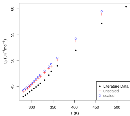
(a) methanol
