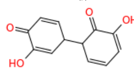
(l) Intermediate species S(280)
