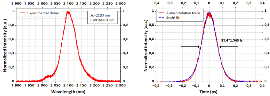
(a) Measured optical spectrum after a long-pass filter. (b) Autocorrelation trace.
