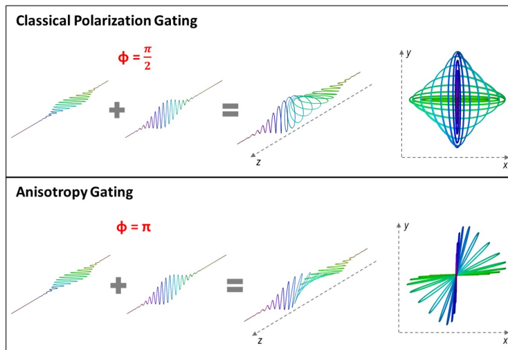
Figure 4.41: Illustration of the polarization gating and the anisotropy gating pulses.
