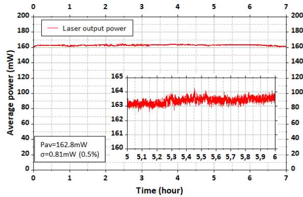
(c) Laser average power measured over a period of seven hours. Excellent stability corresponding to 0.5% rms.
