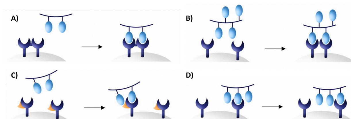
Figure 46 Different mechanisms of multivalent interaction A) chelate mechanism; B) clustering mechanism; C) chelate mechanism involving secondary site D) statistical re-association (adapted from Kiessling and co-workers, Curr Opin Chem Biol. , 2000). 176
