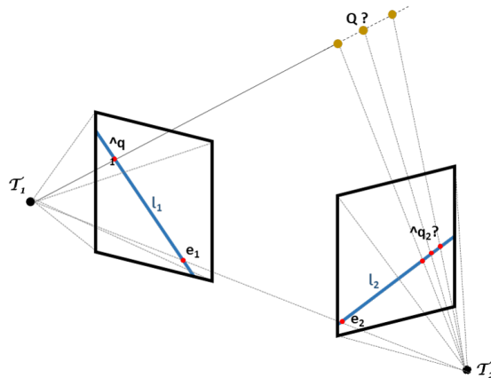
FIGURE B.1: Epipolar Geometry
