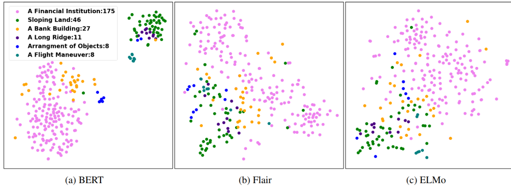
Figure 2.1 – T-SNE plots of contextualized embeddings of bank with their WordNet sense, with the frequency of each sense in the SensEval-3 training data, for 3 language models (Wiedemann, Remus, Chawla, & Biemann, 2019).
