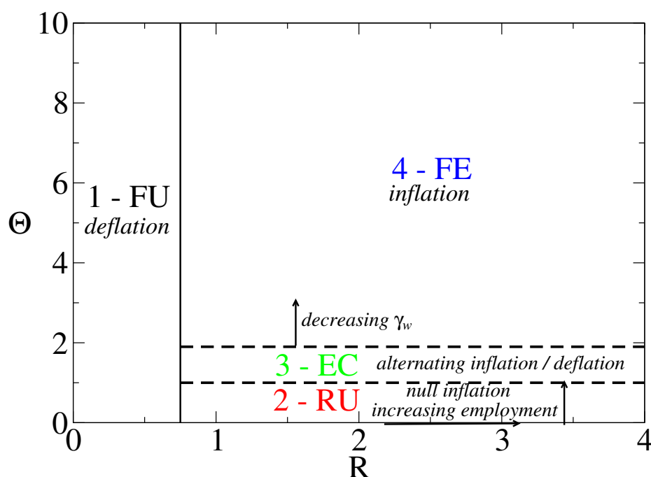
Figure 6.2: The phase diagram of the Mark-0 model is shown. Four distinct phases are identified. The Full Unemployment (FU) and Full Employment (FE) are accompanied by deflation and inflation respectively. The Residual unemployment (RU) phase has zero inflation but some unemployment remains. The Endogenous crises (EC) phase is marked by high employment (and inflation) on average punctuated by deflationary periods of high unemployment. Source [54].
