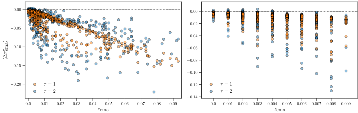
Figure 5.12: Variation of the change in the profits \pi_\mu^{\text{ema}} averaged over all remaining agents following the removal of an agent plotted against z_{\text{ema}} . Two distinct cases are shown, \tau = 1 and \tau = 2 corresponding to changes in the profit of surviving agents one time-step or two time-steps after the removal of agents. Left: \Delta \pi_{\text{ema}}^\mu against z_{\text{ema}} computed over the complete evolution of the economy. Right: Zoom of \Delta \pi_{\text{ema}}^\mu for small values of z_{\text{ema}} .
