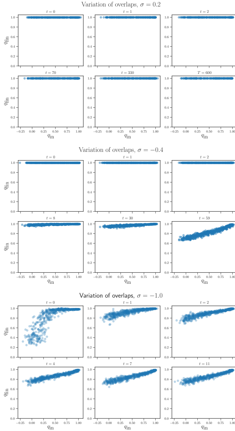
Figure 4.8: Variation of the final overlaps q_{fin} as a function of the initial overlap q_{in} , for \alpha = 20 , N = 200 , m = 0.577 . Overlap plots are shown for three distinct values of \sigma corresponding to different R&R and thermodynamic phases, as shown in Fig 4.7. \sigma = 0.2 is in the R&R-UNSAT (thermodynamically RS) phase whereas \sigma = -1.0 is in the R&R-SAT (thermodynamically RSB) phase. \sigma = -0.4 is an intermediate case: it is in the R&R-SAT, but thermodynamically RS, phase.
