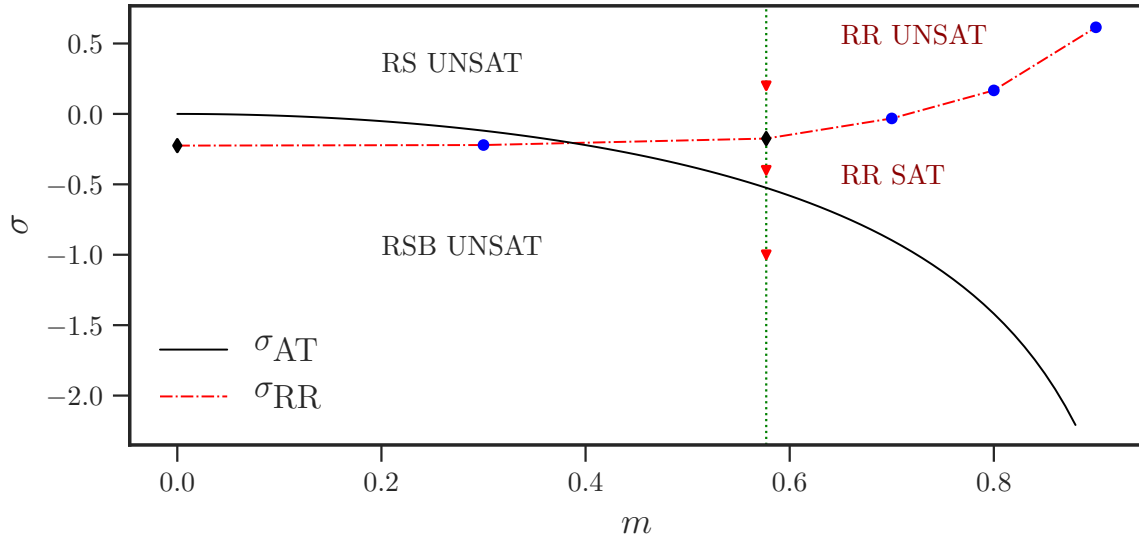
Figure 4.7: The full line is the de Almeida-Thouless transition \sigma_{AT} , below which replica symmetry is broken in the UNSAT phase (RSB UNSAT), obtained analytically for N \rightarrow \infty . Dots indicate the R&R algorithmic transition \sigma_{RR} , below which R&R dynamics converges to a self-planted state (R&R SAT), obtained numerically from the finite size scaling (diamonds, with four values of N as reported in Fig. 4.5; circles, with two values of N , not shown), for \alpha = 20 and as a function of m . The vertical dashed line and triangles indicate the points that are further investigated in Fig. 4.8.
