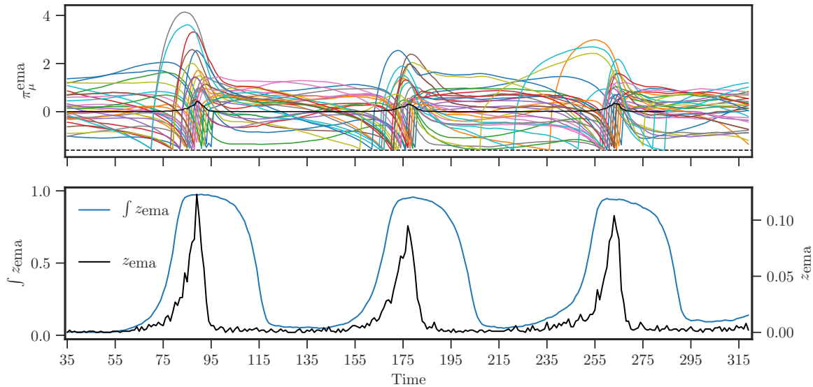
Figure 5.11: Top : \pi_{\mu}^{\text{ema}} time-series for \sigma = -1.6 is shown for 20 agents. The dark black line is the average value of \pi_{\mu} at which agents are re-injected. Bottom : z_{\text{ema}} (in black) with a moving integral of z_{\text{ema}} showing that during the crash almost all agents are removed and replaced.
