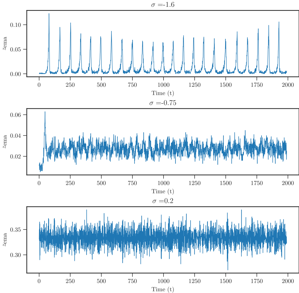
Figure 5.3: Variation of the fraction of unsatisfied agents z_{ema} as a function of time for three values of \sigma , in the EC (top), S (middle) and U (bottom) regimes. For \sigma = -1.6 , the agents are removed and replaced periodically whereas for \sigma = -0.75 , periodicity is lost. In the bottom panel, the \sigma = 0.2 case corresponding to high-profit is shown.
