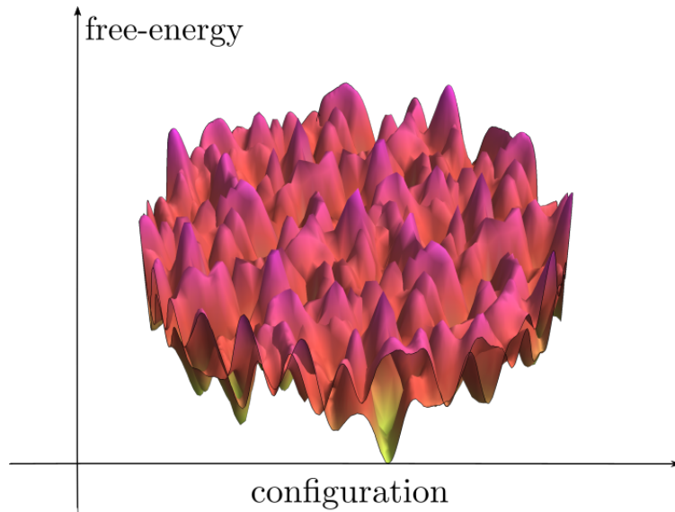
Figure 4.2: Schematic of the free-energy landscape of a system with Replica-symmetry breaking. The landscape has a large number of minimas separated by energy barriers with variable heights. The configuration axis represents a generic configuration, which itself is a higher-dimensional object.
