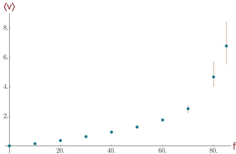
Figure 5.13: Velocity of the system v plotted versus prescribed load f . Bars indicate dispersion of velocity defined as the minimum and the maximum value of the set of n = 20 trajectories.
