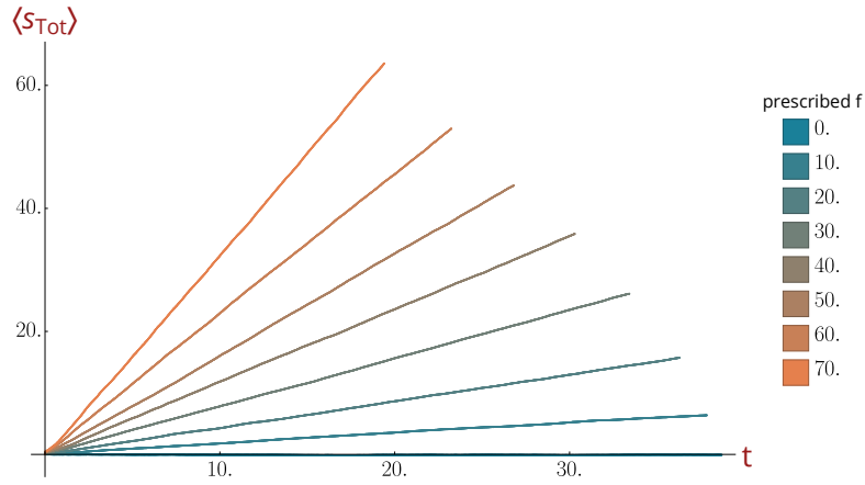
Figure 6.9: Aggregate fibre displacement \langle s_{tot} \rangle averaged over 10 trajectories versus time for different prescribed load f . All displacement are drawn for the same number of iterations.
