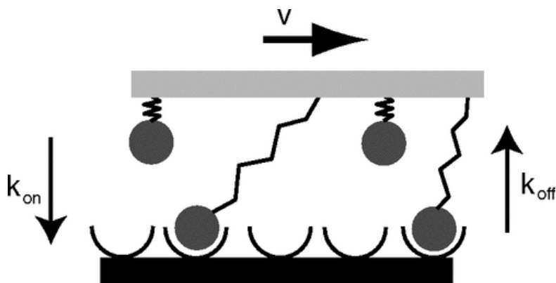
Figure 2.6: Model for an adhesive cluster that bridges two surfaces in motion relative to each other. From Safran and Schwarz [69].
