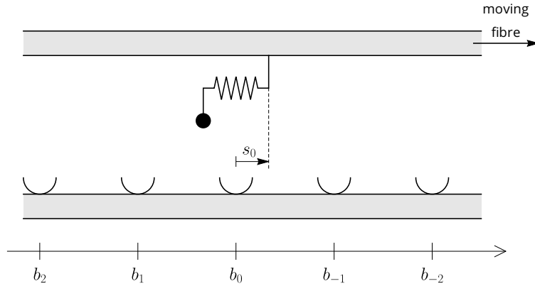
Figure 3.12: Binding sites are numbered relative to the binding site closest to the anchor point of the bond ( i = 0 ). The site number is positive opposite the direction of fibre movement and negative in this direction.
