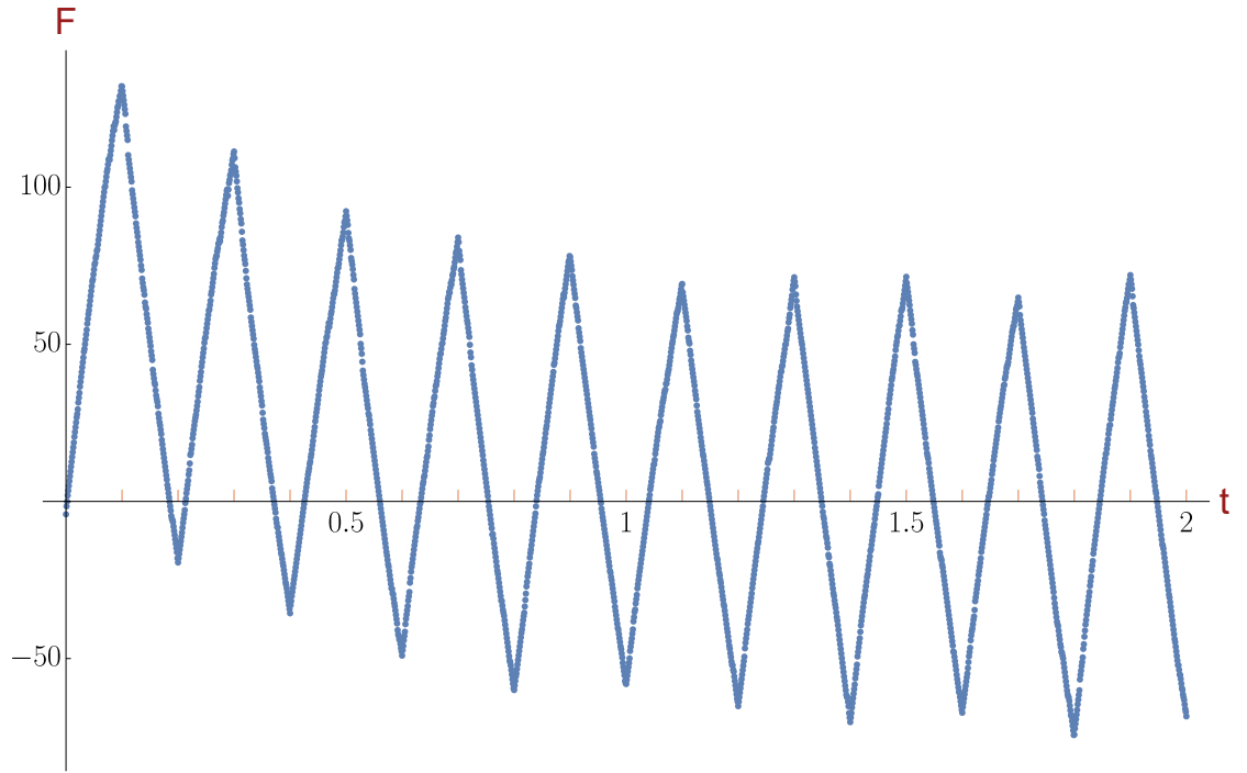
Figure 5.20: Sample trajectory of a cyclic solicitation. Orange ticks indicate the position in time where a reversal of the traction velocity occurs.
