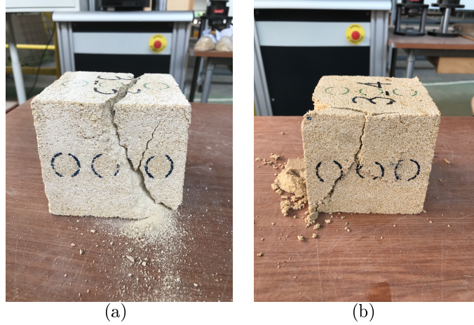
Figure 2.9: Failure mode of dry and saturated sireuil sample
