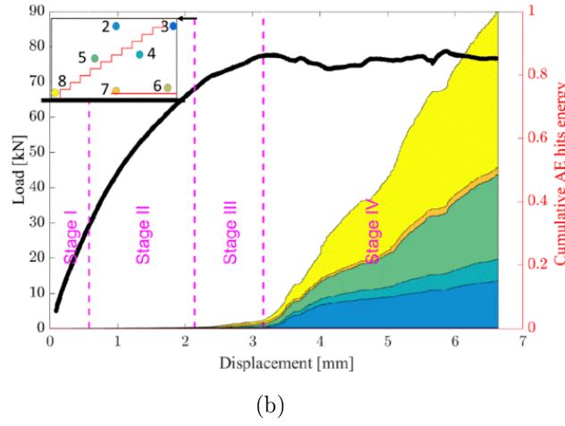
Figure 4.16: Cumulative hit number / energy by each sensor vs. displacement in shear wall test
