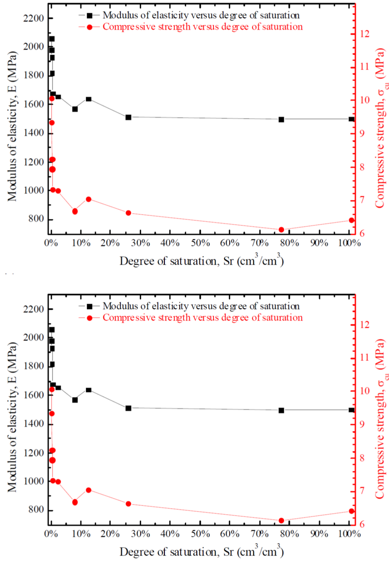
Figure 1.8: Compressive strength/modulus of elasticity vs. degree of saturation for (a) ‘White Tuffeau’ and (b) ‘Sébastopol’ stone[Beck et al., 2007]
