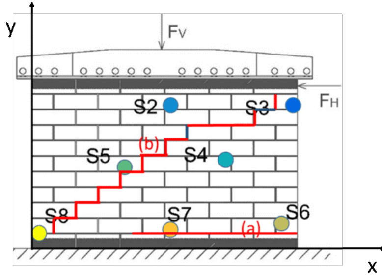
Figure 4.11: Illustration of shear wall test setup and sensor position,
