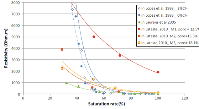
Figure 1.34: Saturation rate versus electrical resistivity[Lataste and Göller, 2018]
