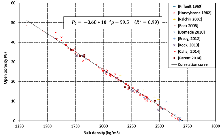
Figure 1.5: Open porosity vs. bulk density [Parent et al., 2015]
