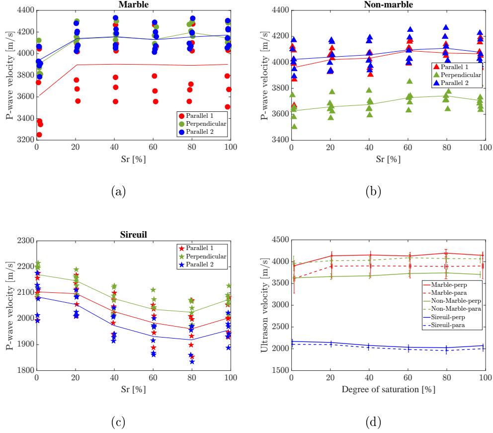
Figure 2.26: Evolution of p wave velocity in (a) marble (b) non-marble (c) sireuil (d) summarised results
