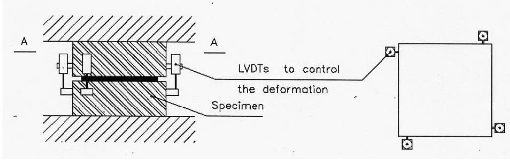
Figure 1.12: Preferred location of LVDTs for direct tensile tests [Lourengo et al., 2005]
