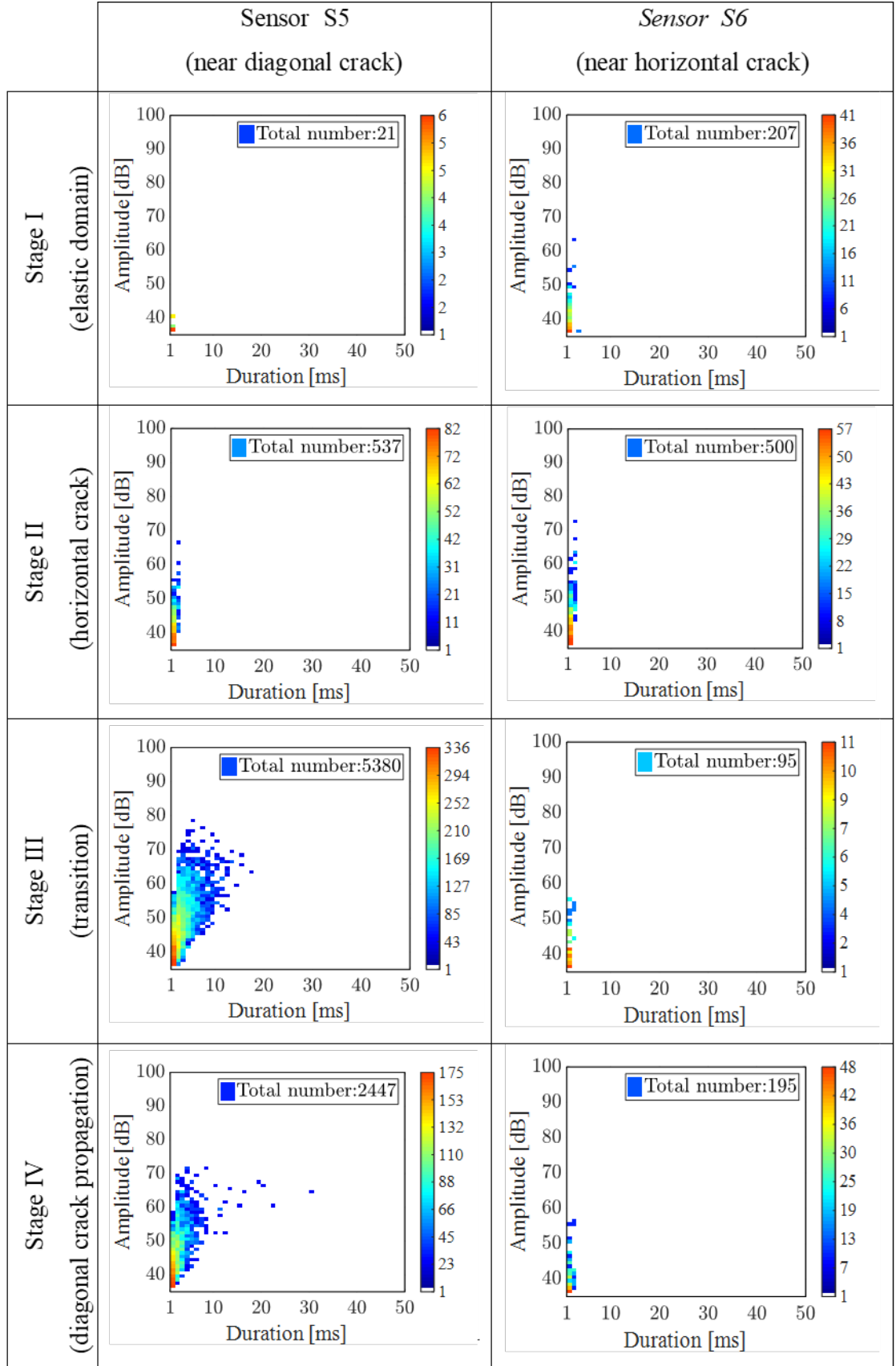
Figure 4.26: Hit intensity map of amplitude vs. duration by sensor 5 and 6 at the four stages
