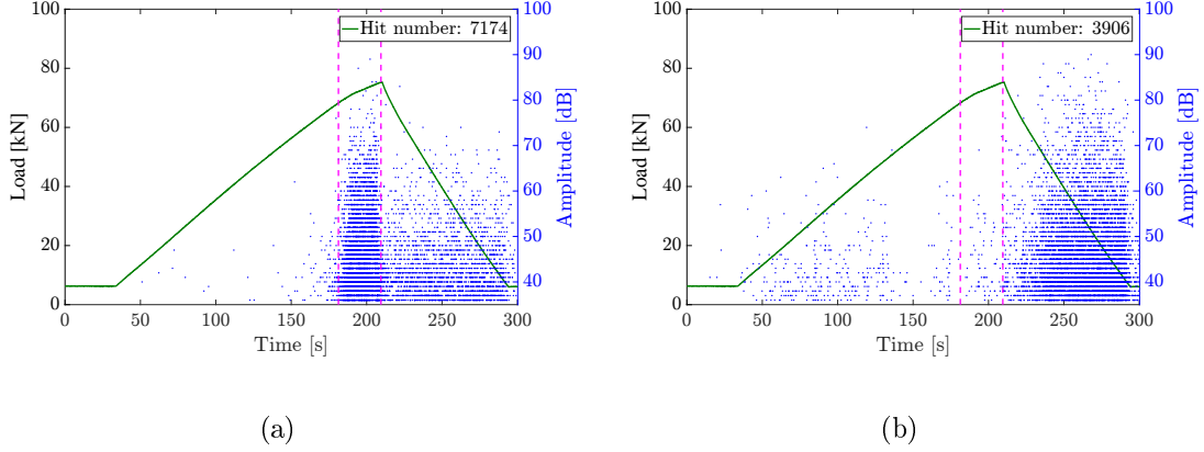
Figure 4.23: Load/amplitude vs. time of sensor 5(left) and sensor 6(right) in stage III
