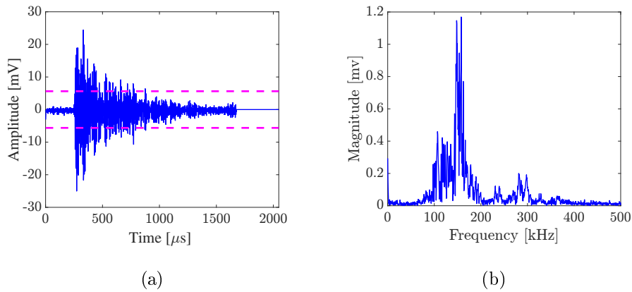
Figure 3.3: A representative signal in the time domain and frequency domain
