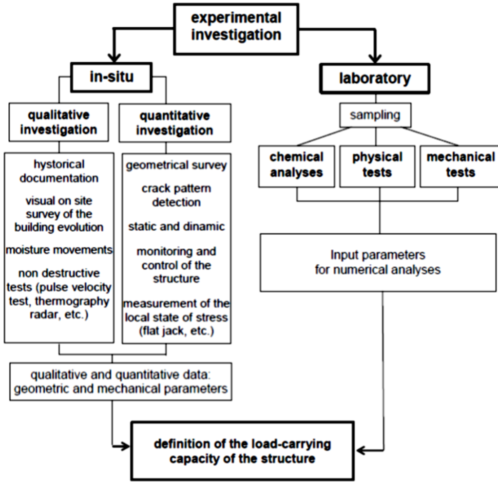
Figure 1.1: Information required and corresponding investigation[Binda et al., 1994]
