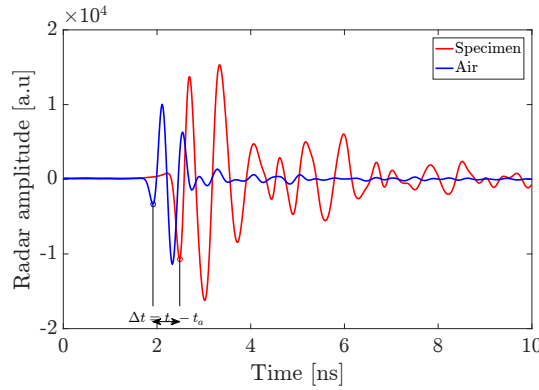
Figure 2.13: Waveform of radar signal through specimen and air
