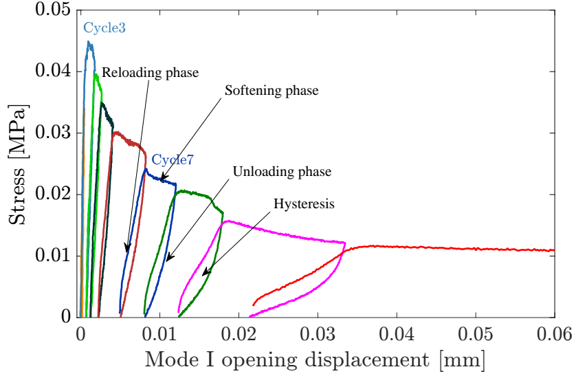
Figure 3.6: Mode I stress vs. displacement curves in cyclic test on TC2 sample.
