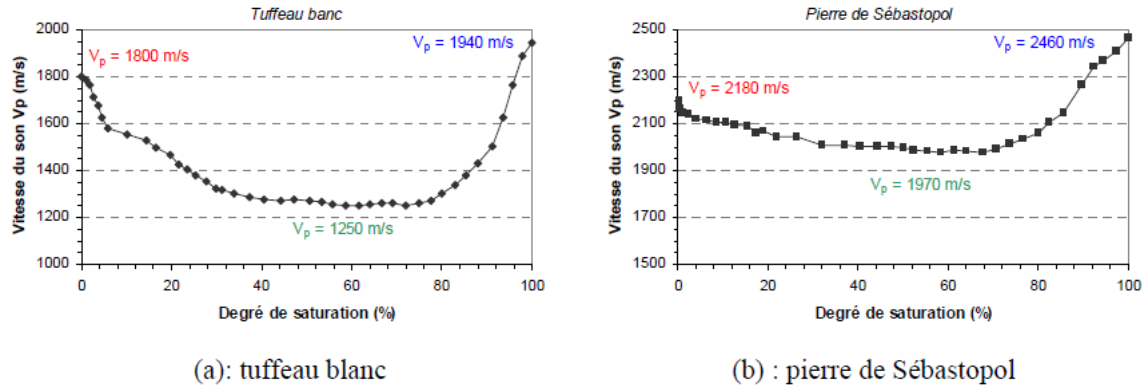
Figure 1.25: Evolution of ultrasound velocity (P-wave) following the degree of saturation pour White Tuffeau / 'Sébastienopol' stone (perpendicular to bedding)[Beck, 2006]
