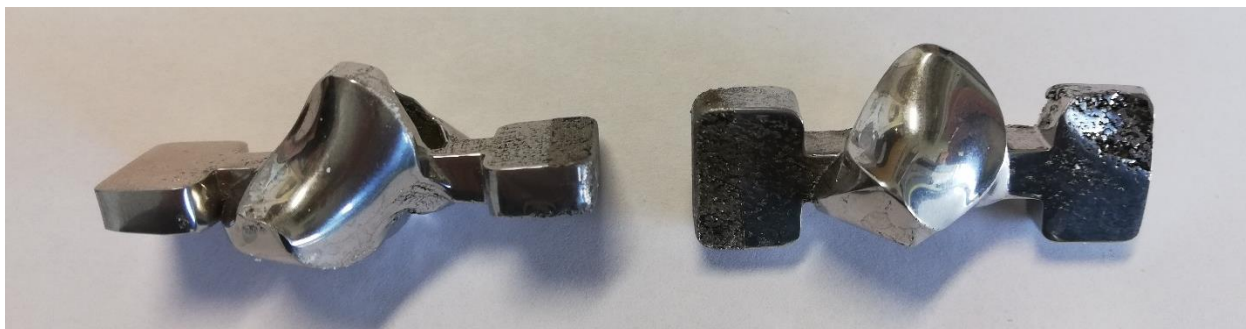
Figure 5: Mirror-like implant processed by SLM and superfinished
