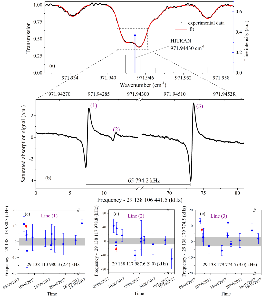
Figure 4.31 – (a) Direct absorption spectrum of methanol from 971.93 to 971.96 \text{cm}^{-1} (part of the spectrum in Figure 4.14. It is recorded at a pressure of \sim 7 Pa using the free-running QCL. The red curve is a fit to the data. The ^P P(E, ri, 0, -5, 32) line frequency position reported in the HITRAN database [54] is also shown as a blue stick. (b) Saturated absorption spectrum showing three methanol transitions (1, 2, and 3) around 971.944 \text{cm}^{-1} recorded using frequency modulation and first-harmonic detection. Experimental conditions: pressure, 1 Pa; modulation frequency, 20 kHz; frequency modulation excursion, 50 kHz; frequency step, \sim 15 kHz; average of 5 pairs of scans of opposite frequency sweep direction; total integration time per point, 1 s; whole spectrum measurement time, 2002 s. (c-e) Frequency measurements of the three rovibrational methanol lines (1), (2), and (3). Eleven measurements were carried out (ten measurements in June and one in October 2017). The transition frequency resulting from the weighted mean of data of June is indicated with the associated 1- \sigma weighted standard error and symbolized by the grey rectangular. The red arrow in each graph pinpoints the measurement corresponding to panel (b) of the figure.
