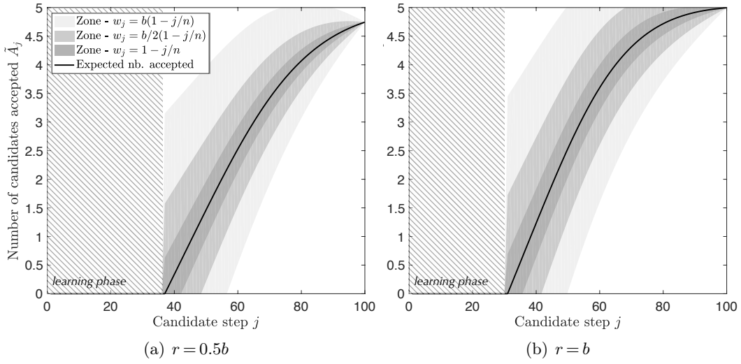
FIGURE 4.4: Expectation of the number of candidates accepted so far for n=100 candidates given that no candidate was accepted by default (black line). Number of jobs is b=5 and the reference set quality is q=0.5 . The zone (see Definition 9) is gray-shaded with, from light to dark, w_j = \{b(1 - \frac{j}{n}), \frac{b}{2}(1 - \frac{j}{n}), 1 - \frac{j}{n}\} .
