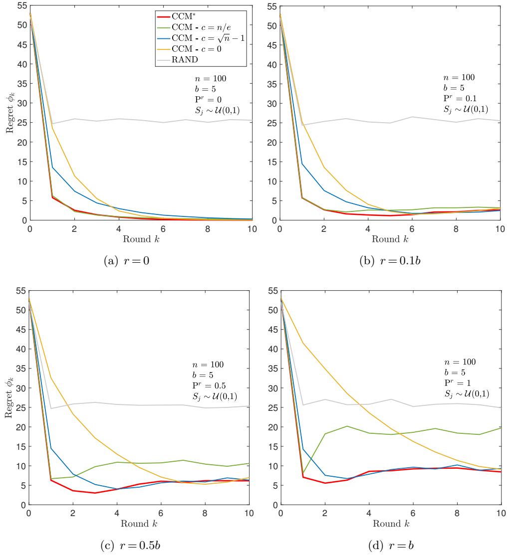
FIGURE 4.5: Average regret \phi_k w.r.t. the round number k , for n=100 candidates, b=5 jobs positions, and the score distribution is S_{i,k} \sim \mathcal{U}(0,1) . Each subfigure corresponds to a different number of resignations r = \{0, 0.1b, 0.5b, b\} .
