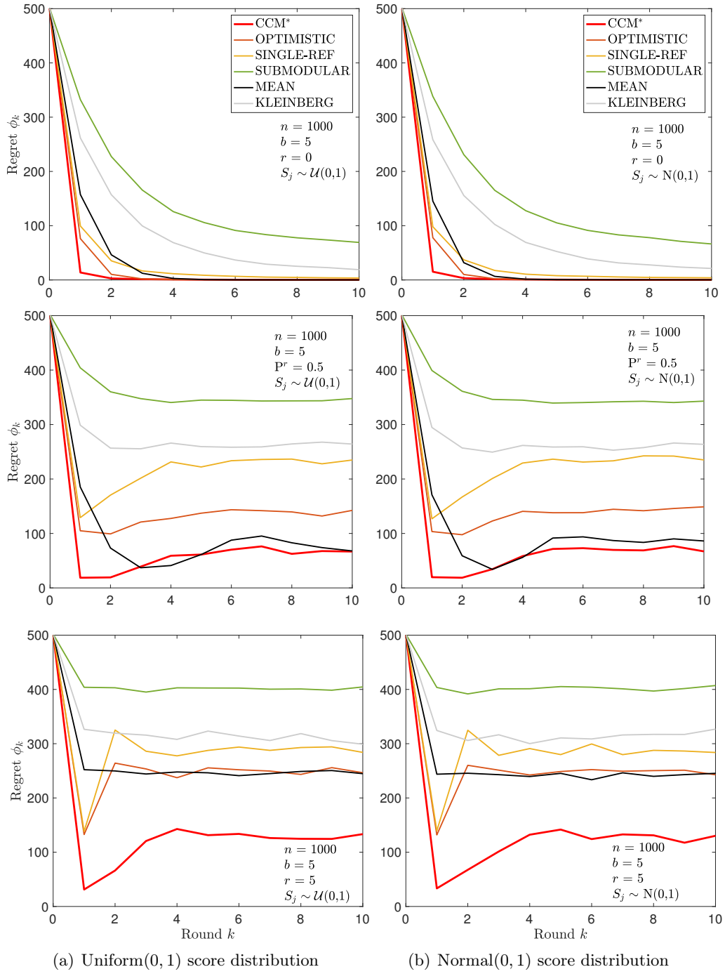
FIGURE 4.9: Average rank-based regret \phi_k w.r.t. the round number k for a budget of b=5 jobs and n=1000 candidates. A different resignation probability is used in each row, namely: P^r=0 ( r=0 )(top row), P^r=0.5 (middle row) and P^r=1 ( r=b=5 ) (bottom row).
