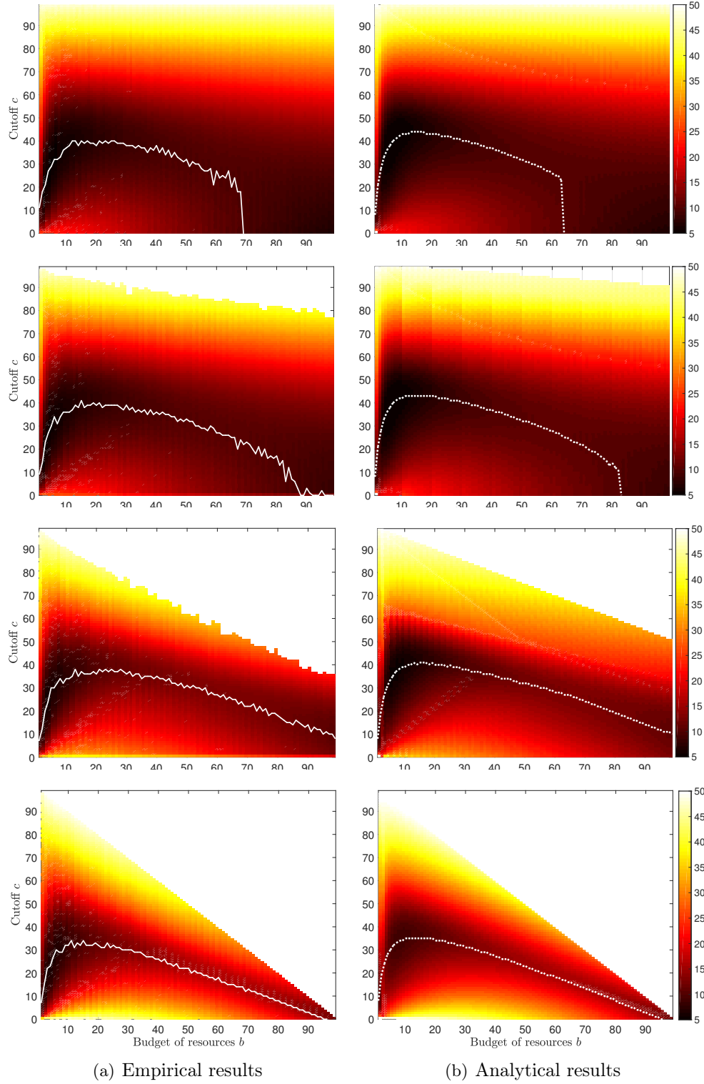
FIGURE 4.2: Comparative heatmaps for the average empirical regret (left column) and the expected regret (right column) derived from Theorem 1 over different resignation numbers r = \{0, 0.1b, 0.5b, b\} from top to bottom line, and all for reference set quality q = 1/2 . In each case, the heatmap of the regret is presented over the parametrization of the cutoff value c and the budget of resources (jobs), b .
