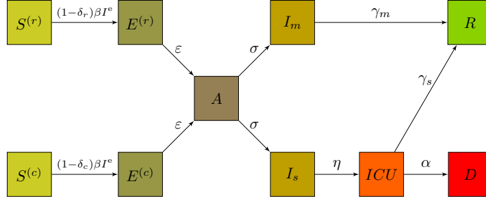
FIGURE A.1: Simplified schematic of the risk-extended SEAIR model, showing rates of passage from the different compartments. Displayed compartments are the released susceptibles, S^{(r)} , the confined susceptibles, S^{(c)} , the released latent, E^{(r)} , the confined latent, E^{(c)} , the asymptomatic, A , the infectious with severe symptoms requiring ICU, I_s , the infectious with milder symptoms, I_m , the people in Intensive Care Unit, ICU , as well as those who died from the disease, D , and those who recovered and are immune, R . All parameters may be found in Table A.2.
