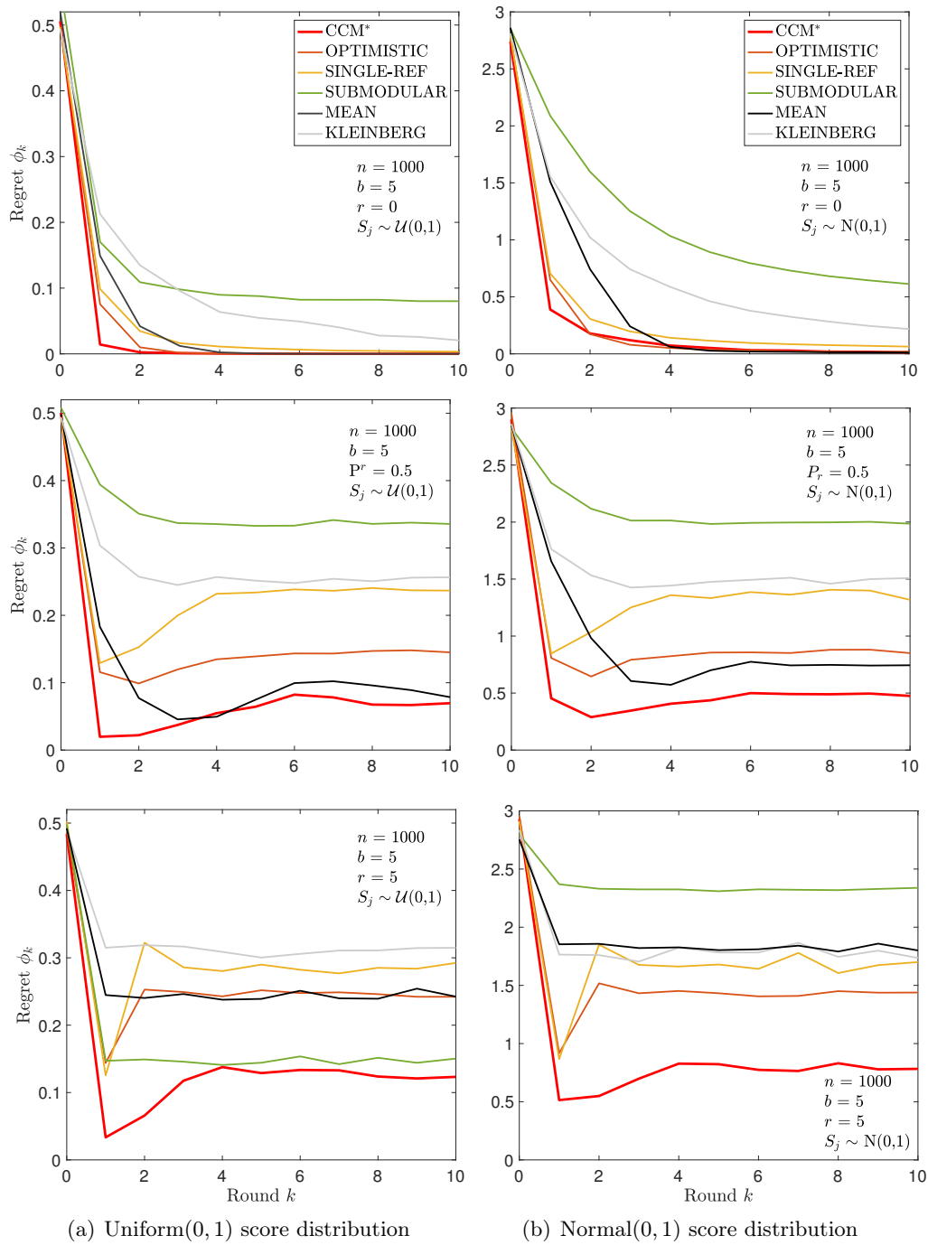
FIGURE 4.10: Average score-based regret \phi_k w.r.t. the round number k for a budget of b=5 jobs and n=1000 candidates. A different resignation probability is used in each row, namely: P^r=0 ( r=0 )(top row), P^r=0.5 (middle row) and P^r=1 ( r=b=5 ) (bottom row).
