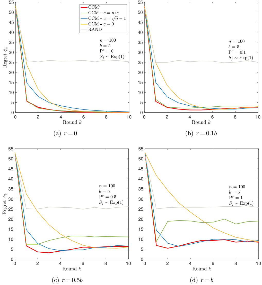
FIGURE 4.7: Average regret \phi_k w.r.t. the round number k , for n=100 candidates, b=5 jobs positions, and the score distribution is S_{i,k} \sim \text{Exp}(1) . Each subfigure corresponds to a different number of resignations r = \{0, 0.1b, 0.5b, b\} .
