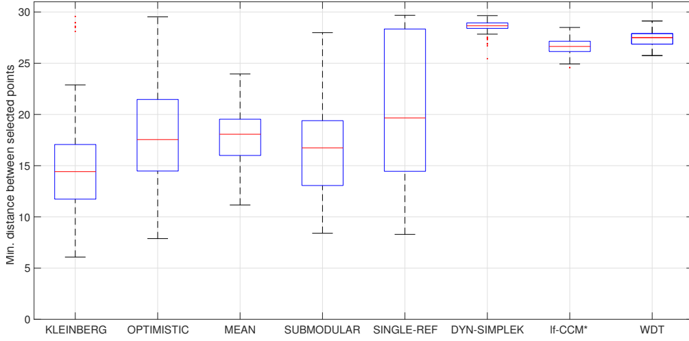
FIGURE 7.2: Minimum distance between the b=10 selected instances on generated random walks. The red line gives each strategy’s median, blue boxes are the quantiles and the outliers are represented with red dots. The lf-CCM* and the WDT algorithms operate in b rounds.
