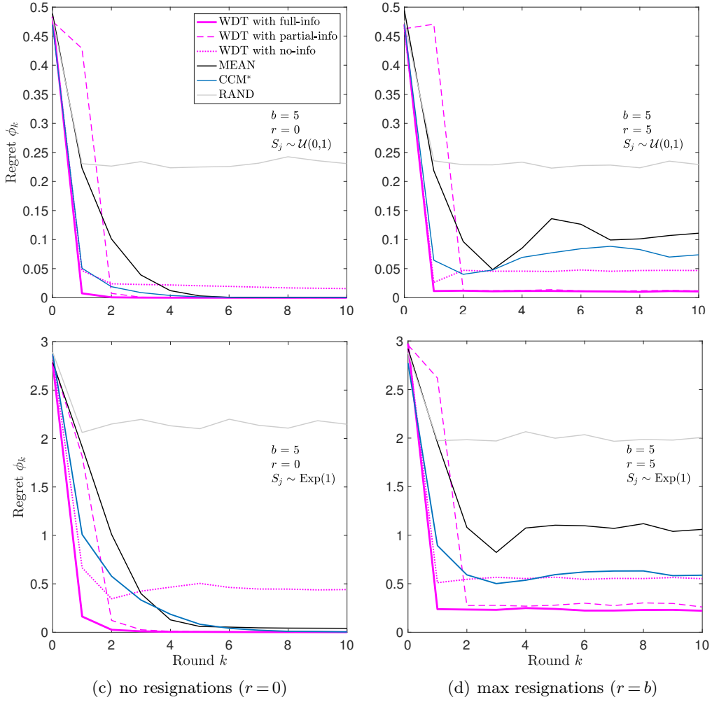
FIGURE 5.2: Average regret \phi_k versus the round number k . The number of job positions is b=5 for n=100 candidates per round. Score distribution: uniform, S_{i,k} \sim \mathcal{U}(0,1) (top row); exponential, S_{i,k} \sim \text{Exp}(1), \forall i, \forall k (bottom row). The number of initially empty job positions is r=0 (left) and r=b=5 (right). Magenta lines use WDT in full-information (plain line), partial-information (dashed line) and no-information (dotted line) settings.
