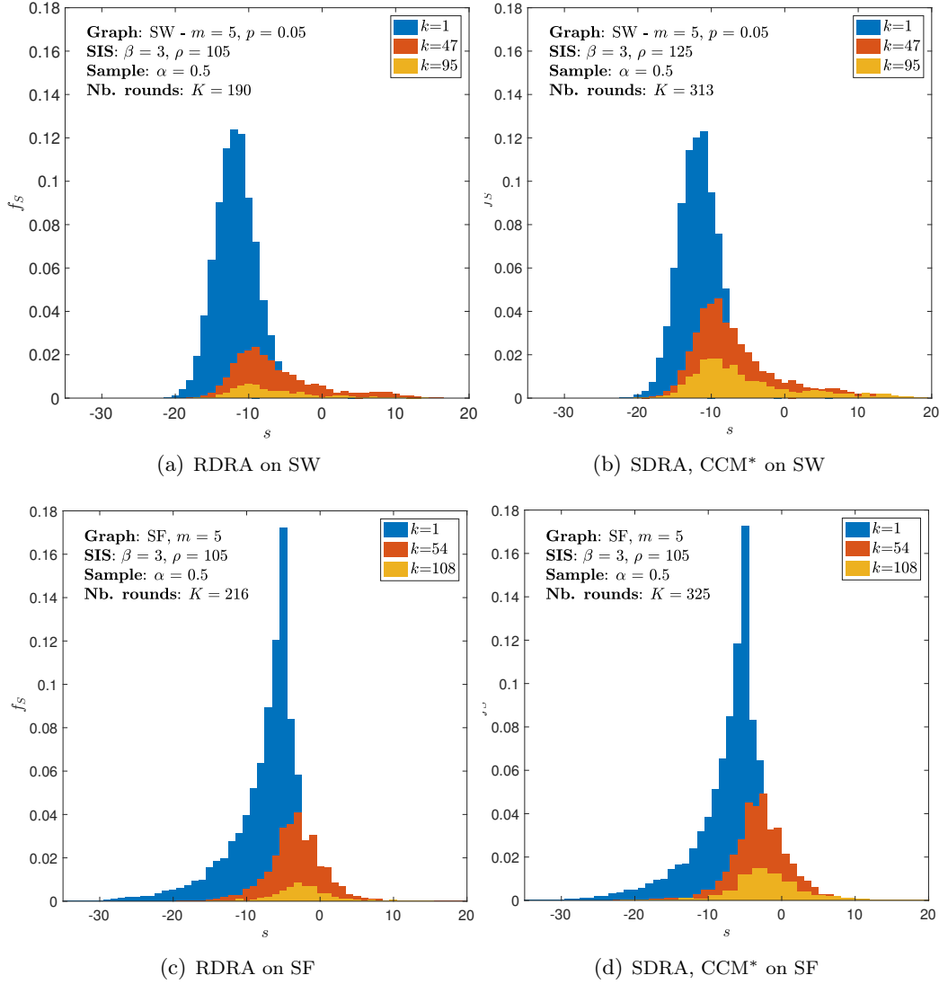
FIGURE 6.6: The empirical p.d.f. f_s of the node scores, at different different rounds k through the multi-round process, for SW (top row) and for SF (bottom row) networks. The results refer to the application of RDRA or SDRA (the CCM*) strategies with the LRIE scoring function (initialization with the same infection level in each row).
