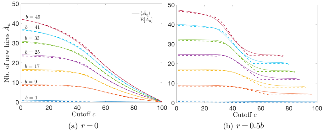
FIGURE 4.11: Dotted lines show display the analytical number of new hires \mathbb{E}[\tilde{A}_n] given in Eq. 4.5, while plain lines are the respective empirical \tilde{A}_n , i.e. the average number of accepted candidates in the simulations. Different colors depict scenarios with number of jobs being, from bottom to top line, b = \{1, 9, 17, 25, 33, 41, 49\} .
