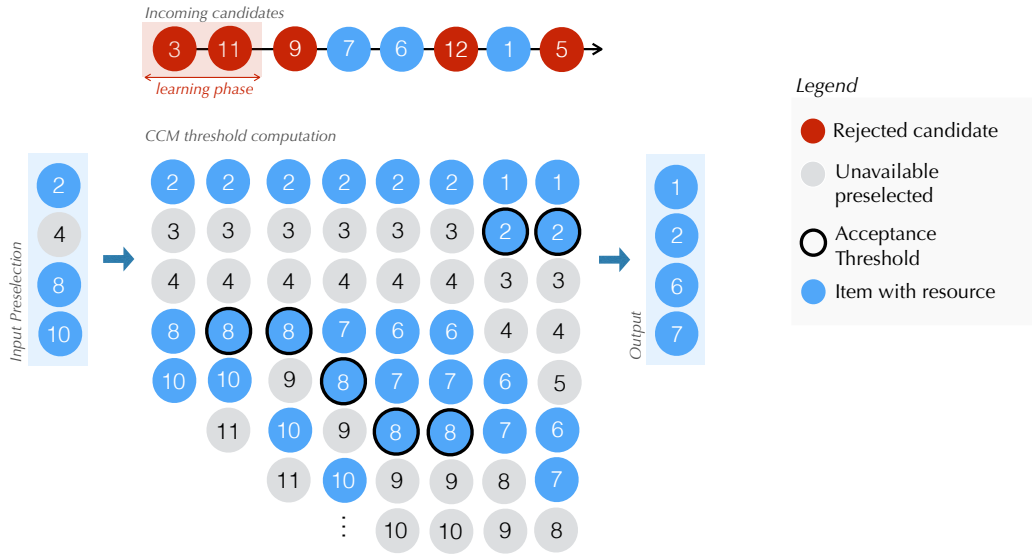
FIGURE 4.1: A step-by-step deployment of the CCM policy for the WSSP. The indicated candidate ranks refer to the true ranking of all twelve items, referents and candidates. The top line gives the sequence of incoming candidates. The scheme reads from left ( j=0 ) to right ( j=n=8 ), i.e. each column lists the items seen so far order by absolute ranks (rank 1 being the best).
