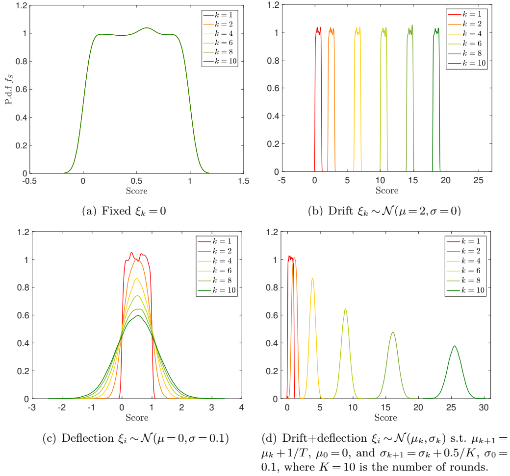
FIGURE 3.3: Example of evolution of the score distribution at different rounds represented by different colors k = \{1, 2, 4, 6, 8, 10\}
