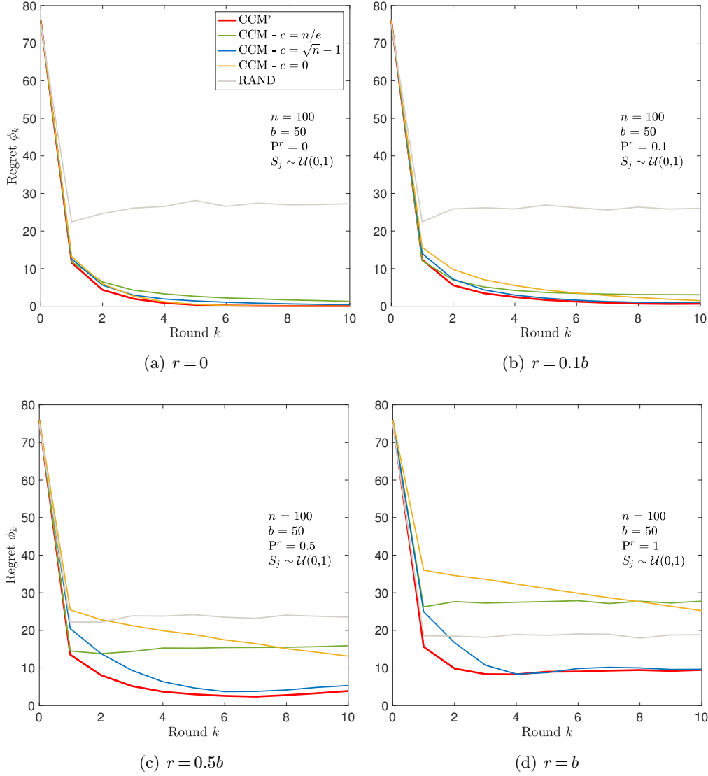
FIGURE 4.6: Average regret \phi_k w.r.t. the round number k , for n=100 candidates, b=50 jobs positions, and the score distribution is S_{i,k} \sim \mathcal{U}(0,1) . Each subfigure corresponds to a different number of resignations r = \{0, 0.1b, 0.5b, b\} .
