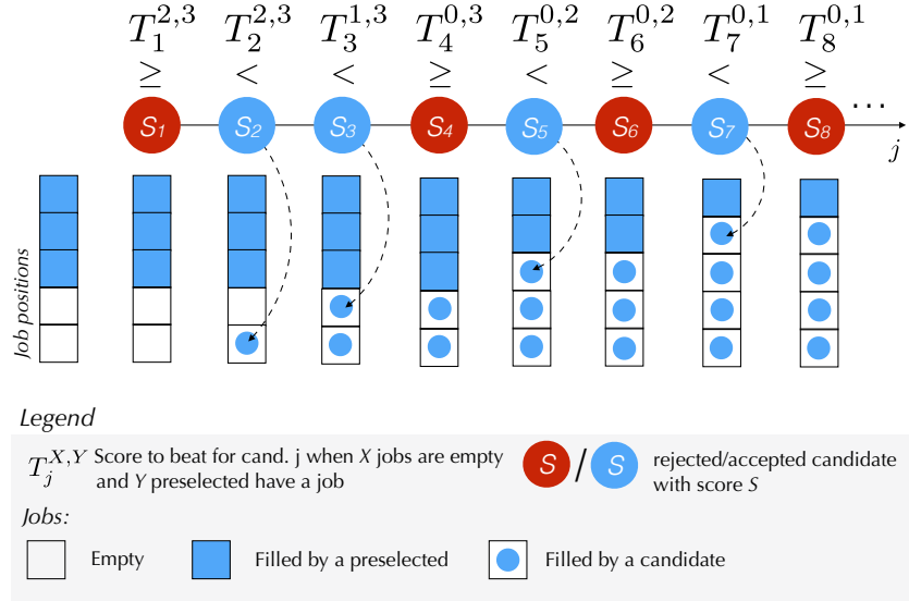
FIGURE 5.1: Demonstration of the WDT algorithm. The score of an incoming candidate, S_j , is compared to an associated acceptance threshold T_j^{X,Y} , where X and Y are respectively the current number of empty positions and that of positions occupied by preselected employees. Accepted candidates (blue circle) first fill empty positions and then, if they are competitive enough, take a preselected employee's positions (e.g. the 5-th candidate).
