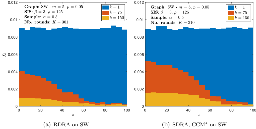
FIGURE 6.10: The empirical p.d.f. f_s of the node scores, at different different rounds k through the multi-round process, for a SW network. The results refer to the application of RDRA or SDRA (the CCM*) strategies with the MCM scoring function (initialization with the same infection level)).
