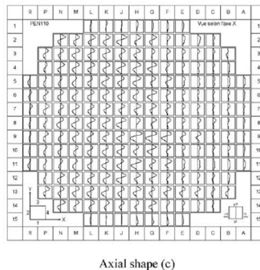
Figure 5-2 - Public domain information about fuel assembly bowing and axial deformation [3]
