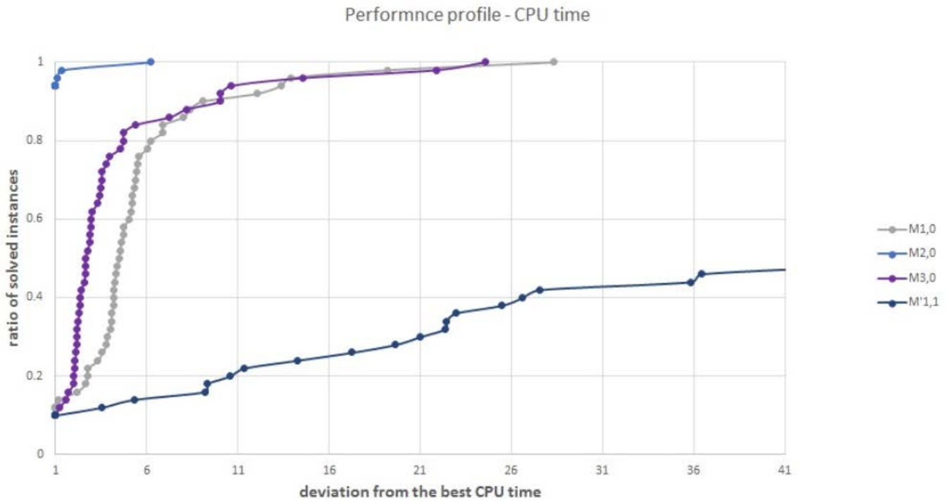
FIGURE 4.6 – Performance profile-CPU times : integrality requirement imposed on variables z_{m,i,n,j}
