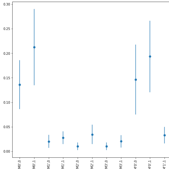
FIGURE 4.1 – 95% confidence interval plot of the optimality gap-integrality requirement on variables z_{m,i,n,j} relaxed
