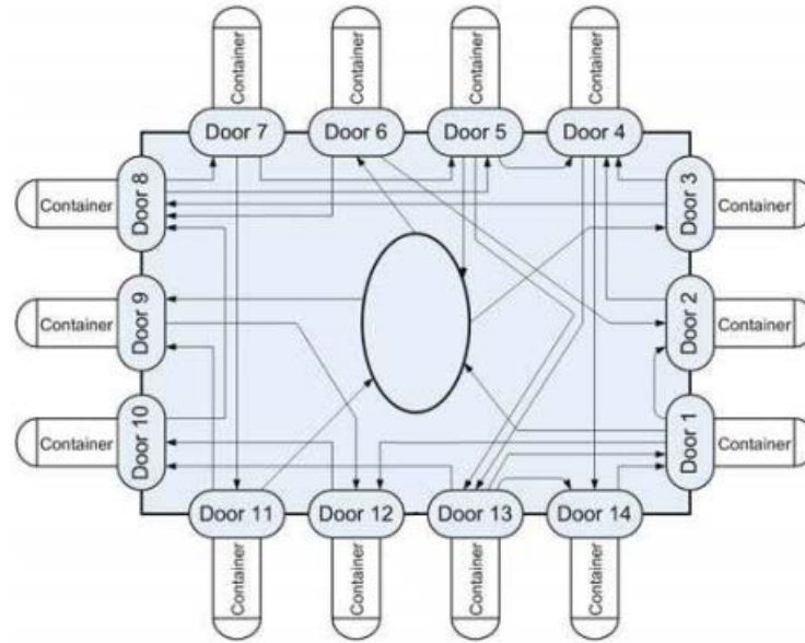
FIGURE 3.6 – Mixed mode of door service, Shakeri et al. (2008)
