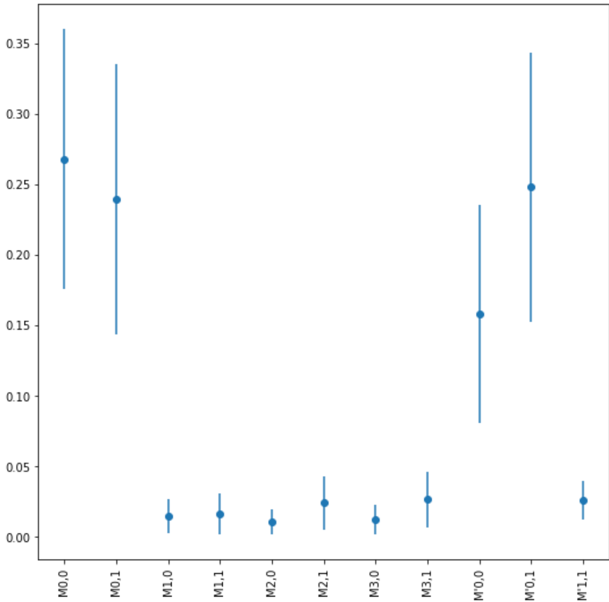
FIGURE 4.4 – 95% confidence interval plot of the optimality gap-integrality requirement on variables z_{m,i,n,j} imposed
