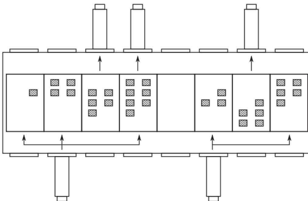
FIGURE 3.8 – Single-stage or two-touch cross-dock , Gue and Kang (2001)
