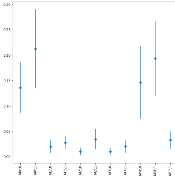
FIGURE 4.1 – 95% confidence interval plot of the optimality gap-integrity requirement on variables z_{m,i,n,j} relaxed
