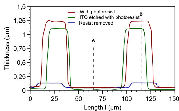
Figure. 4.5 Profilometry of the electrode substrate at different stages of microfabrication
