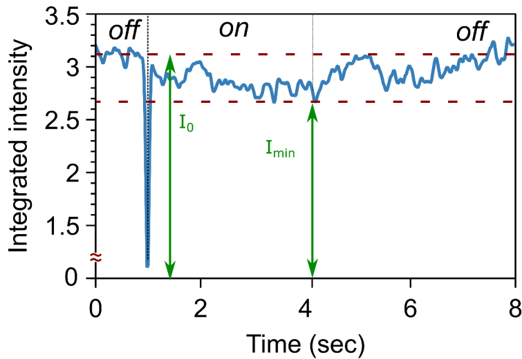
Figure. 5.13 Integrated intensity as a function of time in the monitored area of dielectrophoretic capture of 200 nm latex nanospheres applying an electric field amplitude of 7 V pp and a frequency of 6 MHz using fluorescence videomicroscopy (50 fps). The signal was averaged 25 "ON-OFF" cycles.
