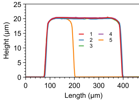
Figure. 4.8 Thickness of SU-8 deposited by spin coating on silicon wafers. 1 to 4: Profilometric scans of four different molds with a 300 \mu\text{m} width channel. 5: microchannel of 100 \mu\text{m} of width.
