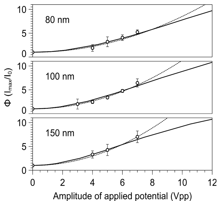
Figure. 5.20 Experimental DEP capture ratios (black circles) for gold nanoparticles in aqueous solution as a function of the amplitude of the AC potential applied to the electrodes, quadratic models fits to the experimental data (dotted lines) and capture ratios from numerical modelling realised in sections 5.5.5 (solid lines) and 5.5.6. Each experimental point corresponds to at least three measurements in different devices ( f = 1 \text{ MHz} ).
