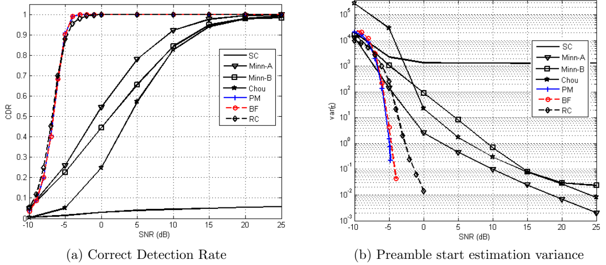
Figure 4.5: Preamble start estimation performance in the monopath AWGN channel.
