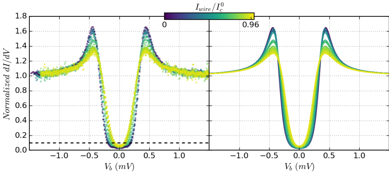
Figure 5.3: DOS as a function of the supercurrent flow. Left panel: Normalized differential conductance as a function of bias voltage of sample N03 for different wire currents I_{wire} at 100 mK. Dashed horizontal line: threshold used to extract \Delta_C plotted in Fig. 5.4b. Right panel: Theoretical fits: the I_{wire} = 0 spectrum (for which \gamma is set to 0) leads to \Gamma_{in} = 0.02\Delta_0 and k_B T_{eff}/\Delta_0 = 0.13 . \Gamma_{in} and T_{eff} are then fixed to fit all the spectra with \gamma and \Delta as free parameters. I_c^0 is the zero temperature critical current in the absence of any perturbation due to the STM tip.
