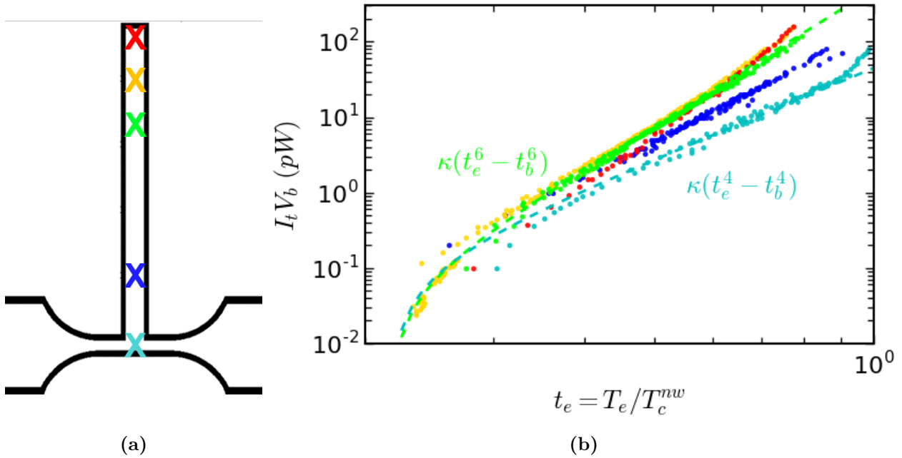
Figure 6.13: Effective electronic temperature as a function of power for different injection positions. (a) Schematics of the sample with indicated injection positions. (b) I_t V_b as a function of the reduced electronic temperature. Dashed lines indicate the I_t V_b = \kappa(t_e^m - t_b^m) curves with m = 4 and m = 6 for respectively \kappa = 118 pW.K -4 and \kappa = 2137 pW.K -6 . Sample N13.
