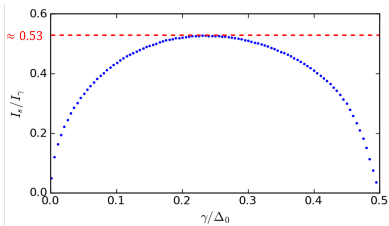
Figure 2.3: Supercurrent versus depairing energy at T = 0 .
