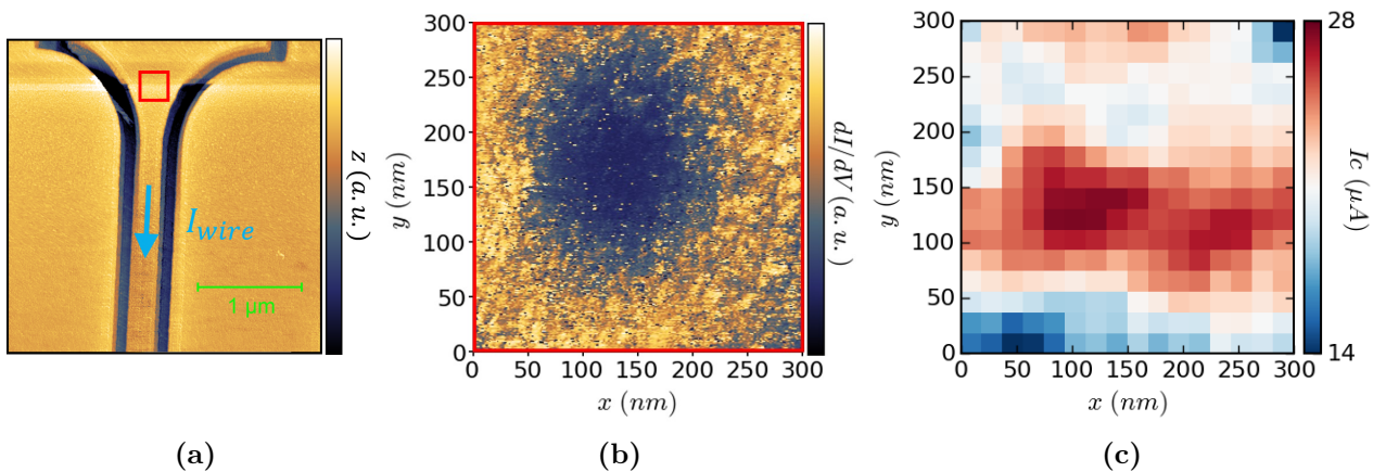
Figure 7.4: Tunneling injection of high energy quasiparticles in the vicinity of a vortex. (a) STM topographic image of the nanowire with in red inset the area of the SCCM measurement. The blue arrow indicates the direction of the current. (b) Spectroscopic image at I_t = 1 nA and V_b = 400 \mu V recorded during the SCCM measurement. (c) Critical current as a function of injection position for a constant tunneling setpoint I_t^{I_c} = 1 nA and V_b^{I_c} = 400 mV. B = 23 mT, T = 100 mK and \Delta_0 = 380 \mu eV. Sample N04.
