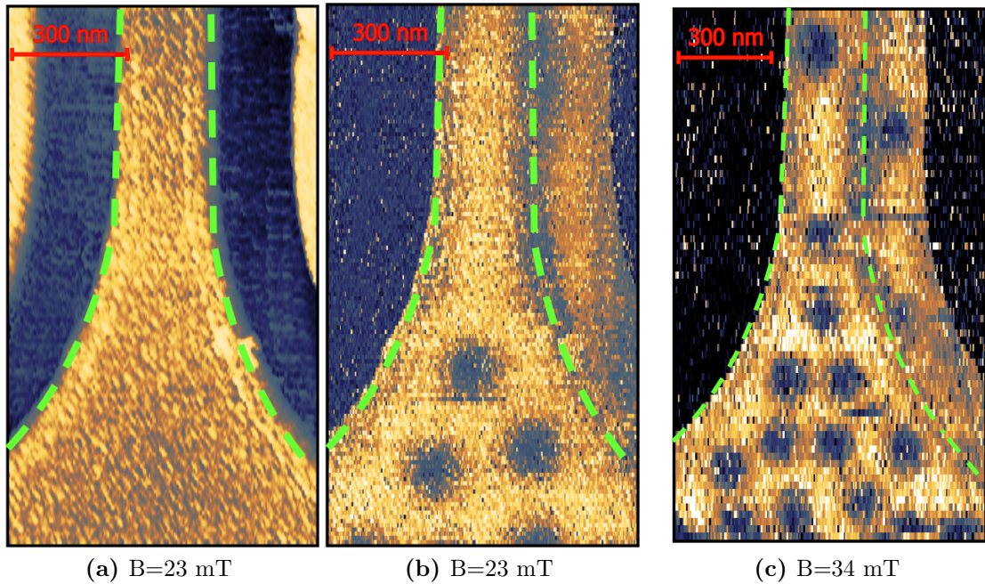
Figure 7.1: Penetration of vortices in a nanowire. (a) and (b) Topographic and spectroscopic images ( I_t = 500 pA ; V_b = 400 \mu V) of the same area for a perpendicular magnetic field B = 23 mT. The color scale is in arbitrary units with light - respectively dark - colors corresponding to large - respectively small - values of tip height and differential conductance. Green dashed line indicates the (geometric) edges of the nanowire. (c) Spectroscopic image of the same sample for a larger magnetic field B = 34 mT. Sample N04.
